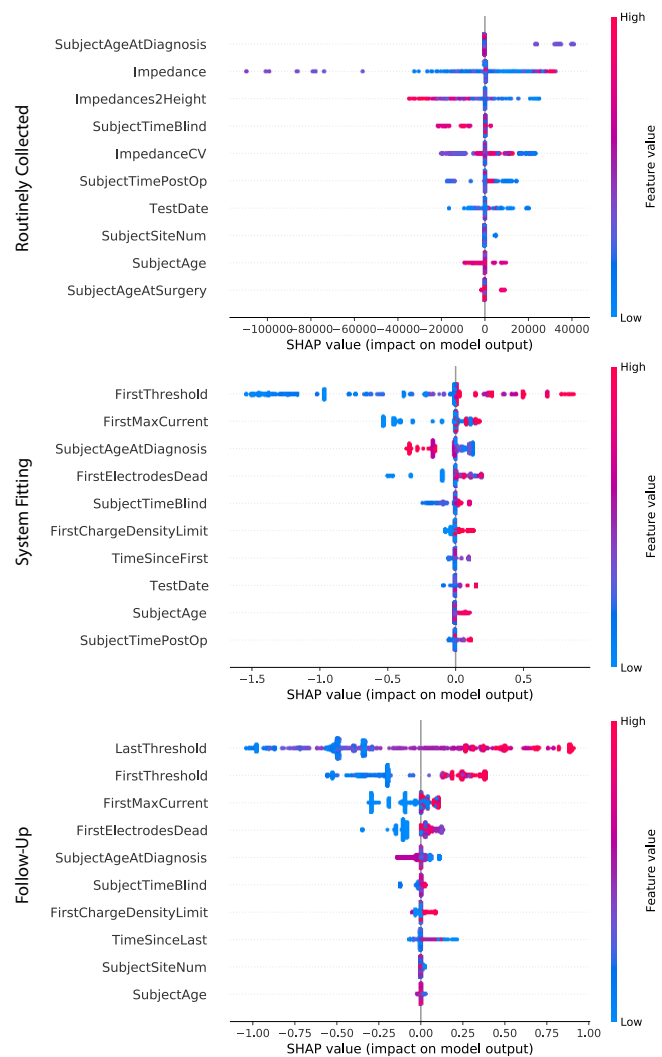
Fig. 2. Force plot of SHapley Additive ex-Planations (SHAP) values for the ten most important features in the dataset (sorted top to bottom). Each data point is a prediction of electrode deactivation from the held-out cross-validation fold (test set). SHAP values indicate each feature’s contribution to the model’s decision (positive: pushing the model towards predicting deactivation; negative: pushing the model away from predicting deactivation). Colors indicate feature values. Results are shown for three different feature splits of the data (see Table II) including routinely collected measures, data from system fitting, and data from follow-up examinations.
