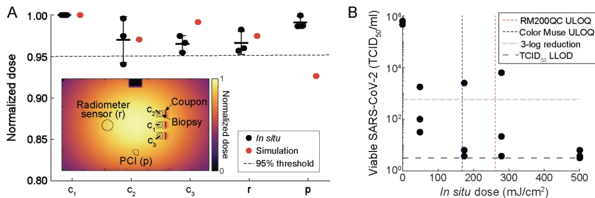
Figure 2. Measurement of UV-C dose required for SARS-CoV-2 inactivation on N95 coupons is informed by optical modeling and in-situ PCI dose measurements. (A) Using the optical model and validating in situ , five locations within the decontamination chamber were identified as receiving similar UV-C doses (<5% variation between mean in-situ dose measurements at each location). To inform biopsy location, the optical model also assessed the impact of each coupon seam (modeled as 15 mm wide × 2.5 mm tall × 1 mm thick absorbing rectangular volumes at the right-hand side of each coupon) on UV-C distribution. In situ measurements were made using PCIs to simultaneously measure dose received at the PCI and 3 coupon locations while simultaneously recording irradiance with the radiometer. Mean and standard deviation are indicated for the in-situ measurements. (B) SARS-CoV-2 recovery on N95 coupons is dependent on in-situ UV-C dose, measured using a radiometer. During UV-C exposure, the radiometer, PCI, and triplicate N95 coupons were each placed as shown in (A). A Borofloat attenuator was placed in front of PCIs to measure doses >168 mJ/cm 2 due to the limited PCI ULOQ. N=3 replicates per dose. ULOQ = upper limit of quantification. LLOD = lower limit of detection.
