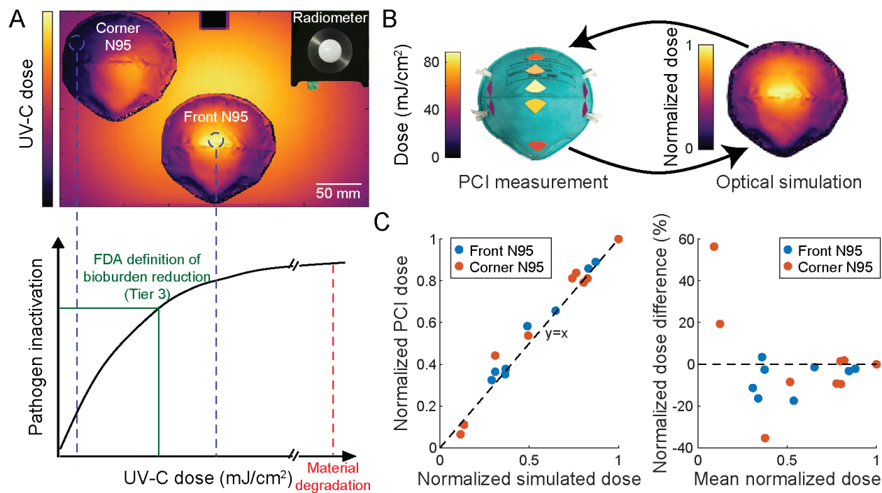
Figure 1. Integrated optical modeling and in-situ PCI measurement pipeline for simultaneous and near-coincident on-N95 UV-C dose and viral inactivation measurements. (A) Schematic highlighting how UV-C dose received across complex N95 surfaces can vary substantially, creating a narrow range of UV-C doses that deliver sufficient dose for pathogen inactivation while not exceeding the exposure threshold for material degradation. (B) In-situ PCI measurements and in silico optical modeling results were used in tandem to inform and rapidly iterate on experimental design. (C) Comparison of normalized in-situ PCI and simulated doses at seven discrete locations on N95s in two different chamber positions. Normalized dose difference was calculated as \frac{\text{simulation}-\text{PCI}}{(\text{simulation}+\text{PCI})/2} . Black lines ( y = x on left, y = 0 on right) indicate where the data would lie if PCI and simulation measurements were equal. Simulation tends to underestimate normalized in-situ PCI dose.
