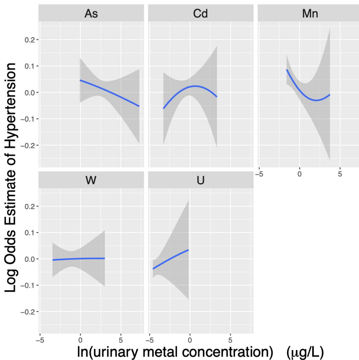
Figure 3C. Exposure-response functions relating urinary metal concentrations to the log hazard estimate (interpreted as a log odds estimate) of prevalent hypertension. Model adjusted for ethnicity (Hispanic/non-Hispanic), income, smoking (never/former/current), and diet.
