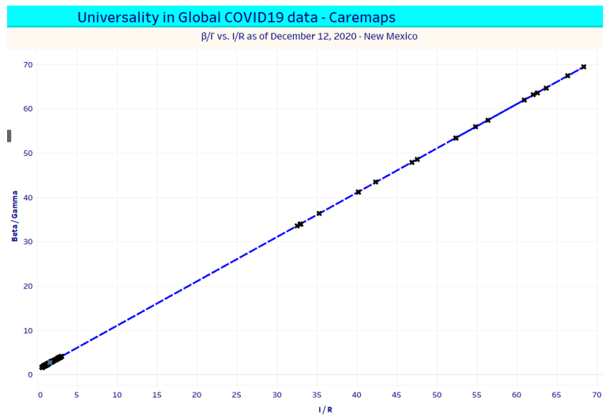
Fig. 2 Universal rule for New Mexico
