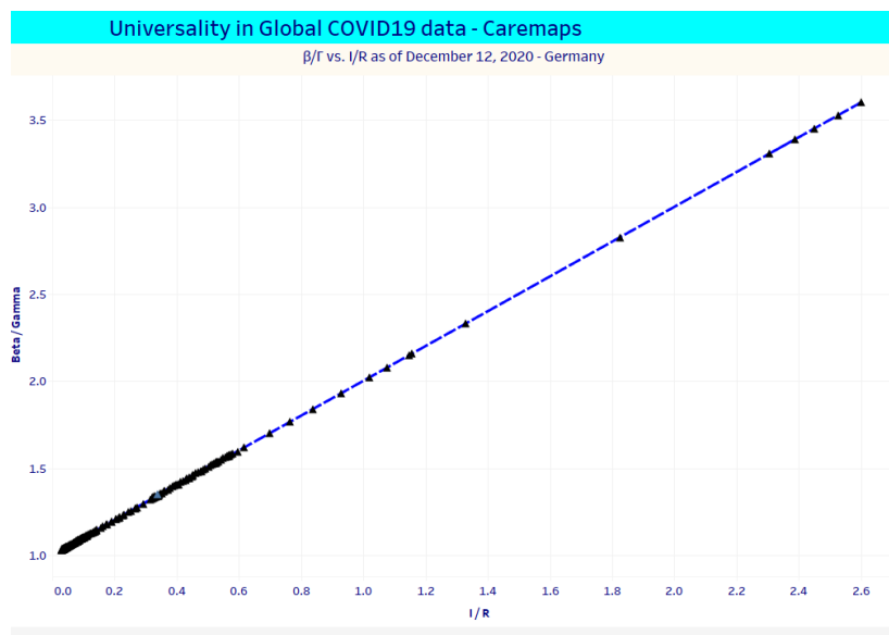
Fig. 3 Universal rule for Germany
