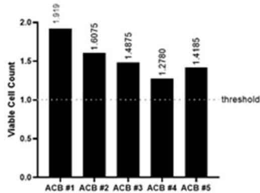
ACB-IP 1.0 Plasma Neutralizing Antibody Activity
