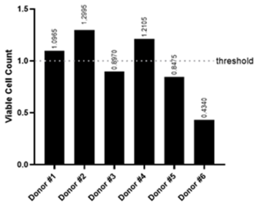
Single Donor Plasma Neutralizing Antibody Activity
