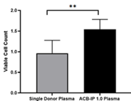
Mean Plasma Neutralizing Antibody Activity
