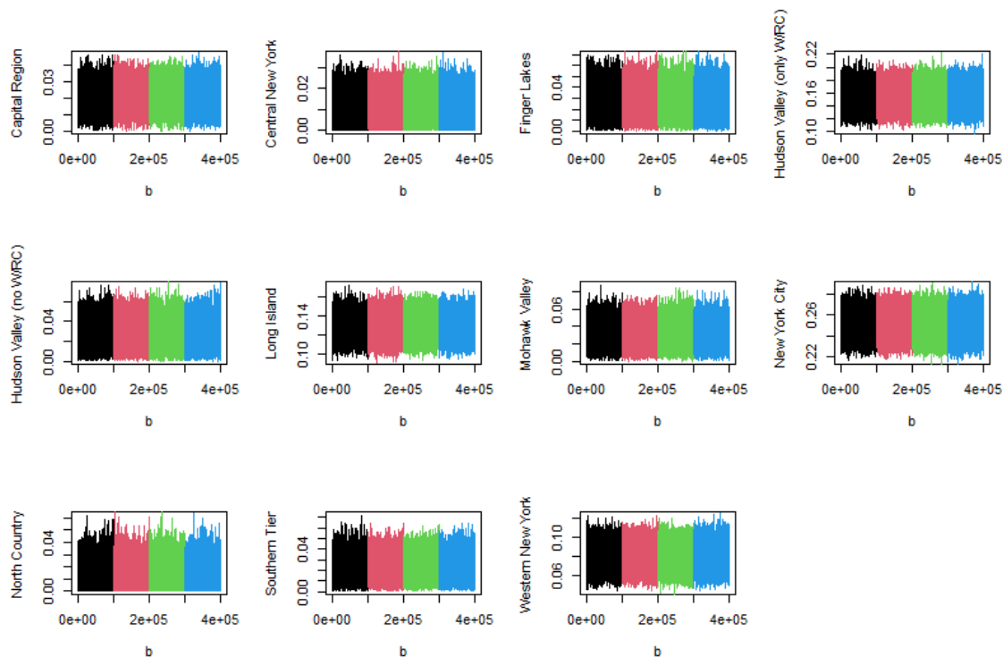
Fig 3. Traceplots of the posterior true prevalence, by region, for the primary model.
