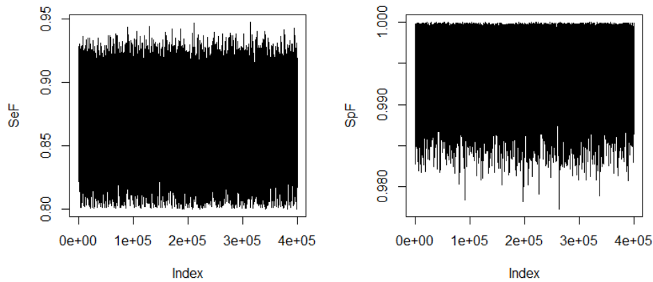
Fig 8. Traceplots of the posterior sensitivity and specificity for the uniform prior prevalence model.
