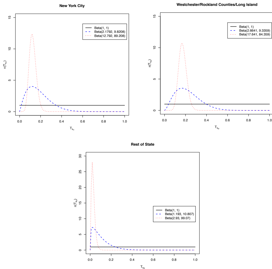
Fig 1. Plots of the prior distributions on true prevalence, T_{s_{ij}} , by super-region. Uniform priors are in solid black, primary model (weakly informative) priors in dashed blue, and informative priors in dotted red. Specific prior details on provided in each plot's legend.
