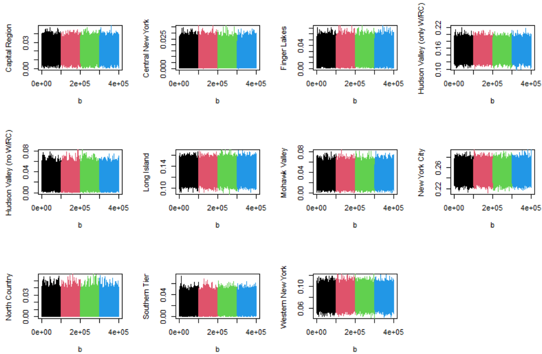
Fig 6. Traceplots of the posterior true prevalence, by region, for the uniform prior prevalence model.
