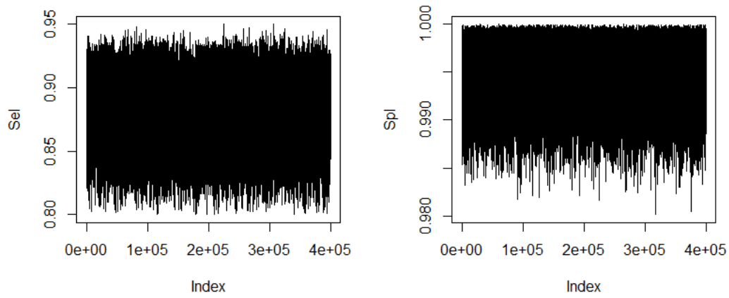
Fig 11. Traceplots of the posterior sensitivity and specificity for the informative prior prevalence model.
