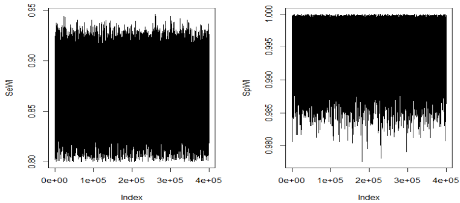
Fig 5. Traceplots of the posterior sensitivity and specificity for the primary model.
