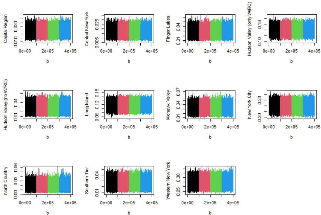
Fig 10. Traceplots of the posterior observed prevalence, by region, for the informative prior prevalence model.
