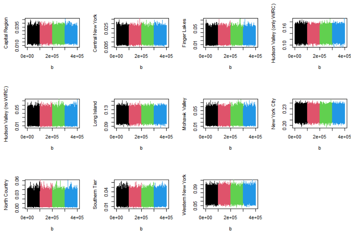
Fig 4. Traceplots of the posterior observed prevalence, by region, for the primary model.
