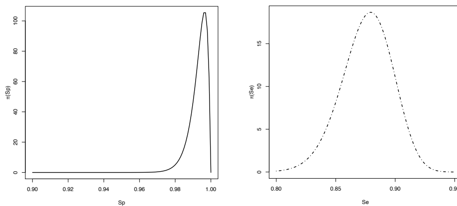
Fig 2. Plots of the prior distributions on specificity, Sp (left panel), and sensitivity Se (right panel). Primary Model (Weakly Informative Prior)
