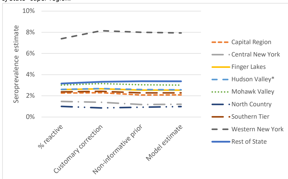
Figure 2. Seroprevalence estimated by the proportion reactive, the customary correction, and the fully Bayesian approach with both weakly informative and non-informative priors for the regions in the “Rest of State” super-region.
