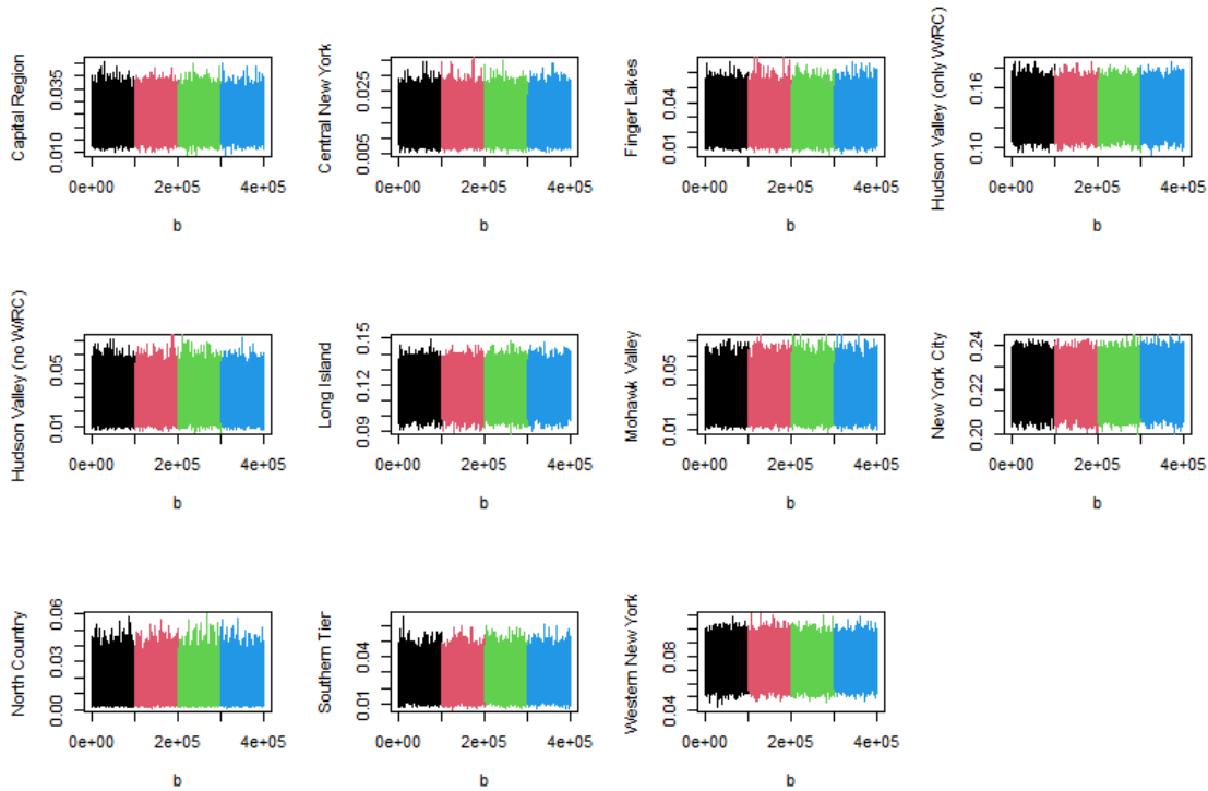
Fig 7. Traceplots of the posterior observed prevalence, by region, for the uniform prior prevalence model.
