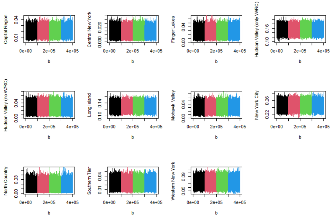
Fig 9. Traceplots of the posterior true prevalence, by region, for the informative prior prevalence model.
