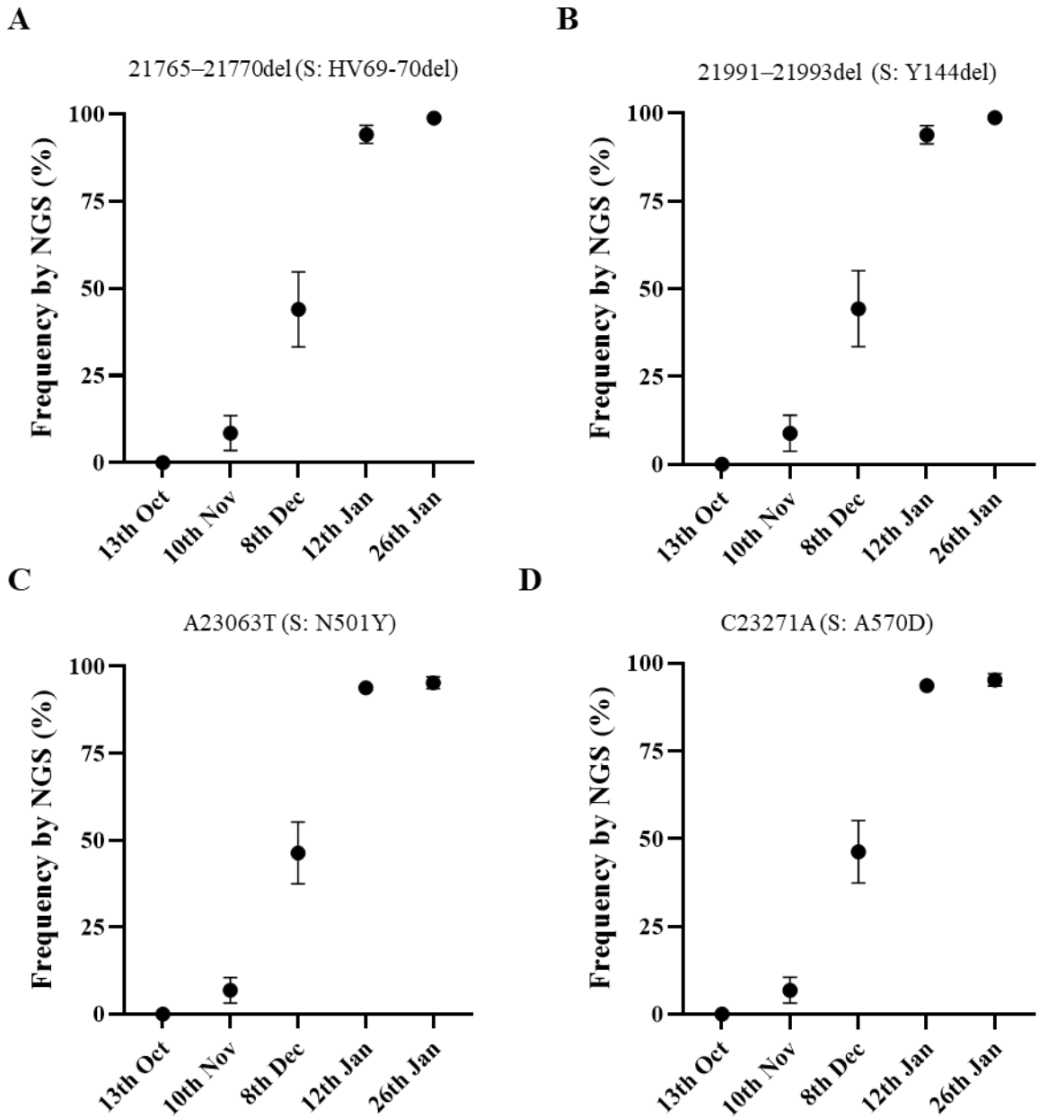
Figure 3. Mean frequency values of nucleotide mutations in the spike gene distinctive of SARS-CoV-2 B.1.1.7 lineage identified in nPCR C and nPCR D products synthesized from sewage concentrates and measured by NGS analysis. A) deletion of nucleotides 21765–21770 (deletion of amino acids HV69-70); B) deletion of nucleotides 21991–21993 (deletion of amino acid Y144); C) mutation A23063T (amino acid change N501Y); and D) mutation C23271A (amino acid change A570D). Error bars indicate standard error of the mean.
