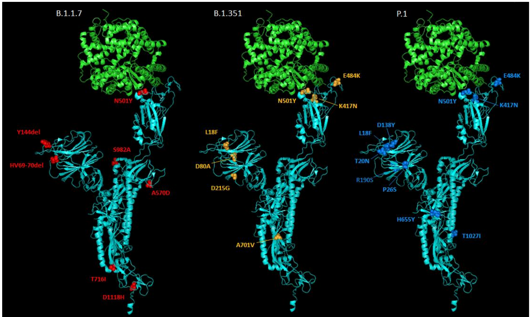
Figure 1. Molecular cartoon diagram of the three-dimensional structure of SARS-CoV-2 spike protein monomer in the open form (cyan) in complex with receptor ACE-2 (green). The image was generated using PyMOL Molecular Graphics System, Version 1.7.0.3 software (Schrödinger, LLC) using cryo-EM data (Protein Data Bank accession number 7DF4.pdb [31]). Amino acid substitutions found in B.1.1.7 (red), B.1.351 (orange) and P.1 (blue) variants are shown.
