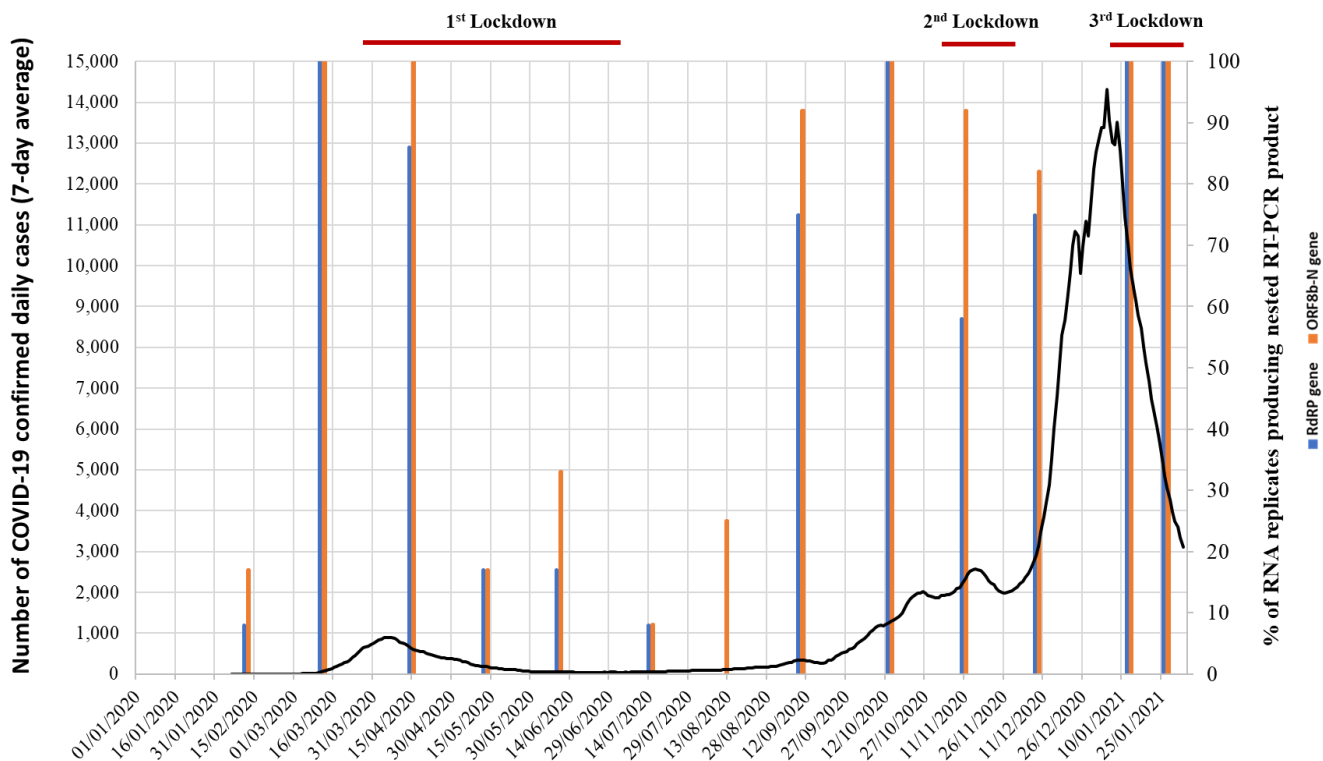
Figure 2. Detection of SARS-CoV-2 RNA in sewage samples collected in London between 14 th January 2020 and 26 th January 2021. The % of RNA replicates producing positive results in nPCR A (blue) and nPCR B (orange) reactions targeting RdRP and ORF8b genomic regions, respectively, are shown as vertical columns. The number of daily confirmed COVID-19 cases in London are represented with a black line (7-day rolling average). Nationwide lockdown periods are indicated as horizontal red lines. Source for COVID-19 cases data:
