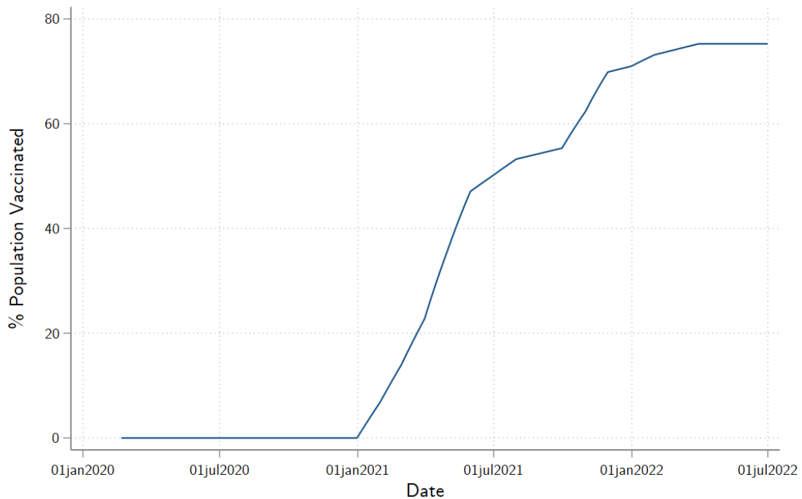
Figure 1. Vaccination Forecast Path
