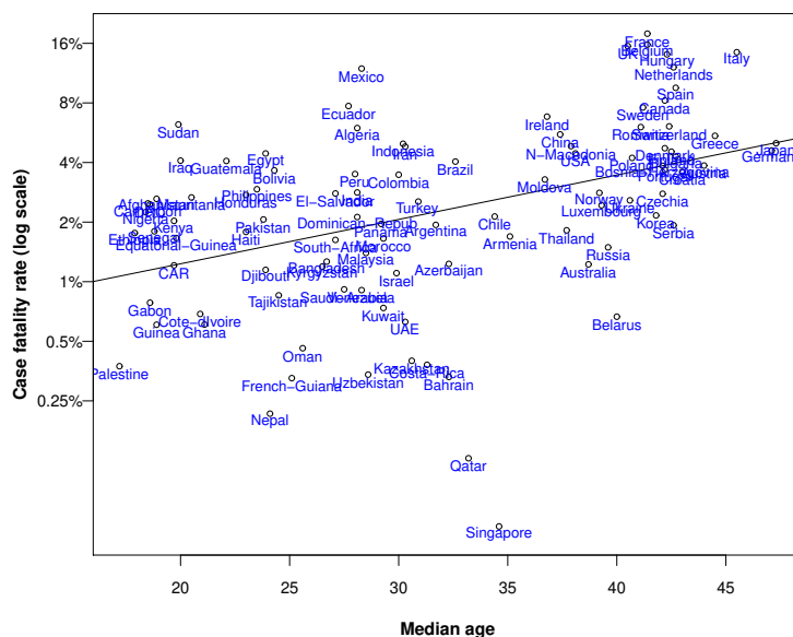
Figure 3: Scatter plot of CFR by median ages for individual countries as of Jul 6, 2020. The solid line is the regression line.
