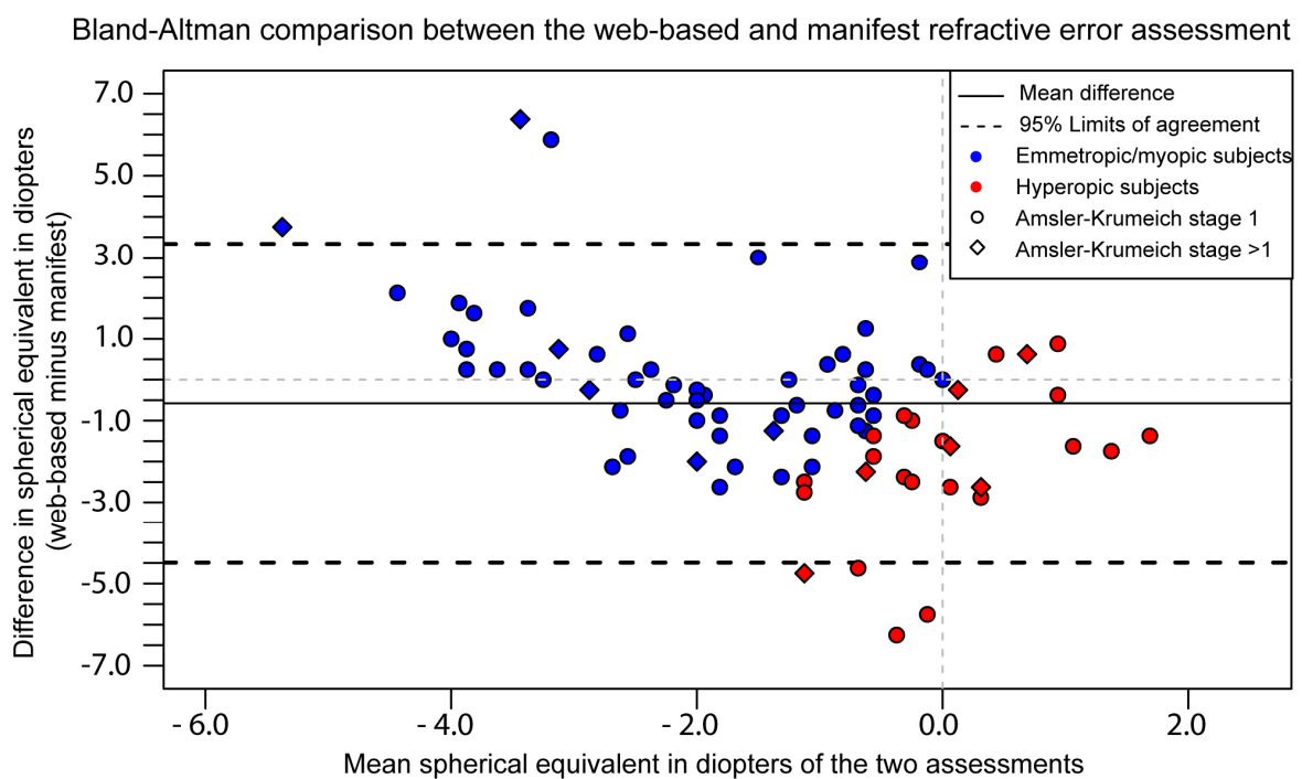
248 Figure 3. A Bland-Altman plot displaying the differences in refractive error between the web-based 249 refractive assessment (index test) and the manifest refraction (reference test). The difference 250 between the reference and index test shown on the Y-axis is expressed as the difference of the web- 251 based refractive assessment outcome compared to the manifest refraction. The x-axis shows the
