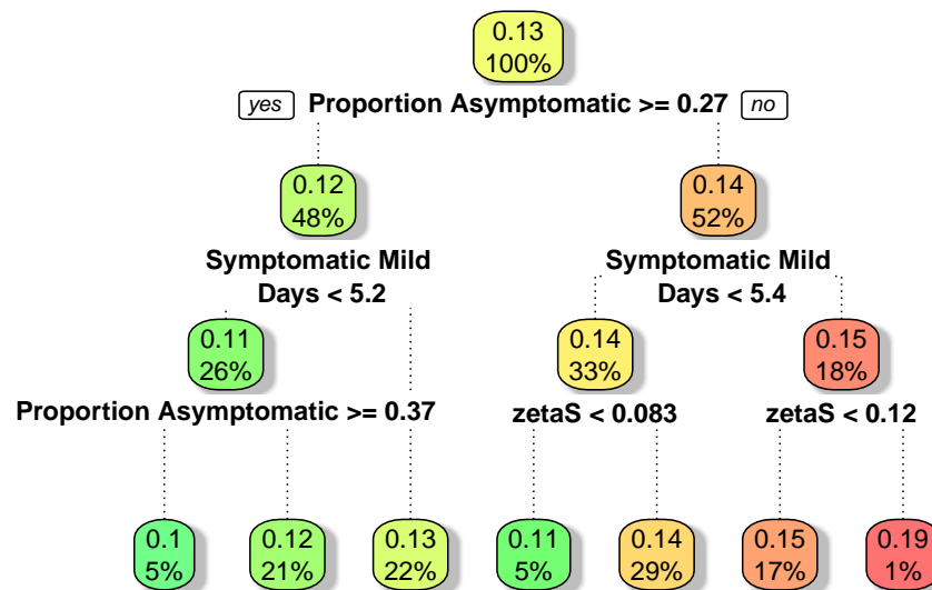
Figure 9: Cumulative Diagnosed CART decision tree.
