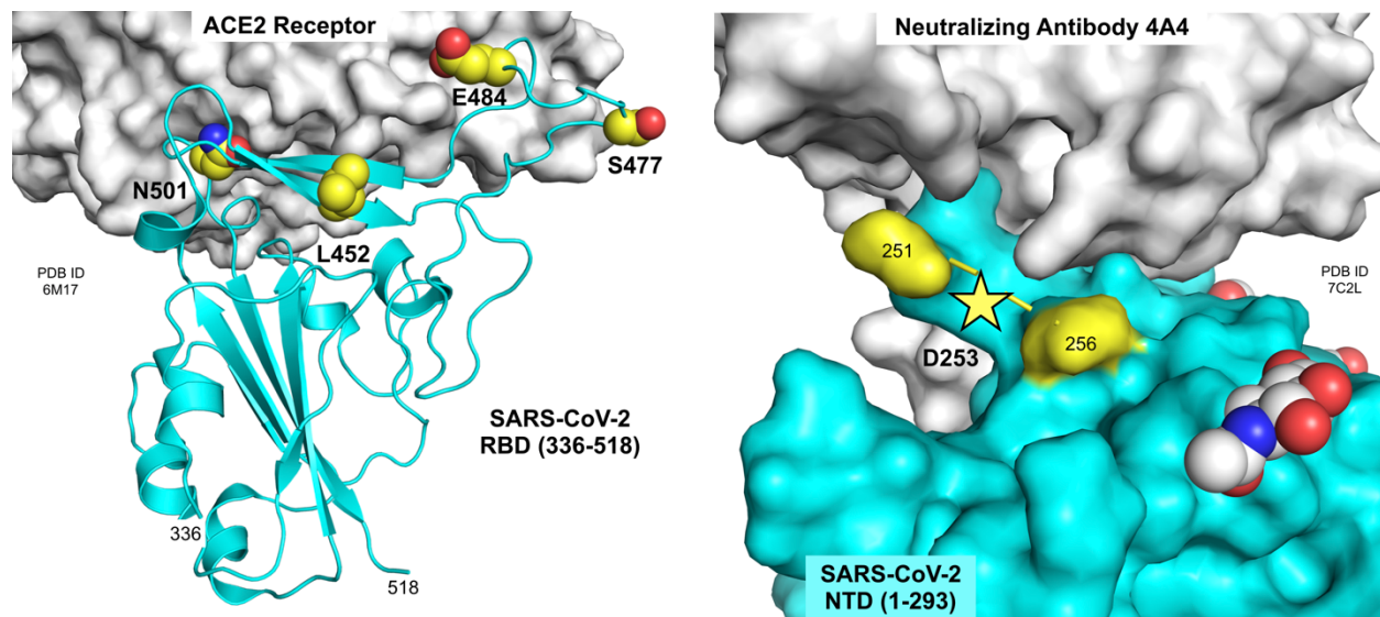
Figure 5. Residues mutated in B.1.526 spike protein. Residues 452, 477, 484 and 501 are located at or near the interface of the RBD with the ACE2 receptor (left panel; PDB ID 6M17, Yan et al., 2020). Residue 253 is located in a small disordered loop in the NTD near the interface with neutralizing antibody 4A4 (right panel; PDB ID 7C2L, Chi et al., 2020). Figure prepared using the PyMOL Molecular Graphics System v2.3.5 (Schrödinger, LLC).
