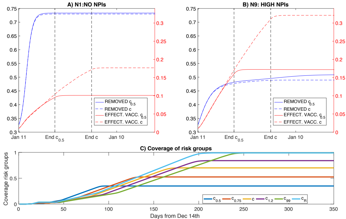
Fig S10 Effect of NPIs and vaccination uptake on population immunity. Panels A and B) Cumulative individuals no longer susceptible or infected (blue lines: recovered + deceased) and effectively vaccinated (red lines: recipients of vaccine who were susceptible) in scenario N1 (NO NPIs, panel A) and N9 (HIGH NPIs, panel B). Dashed blue and red lines refer to uptake scenario c and solid blue and red lines refer to uptake scenario c_{0.5} . Black vertical dashed lines mark the end of vaccination (first doses) in c and c_{0.5} . Panel C) Vaccine coverage of risk groups (adults with RF and population \geq 65 with and without RF) through time from December 14, 2020 for the 6 uptake scenarios ( c_{0.5} , c_{0.75} , c , c_{1.2} , c_{99} , c_R ).
