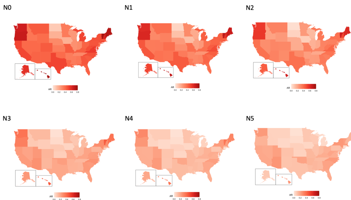
Figure S2 Attack rate by state in scenarios N0 to N5. Maps show the mean estimates of the attack rate (AR) for each state with R_0=2.8 for the 6 scenarios N0 to N5.
