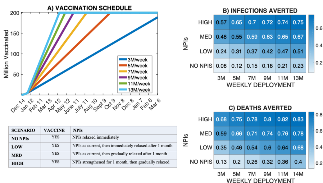
Figure 4 Effect of vaccine administration rate. Panel 3A) shows the vaccine administration timeline for the 6 vaccine deployment rates simulated. Panels 3B) and 3C) show the fractional averted burden of infections and deaths for each combination of administration rate and NPI scenario relative to Scenario N0. NPI scenarios NO NPIS, LOW, MED and HIGH correspond to Scenarios N1, N7, N8 and N9 of Supplementary Table S5.
