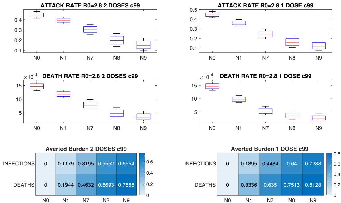
Fig S7 Comparison between one-dose and two-doses vaccination in uptake scenario c99. Left panels show the attack rate, death rate and averted burden for two-dose vaccination with 61.5% coverage and 5 million vaccination per week in uptake scenario c99; right panel show the attack rate, death rate and averted burden for and one-dose vaccination (right) with 99% coverage and 10 million vaccination per week. The NPI scenarios N0, N1, N7, N8, N9 are described in Table S5.
