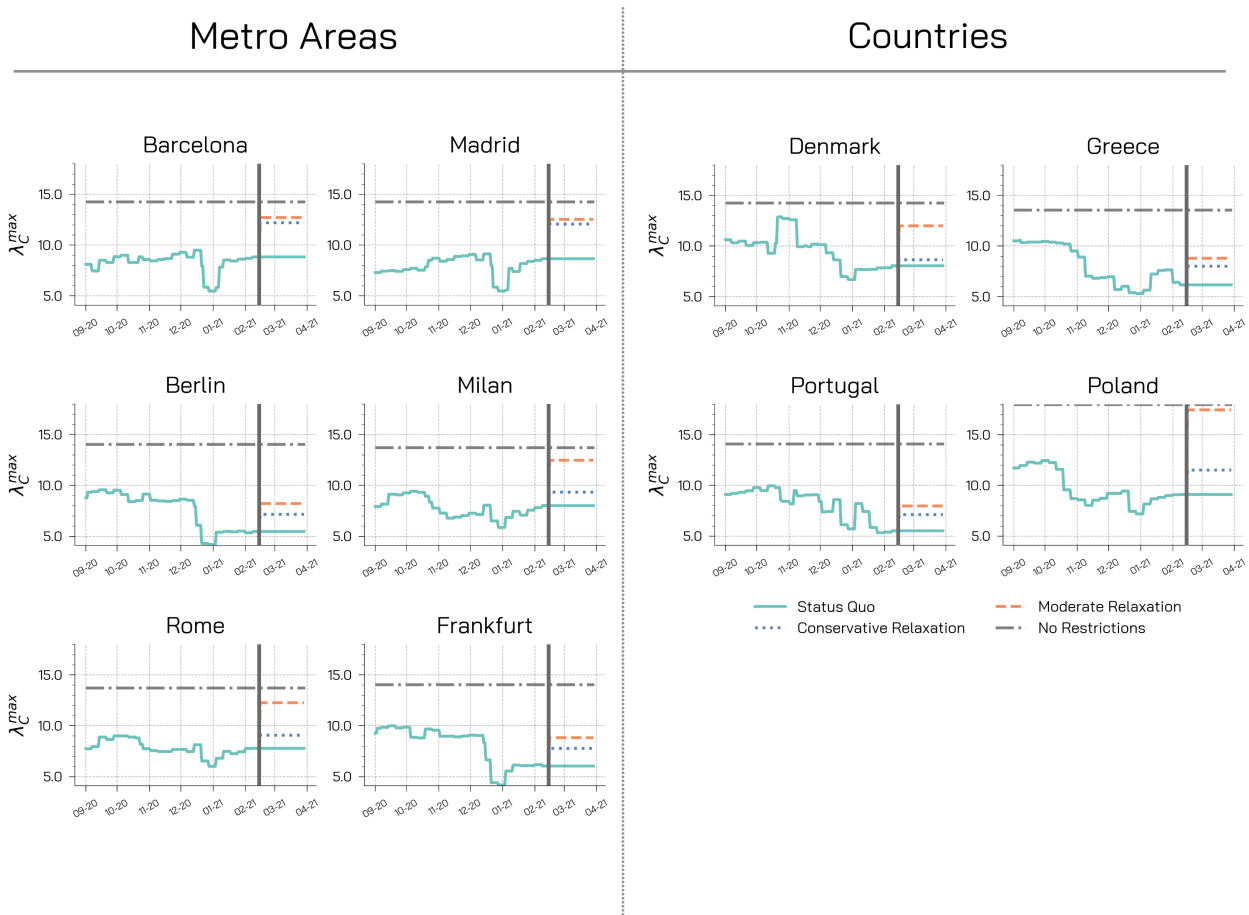
Figure 4: Maximum eigenvalue of the contact matrices. We represent the maximum eigenvalue of the overall contacts matrix over time. The vertical line indicates where the restriction scenarios start. We consider three possible scenarios. In the first scenario ( status quo ), we keep contact matrices unchanged with respect to week 6 of 2021. We then propose two scenarios describing a conservative and a moderate relaxation of social distancing and other NPIs.
