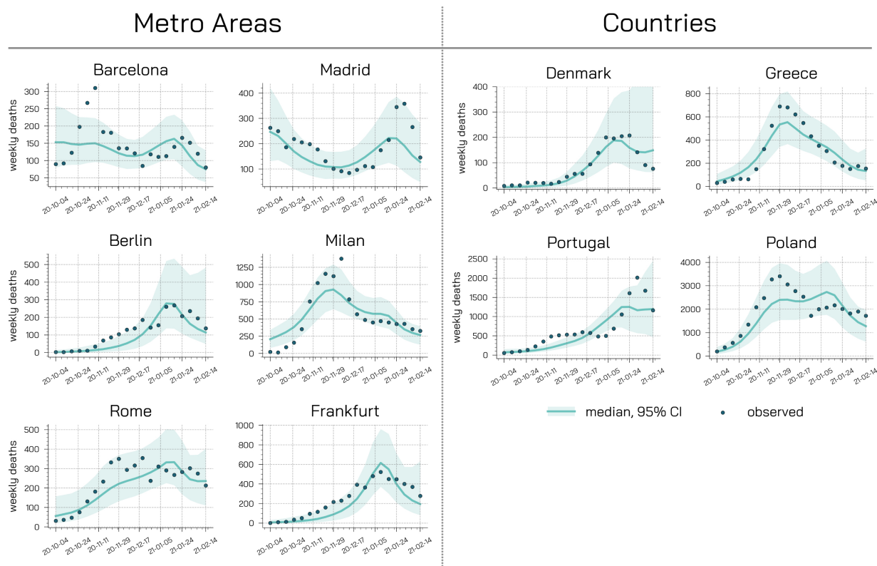
Figure 7: Model adequacy provided by comparing the weekly deaths data with the projections of the calibrated model.
