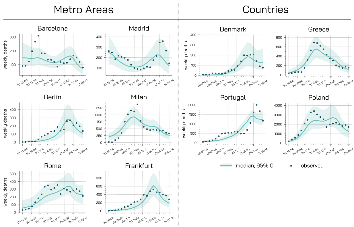
Figure 11: Model adequacy provided by comparing the weekly deaths data with the projections of the calibrated model ( \psi = 0.3 ).
