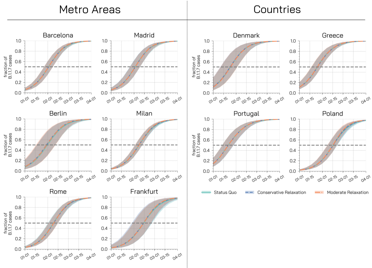
Figure 16: Fraction of new cases attributable to the B.1.1.7 variant. Each plot shows the fraction of new weekly cases attributable to the variant in different regions for different restrictions scenarios under the assumption of a 70% increase in transmissibility. Dashed horizontal lines represent the dominance threshold of 50% of new cases caused by the B.1.1.7 variant. The shaded areas represent the 50% CI.
