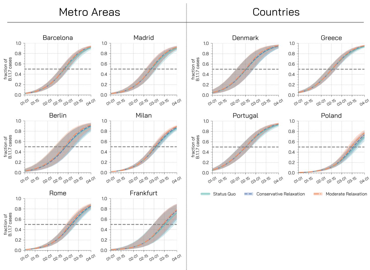
Figure 1: Fraction of new cases attributable to the B.1.1.7 variant. Each plot shows the fraction of new weekly cases attributable to the variant in different regions for different restrictions scenarios under the assumption of a 50% increase in transmissibility. Dashed horizontal lines represent the dominance threshold of 50% of new cases caused by the B.1.1.7 variant. The shaded areas represent the 50% CI.
