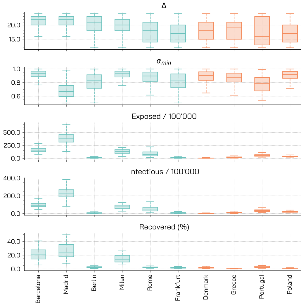
Figure 6: Posterior Distributions - Other parameters. For different regions, we represent the posterior distributions for the delay in deaths \Delta , the seasonality parameter \alpha_{min} , and the initial conditions expressed as total number of initial exposed and infectious per 100'000 and the percentage of initial recovered. These posterior distributions are obtained for \psi = 0.5 and weighted mean absolute percentage error as a distance metric with a tolerance \epsilon of 0.35.
