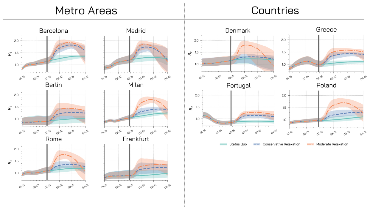
Figure 8: Effective Reproductive Number. Estimate of R_t (median and 90% CI) in different regions for different restrictions scenarios. The B.1.1.7 variant is assumed to have a 50% increase in transmissibility.
