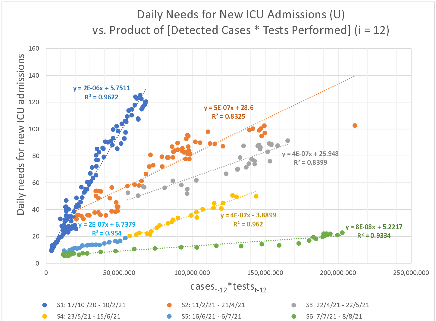
214 Figure 3. Correlation of the numerator and denominator of SDR, i.e. , number U versus the product 215 ( \text{cases}_{t-12} * \text{tests}_{t-12} ), with a lag of 12 days. Numbers of daily tests and detected cases were derived from 216 the period from 17/10/2020 to 8/8/2021.
