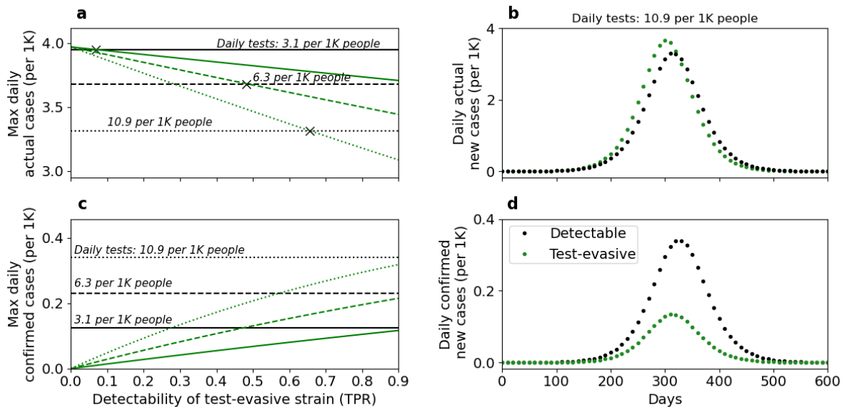
Figure 6. Effects of decreased detectability on epidemiological metrics. These results demonstrate the outcomes of two separate outbreaks: (i) exclusively by a detectable strain (black lines) and (ii) exclusively by a test-evasive strain (green lines), under three testing regimes (solid, dashed, and dotted lines). Panels a and c show the maximum number of actual and test-confirmed daily cases, respectively. Panels b and d show a timeline of these epidemiological metrics for a relatively high testing rate and low detectability. Higher detectability of the test-evasive strain increases the daily number of confirmed cases (panel c , green lines) and decreases the daily number of actual cases (panel a , green lines). The effect of detectability on the number of daily actual cases is associated with the cost of infectiousness, c , producing a detectability threshold (panel a , marked with 'X'), above which the number of actual daily cases for the test-evasive strain is lower than for the detectable strain (see Fig. S4 for the effect of decreased detectability without cost of infectiousness). A higher testing rate increases the number of confirmed cases (panel c , compare solid, dashed and dotted lines) and decreases the number of actual cases (panel a , compare solid, dashed and dotted lines). Overall, when testing rate is high and the epidemic is driven by a test-evasive strain with low detectability (panels b and d ), the number of confirmed cases is lower compared to an epidemic driven by a detectable strain, while the number of actual cases is higher. Here, \beta = 0.42 (Impact of NPI = 0.65), \mu = 0.6 , \alpha_1 = 0.6 , \alpha_2 = 0.6 , d_1 = 0.9 , c = 0.01 . For panels b and d , d_2 = 0.3 , p = 10.9 per 1K people.
