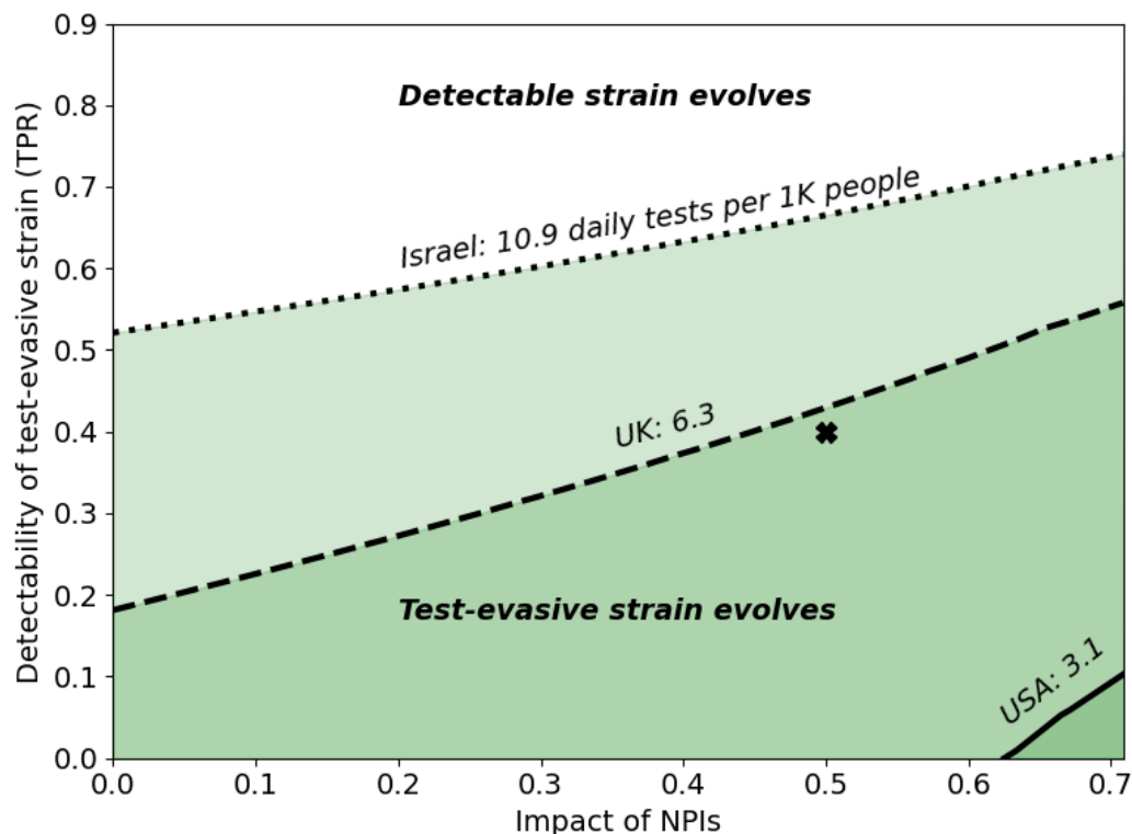
Figure 5. High testing rate and effective NPIs favor the evolution of test-evasive strains.
