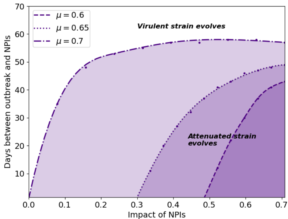
Figure 3. Earlier start of NPIs favors the evolution of the attenuated strain. Each curve corresponds to a different relative transmissibility of infection by asymptomatic individuals, \mu . The colored areas below each curve show the regions in which the attenuated strain evolves. The areas above each of the curves show the regions in which the virulent strain evolves. Here, \beta_{\min} = 0.35 , \beta_{\max} = 1.2 , \alpha_1 = 0.6 , \alpha_2 = 0.05 .
