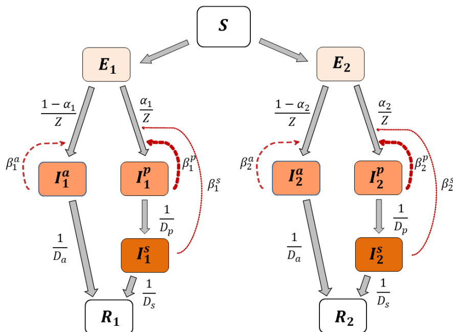
Figure 1. Evo-epidemiological model. Our model follows two viral strains simultaneously spreading in an initially susceptible population. Susceptible ( S ) individuals become exposed ( E ) after contact with an infected individual with rate \beta^x (where x=p, s , or a is the class of infected individual). Exposed individuals ( E ) undergo an incubation period during which they are not infectious. After an average incubation period of Z days, exposed individuals become infected, with either a presymptomatic ( I^p ) or asymptomatic ( I^a ) infection, with probability \alpha and (1 - \alpha) , respectively. Asymptomatic individuals ( I^a ) are infectious but asymptomatic from disease onset until recovery. Presymptomatic individuals ( I^p ) are infectious and may be asymptomatic or exhibit mild symptoms for several days, after which they exhibit clinical manifestation of the disease ( I^s ) and are therefore isolated. Symptomatic and asymptomatic cases become recovered ( R ) after an average of D_s and D_a days, respectively.
