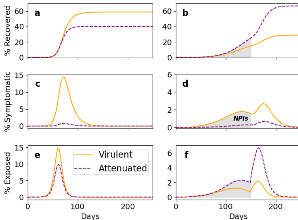
Figure 4. Temporal application of NPIs favors the evolution of the attenuated strain.
