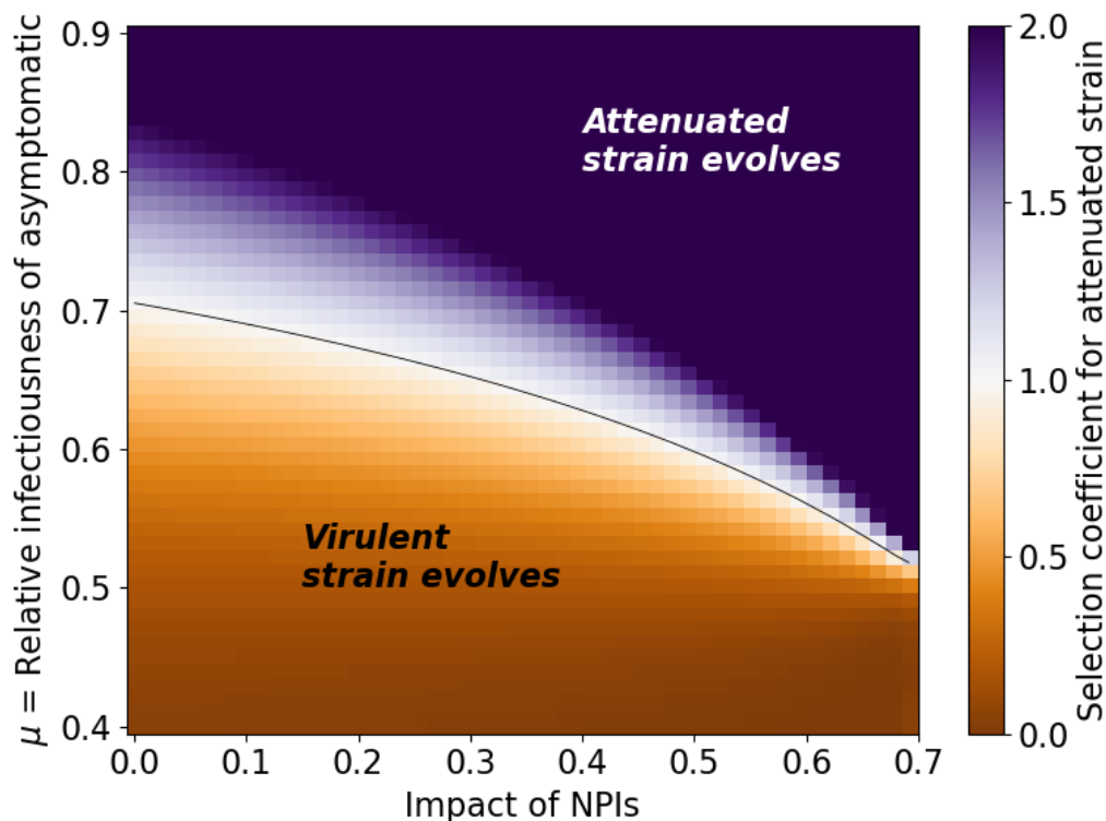
Figure 2. Effective NPIs facilitate the evolution of the attenuated virus. This figure presents the conditions for evolution of either the attenuated (purple) or the virulent (orange) strains under constant NPIs. High impact NPIs (right side) facilitate the evolution of the attenuated strain, while low impact NPIs (left side) facilitate the evolution of the virulent strain. The attenuated strain can also evolve if asymptomatic individuals are infectious enough relative to presymptomatic individuals ( \mu is high, top side). Here, \beta_{\max} = 1.2 , \alpha_1 = 0.6 , \alpha_2 = 0.05 .
