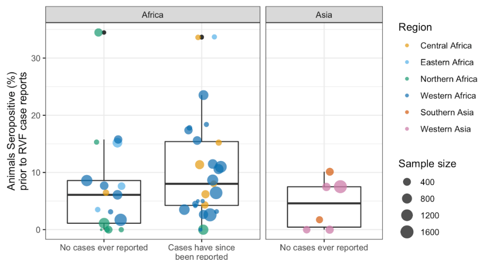
Figure 5: Rift Valley fever virus seroprevalence when RVF cases had never been reported in the country (human and/or animal). The outliers represent samples from Tunisia, no known RVF cases, during 2017-2018 (34.5% positive of 470 camels) [57], and two countries currently known to report RVF cases, South Sudan in 1979-1983 (33.7% positive of 92 ruminants, cattle and goats) [58], and Cameroon in 1968 (33.6% of 122 sheep) [59].
