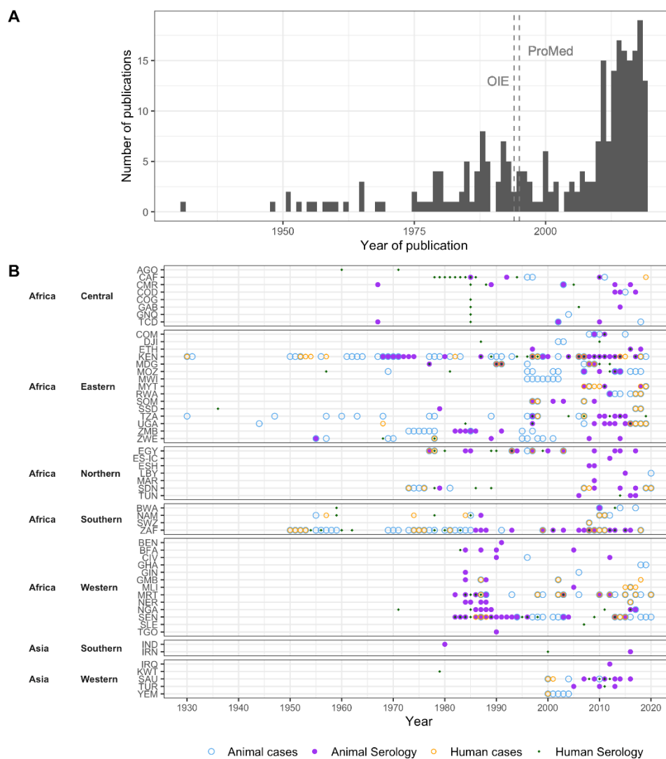
Figure 2. Regional variation in RVF reports and seroprevalence studies over time A) Number of included publications by year. Vertical lines represent the first year during which OIE and ProMED reports were included. B) For each country, the years during which Rift Valley fever cases were reported, and the years during which Rift Valley fever virus seroprevalence data were collected are marked for animals and humans. When results from multiple years were reported as one, e.g. 1991-2000, we marked the first year in the figure. Serological data also include studies where no RVFV antibodies were detected, note that this is not a RVFV detection chart.
