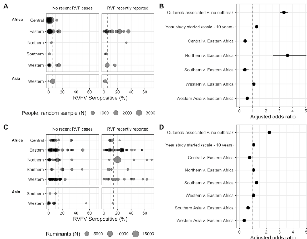
Figure 4: Regional human (A, B) and ruminant (C, D) RVFV seroprevalence in the absence of recent human and/or animal RVF cases or within the same year, or year post, reported RVF cases. A and C) Sample size and seroprevalence per country and year. The grey, dashed vertical line represents the overall mean seropositivity in humans (A) and ruminants (C). Note: dots can overlap. B and D) Adjusted odds ratio for odds of detecting a seropositive person (B) or ruminant (D). The grey,
