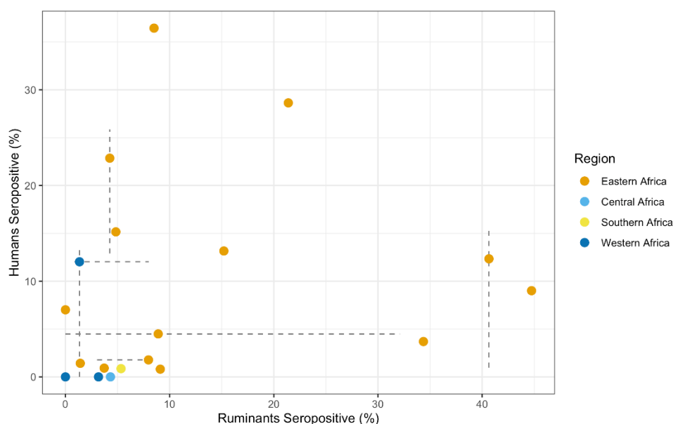
Figure 6: Animal and human RVF seroprevalence data from the same year and country. Point estimates represent mean seropositivity (percent of individuals testing positive of the total number of individuals tested), and lines represent the range in seroprevalence estimates reported when multiple publications were included in the prevalence estimate.
