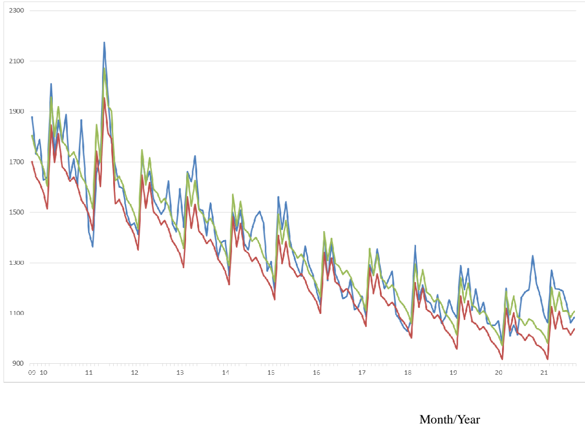
Figure 1: Observations of the estimated baseline and threshold for suicide deaths from October 2009 through September, 2021, among males.
