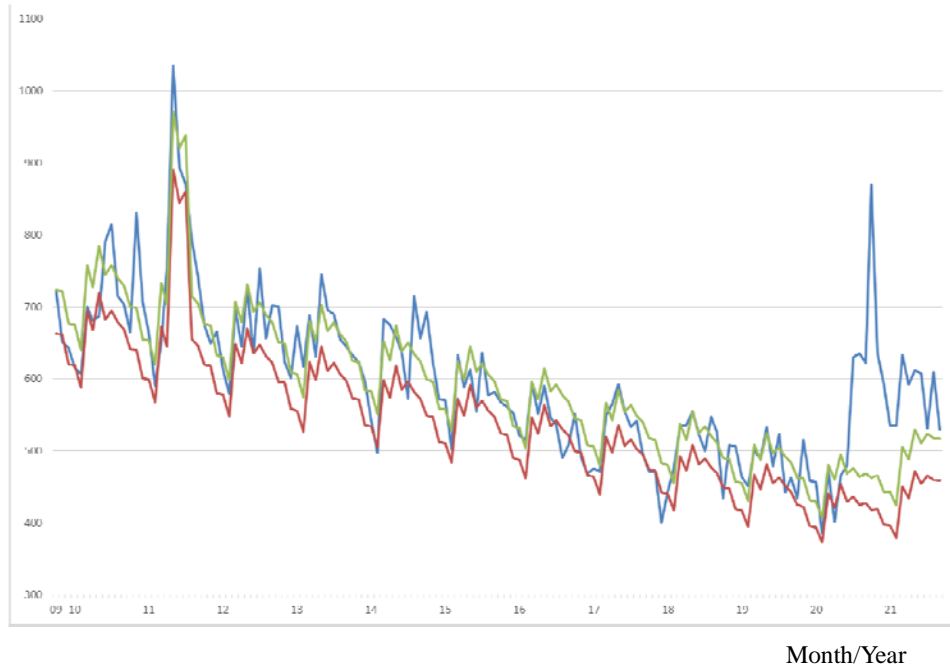
Figure 2: Observations of the estimated baseline and threshold for suicide from October 2009 through September, 2021, among females.
