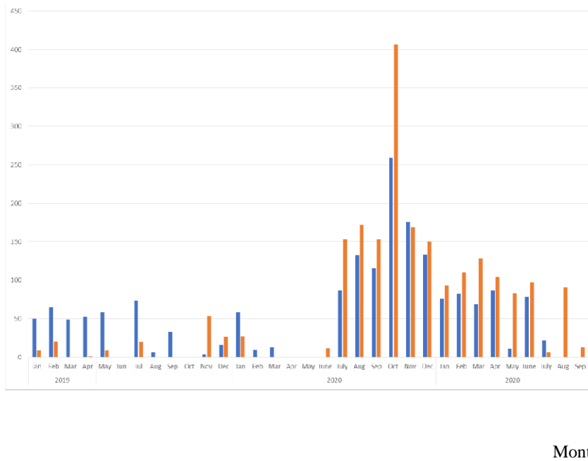
Figure 3: Excess mortality in suicide by gender since 2019 by month in Japan. (persons)
