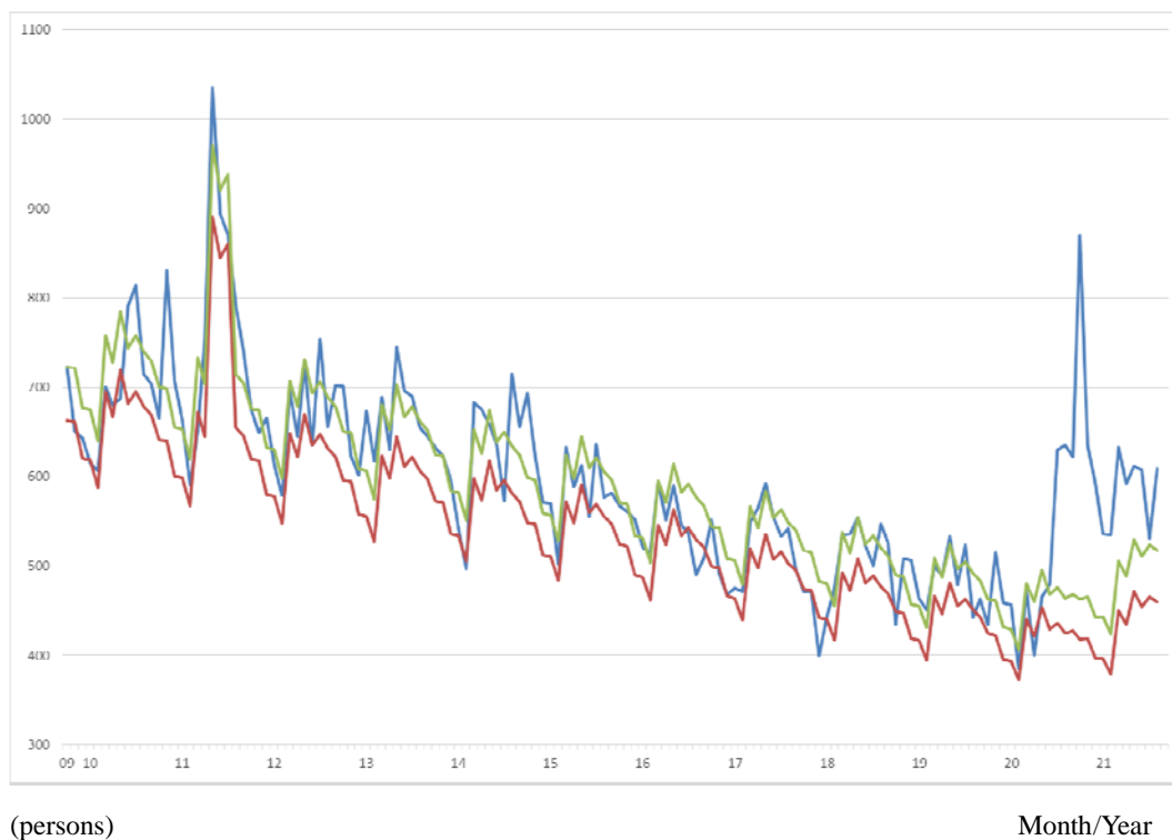
Figure 2: Observations of the estimated baseline and threshold for suicide from October 2009 through August, 2021, among females.
