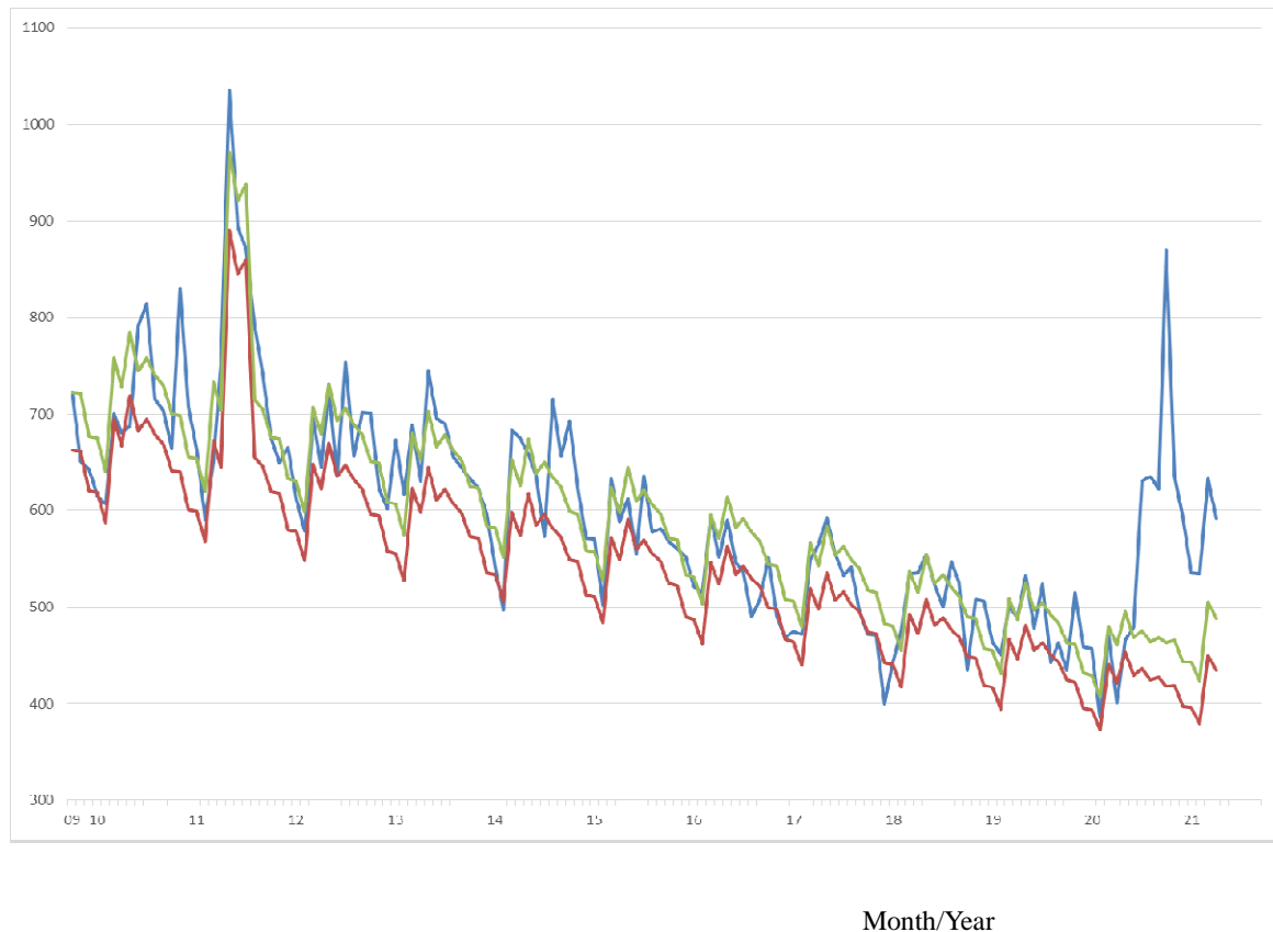
Figure 2: Observations of the estimated baseline and threshold for suicide from October 2009 through May, 2021, among females.
