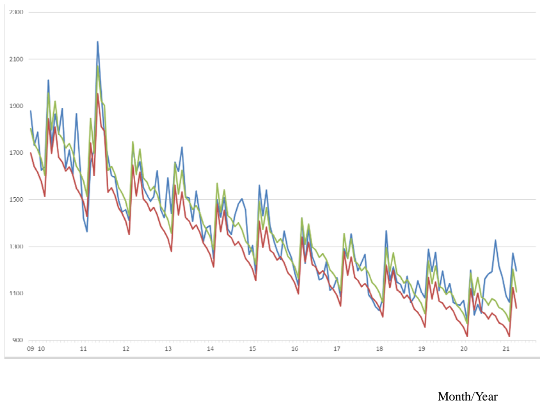
Figure 1: Observations of the estimated baseline and threshold for suicide deaths from October 2009 through May, 2021, among males.
