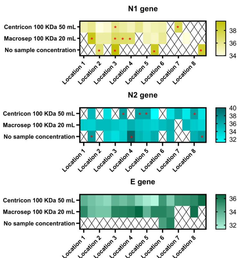
293 294 Figure 4 Comparison of sample concentration methods in IWW from 8 Belgian WWTPs. The colour of each cell represents 295 the Ct-value. Cells indicated with a red asterisk have higher Ct-values than the lowest point of the calibration curve and could 296 therefore not be quantified. However, in these cells a positive signal was still detected. No signal was detected in cells with a black 297 cross. Side-by-side cells for each location represent duplicate Ct-values. The Maxwell PureFood GMO and Authentication kit was 298 used for RNA extraction.
