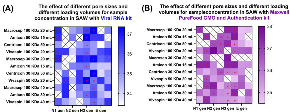
275 276 Figure 3 Optimization of pore sizes and loading volumes with the different sample concentration methods in SAW using 277 (A) the Viral RNA extraction kit and (B) the Maxwell PureFood GMO and Authentication kit. The colour of each cell 278 represents the Ct-value. Cells indicated with a red asterisk have higher Ct-values than the lowest point of the calibration curve 279 and could therefore not be quantified. However, in these cells a positive signal was still detected. No signal was detected in cells 280 with a black cross. Side-by-side cells for each location represent duplicate Ct-values.
