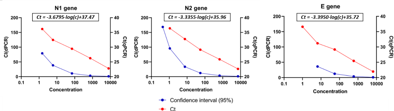
351 352 Figure 5 Evaluation of the precision of the standard curve with dPCR as a means to validate qPCR results. CI = confidence 353 interval; Ct = cycle threshold. The left y-axis represents the precision of the 95% confidence interval after running the standard 354 curve with dPCR. The right y-axis represents the Ct-values measured at the different concentration levels with qPCR.
