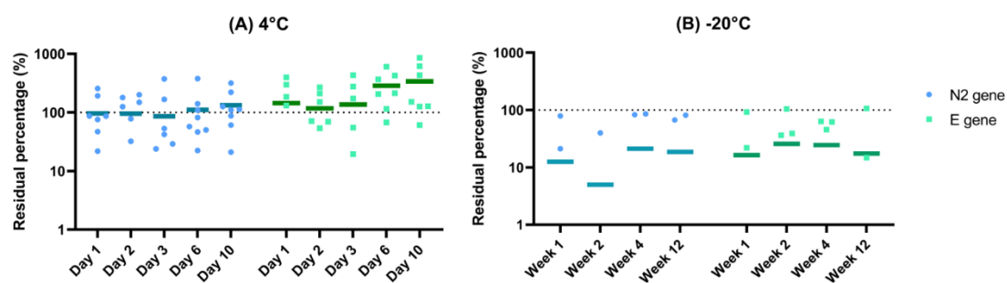
356 357 Figure 6 In-sample stability of the different SARS-CoV-2 genes at (A) 4 °C and (B) -20 °C. The horizontal lines represent 358 the mean residual percentage for the eight samples. Detection of the N1-gene was generally low in the IWW samples (i.e. 10-1 359 copies/ \mu L) with Ct-values below the LLOQ in most samples. Therefore, it was not possible to assess in-sample stability for the 360 N1-gene.
