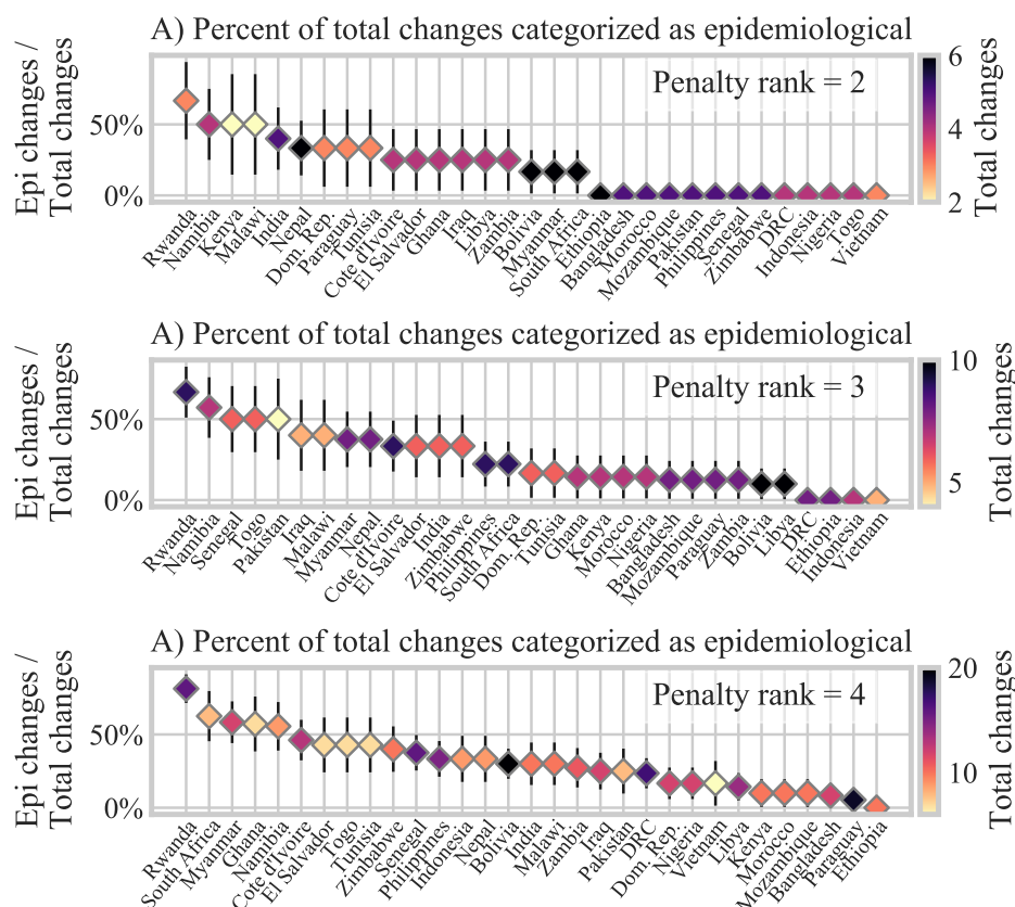
Figure A.11: Countries ranked by epidemiological change detection rate, as in Figure 7, shown for different choices of penalty parameterization. Order top to bottom follows order of time series of Figure A.10, without rank one for which there are often no changes.
