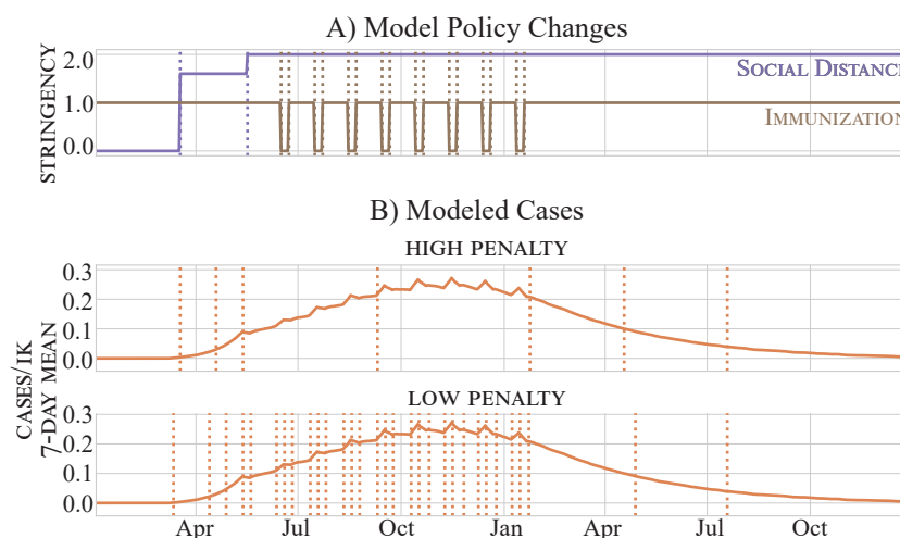
Figure 3: Synthetic model time series; detected change points shown as vertical dotted lines. A) Imposed policy inputs to model: social distancing (purple) and immunization campaigns (brown). Short-term immunization campaigns represented by a switch in the immunization time series from one to zero. B) Model output: case rates over time. Upper plot shows detected change points using a high penalty, thereby promoting sparse change point detection. Lower plot shows detected change points using a low sparsity penalty.
