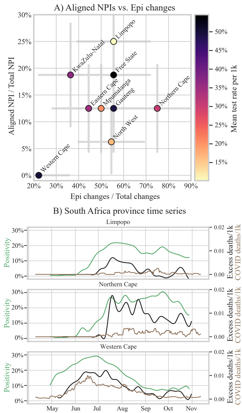
Figure 9: A) South African provinces by aligned NPI fraction versus epidemiological detection rate with mean testing rate in color. B) Time series from three example provinces. Positivity shown in green on left y-axis. Deaths shown on the right y-axis: excess mortality in black; COVID-19-confirmed deaths in brown.
