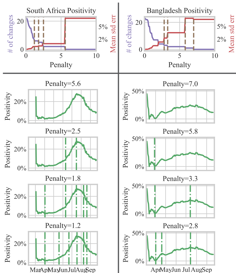
Figure A.10: Top row: change detection results over parameter space for the positivity time series of South Africa (left) and Bangladesh (right). For each penalty value, the associated number of changes is plotted in purple on the left y-axis and the mean standard error of linear regressions of the time series segments are plotted on the right y-axis. The parameter values selected to represent plateaus are shown as brown dotted vertical lines. Bottom row: positivity time series for South Africa (left) and Bangladesh (right) plotted with detected changes as vertical lines for each of the four penalty values selected to represent plateaus in the top row.
