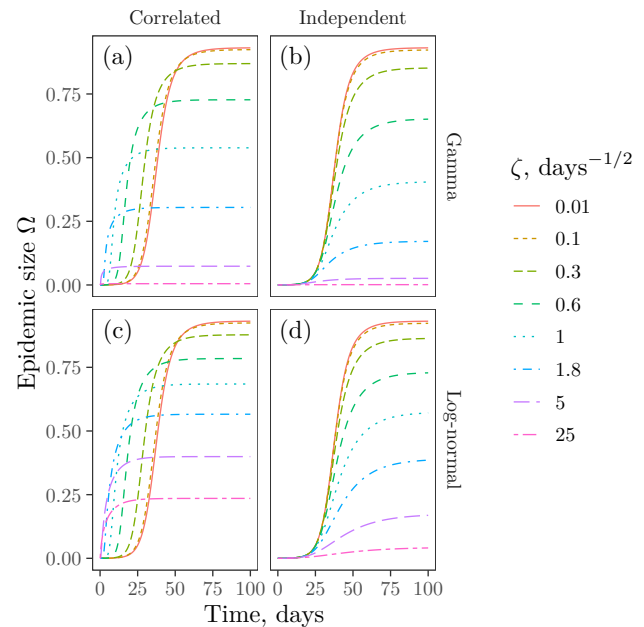
Figure 2. Comparison of epidemics spread for Gamma [panels (a)–(b)] and log-normal [panels (c)–(d)] distributions of infectivity and susceptibility with standard deviation \zeta and parameters in equation (31). The cases of independent or completely correlated \sigma and s are shown.
