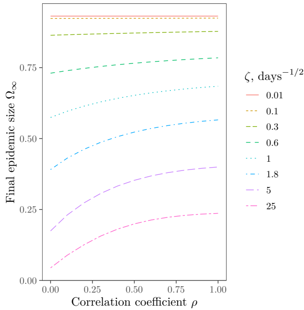
Figure 3. Dependence of final epidemic size \Omega_\infty on \rho where [\ln(s), \ln(\sigma)] is a Gaussian vector with mean \mathbb{E}[s] = \mathbb{E}[\sigma] = 0.6 \text{ day}^{-1/2} , \text{Var}(s) = \text{Var}(\sigma) = \zeta^2 and correlation \mathbb{E}[s\sigma] = \mathbb{E}[s]\mathbb{E}[\sigma]\exp(\rho\zeta^2) with \zeta^2 \equiv \ln[1 + \zeta^2/(\mathbb{E}[s]\mathbb{E}[\sigma])] . Note that \rho is the correlation coefficient for \ln(s) and \ln(\sigma) rather than for s and \sigma .
