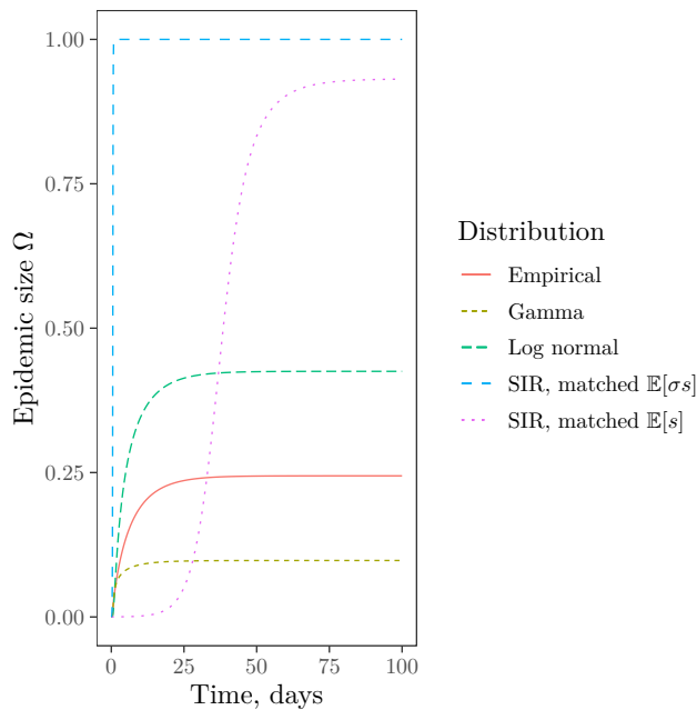
Figure 4. Epidemics progression for the distributions shown on Figure 1 with parameters in equation (31). A classical SIR solution with the same susceptibility and infectivity is also shown.
