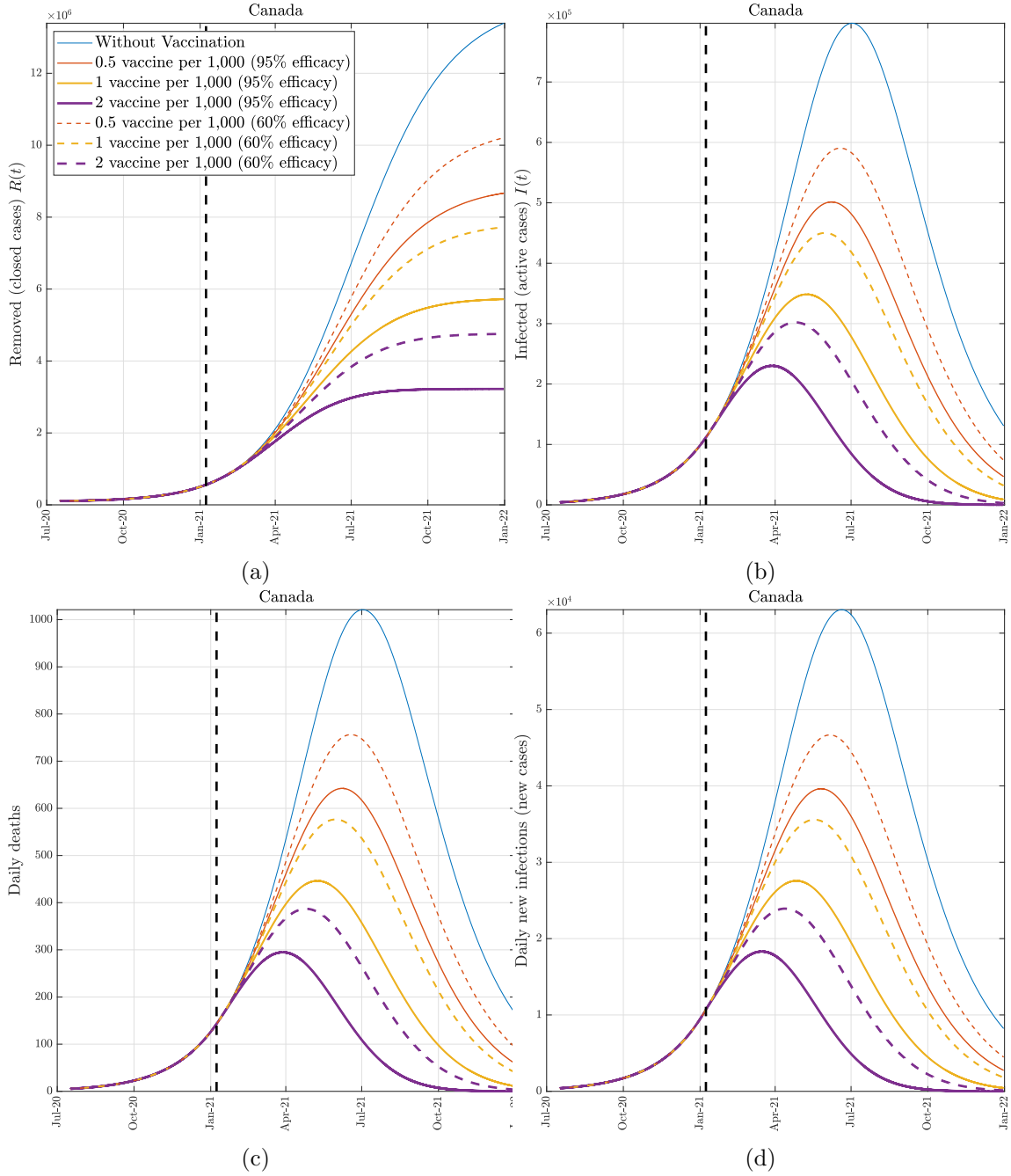
Figure 2: The effect of vaccination (Canada) . COVID-19 epidemic evolution in Canada predicted by the proposed model from January 8, 2021 to December 31, 2021. The colored (solid and dashed) lines represent the four boundary scenarios. We consider two derivative scenarios for the vaccine efficacy: an optimistic scenario at 95% efficacy (solid lines) and a pessimistic scenario at 60% efficacy (dashed lines). The dashed vertical line identifies January 8, 2021.
