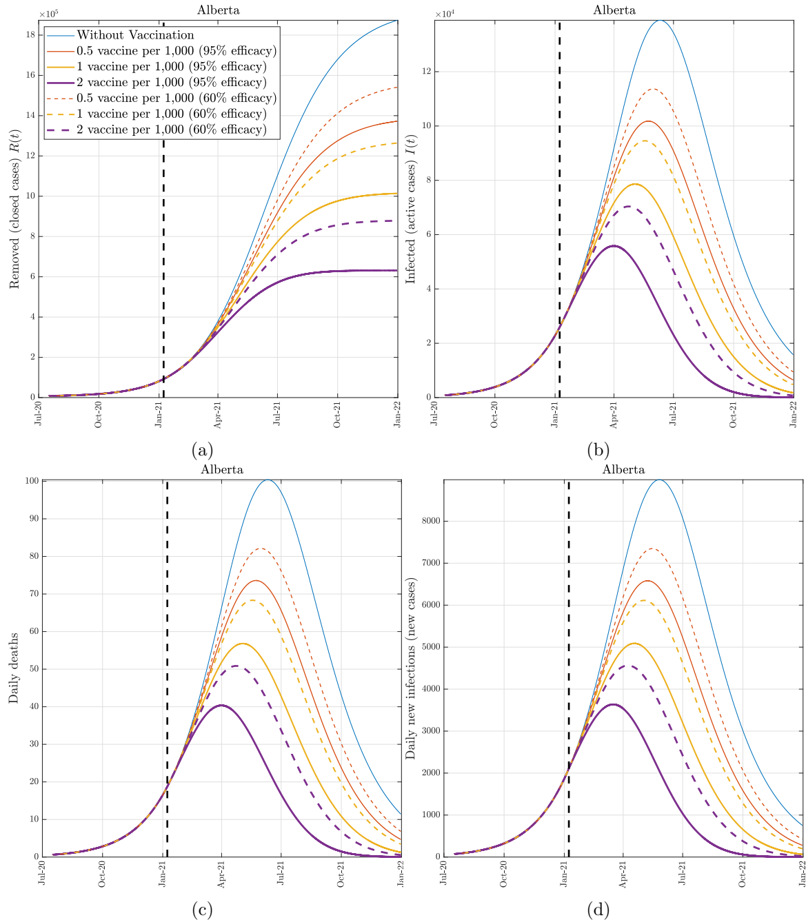
Figure 6: The effect of vaccination (Alberta) . COVID-19 epidemic evolution in Alberta predicted by the proposed model from January 8, 2021 to December 31, 2021. The colored (solid and dashed) lines represent the four boundary scenarios. We consider two derivative scenarios for the vaccine efficacy: an optimistic scenario at 95% efficacy (solid lines) and a pessimistic scenario at 60% efficacy (dashed lines). The dashed vertical line identifies January 8, 2021.
