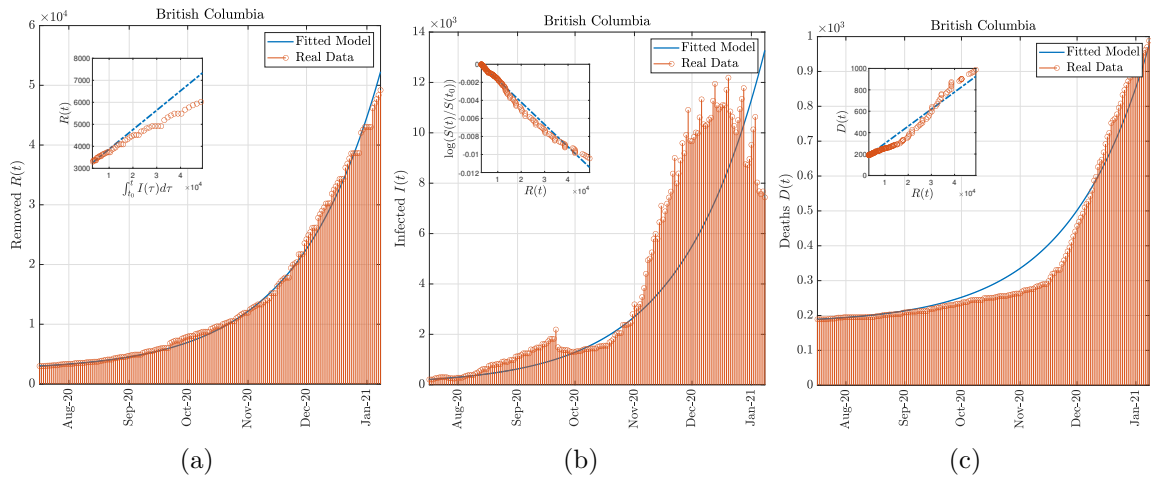
Figure 12: Model simulation compared to real data (British Columbia) . Comparison between the official data (red dots histogram) and the results with the calibrated SIR model (blue line). Panel (a): number of reported removed cases (deaths and recovered). Panel (b): number of reported infected. Panel (c): number of cumulative deaths. The real data covers the period between July 17, 2020 and January 8, 2021.
