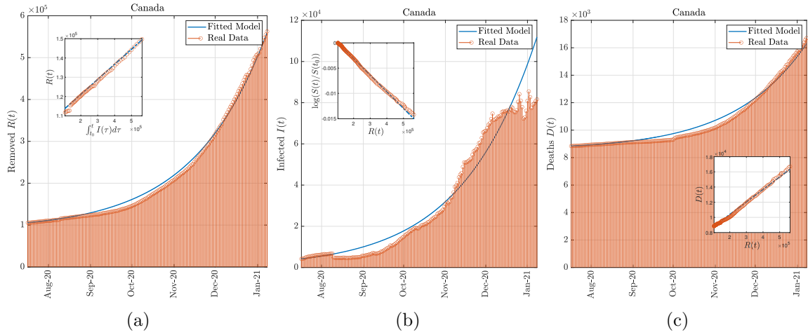
Figure 9: Model simulation compared to real data (Canada) . Comparison between the official data (red dots histogram) and the results with the calibrated SIR model (blue line). Panel (a): number of reported removed cases (deaths and recovered). Panel (b): number of reported infected. Panel (c): number of cumulative deaths. The real data covers the period between July 17, 2020 and January 8, 2021.
