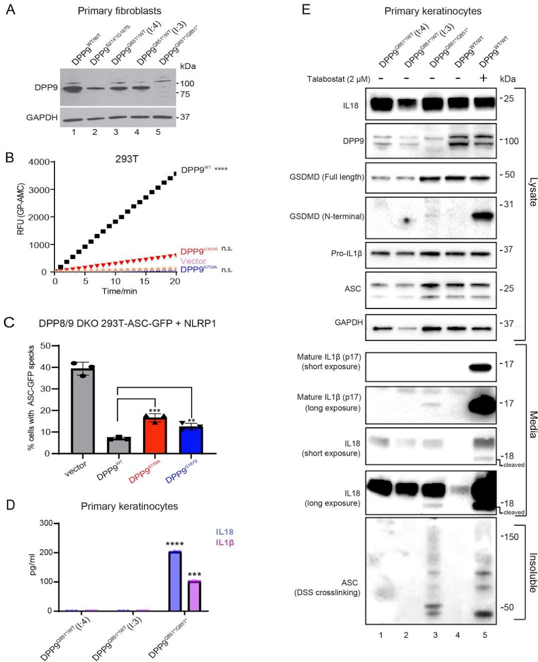
Fig. 2: Patients' cells lack DPP9 or produce a strong enzymatic hypomorph
