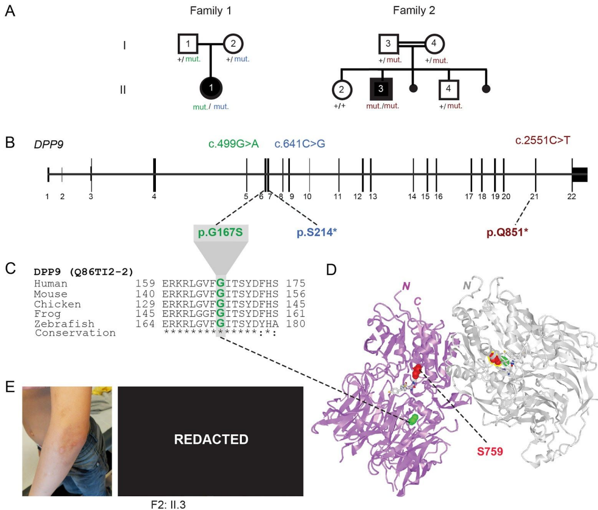
Fig. 1: Two families segregating recessive DPP9 germline mutations
