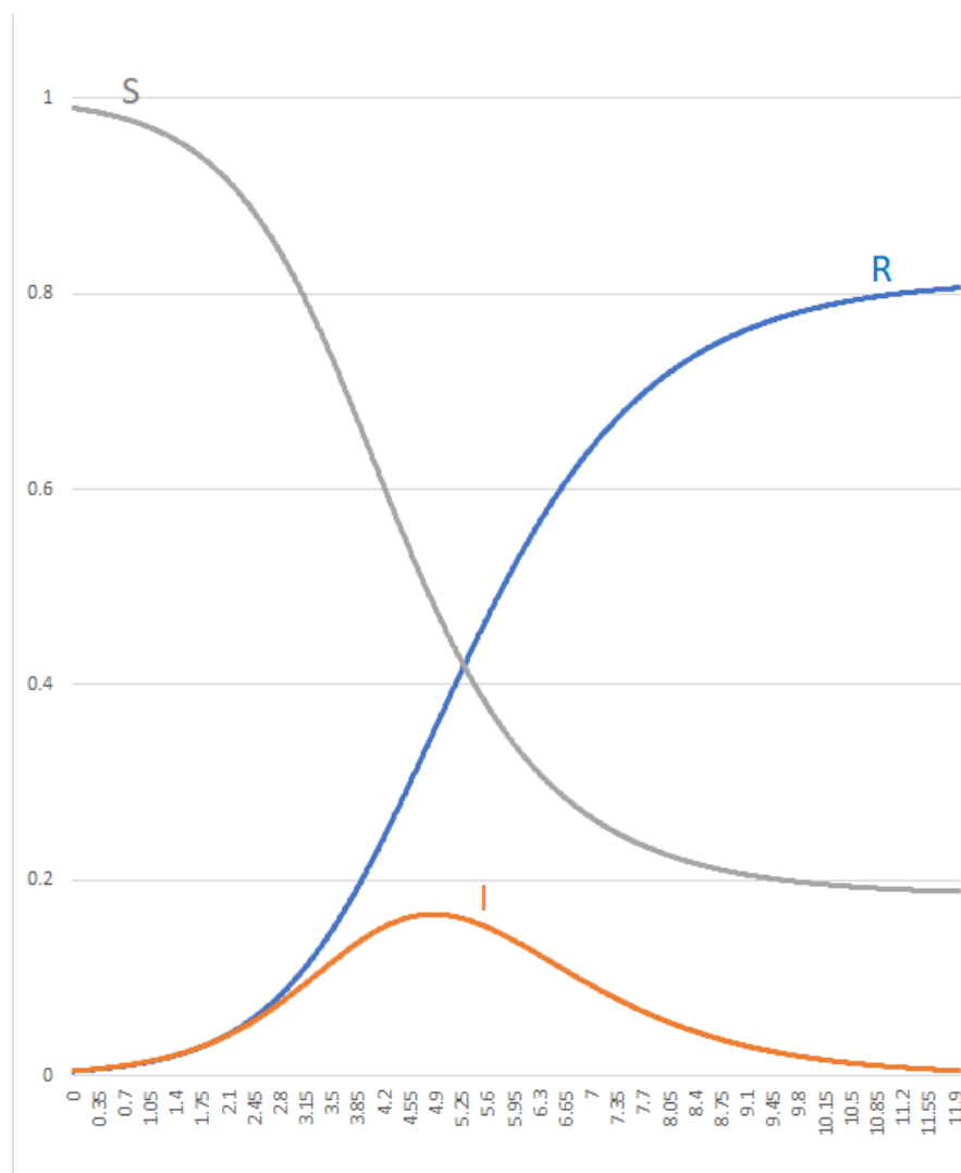
Figure 1: Graph of S , I and R for \alpha = 2.07 and c = 0.041
