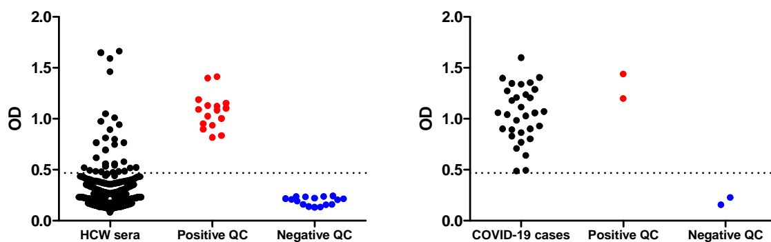
Figure 3: Anti-SARS-CoV-2 antibodies in samples from COVID-19 patients and HCWs in Riyadh, Saudi Arabia.
