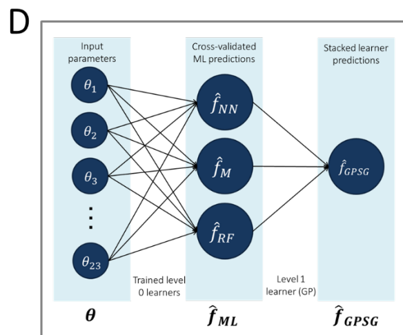
Gaussian process stacked generalization
