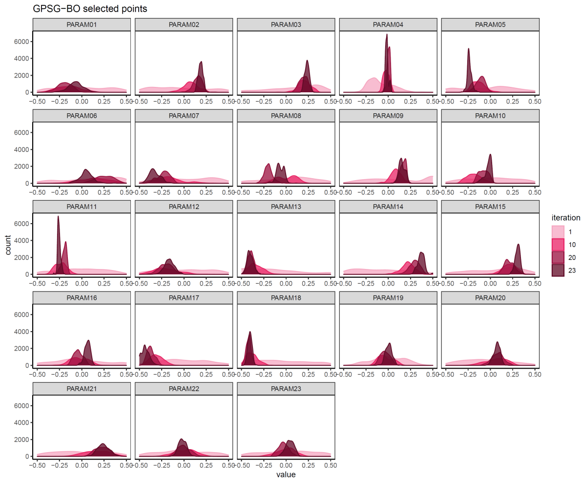
Figure S7. GPSG-BO sampling behavior. Values in each dimension of the points sampled during adaptive sampling of GPSG-BO algorithm in iterations 1,10, 20, and 23.
