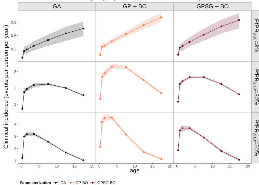
Figure S25. Yearly incidence of clinical malaria in a seasonal transmission setting as a function of age, displayed by transmission intensity ( PfPR_{2-10} ) and parameterization. Clinical incidence is presented in terms of the yearly number of events per person. The PfPR_{2-10} categories include simulated prevalences of 2.5-3.5%, 9-10%, 28-32%, and 47-53% labeled as 3%, 10%, 30%, and 50%, respectively.
