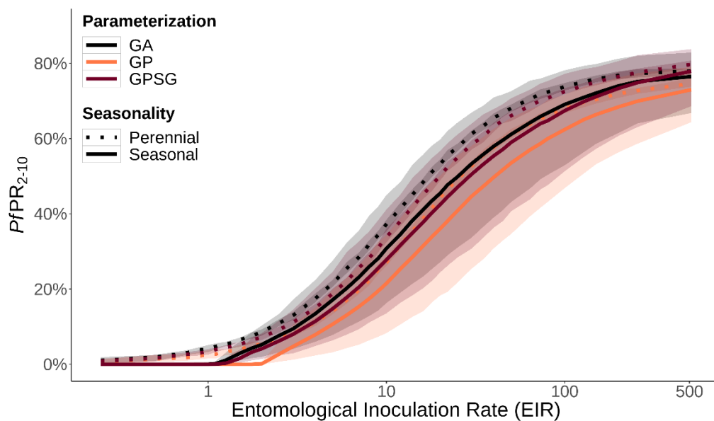
Figure S21. Relationship between EIR and PfPR_{2-10} under three parameterizations. Solid lines show medians and shaded regions show 95% credible intervals. EIR denotes the entomological inoculation rate.
