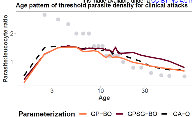
Figure S14. Objective 6. Age pattern of threshold parasite density for clinical attacks. Final simulator fit using the parameter sets yielded using GP-BO and GPSG-BO compared to the previous parameterization (derived using optimization with a genetic algorithm, GA-O).
