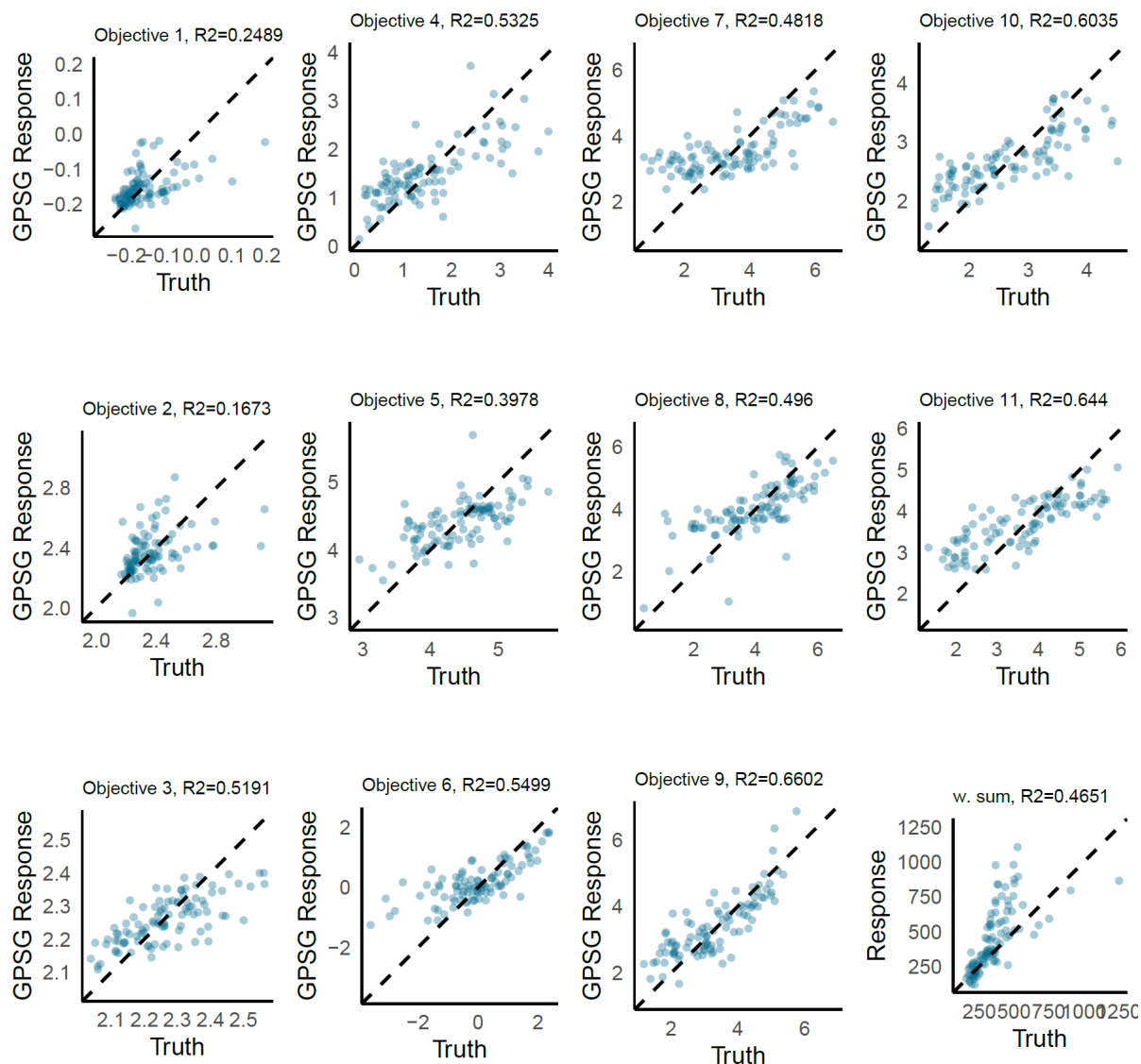
Figure S5. GPSG emulator performance. Emulator predictions vs true values on a holdout set compromising 10% of initial samples in iteration 23 (final iteration). w.sum is the weighted sum F , of the 11 objectives. Here, predictions are generated as the weighted sum of individual objective predictions.
