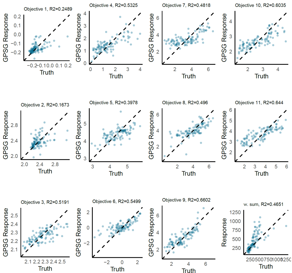
Figure S5. GPSG emulator performance. Emulator predictions vs true values on a holdout set comprising 10% of initial samples in iteration 23 (final iteration). w.sum is the weighted sum F , of the 11 objectives. Here, predictions are generated as the weighted sum of individual objective predictions.
