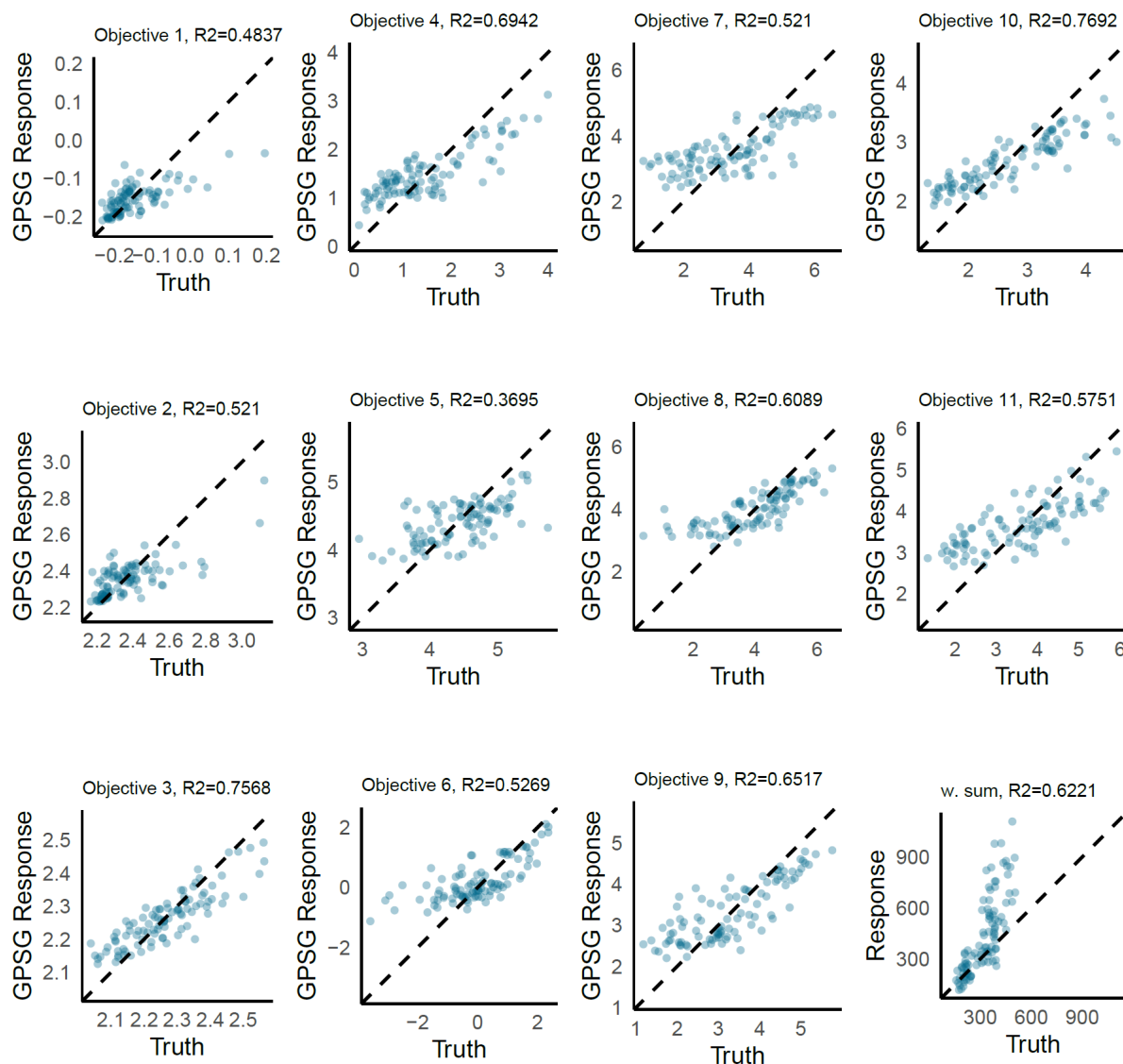
Figure S4. GPSG emulator performance. Emulator predictions vs true values on a holdout set compromising 10% of initial samples in iteration 1. w.sum is the weighted sum F , of the 11 objectives. Here, predictions are generated as the weighted sum of individual objective predictions.
