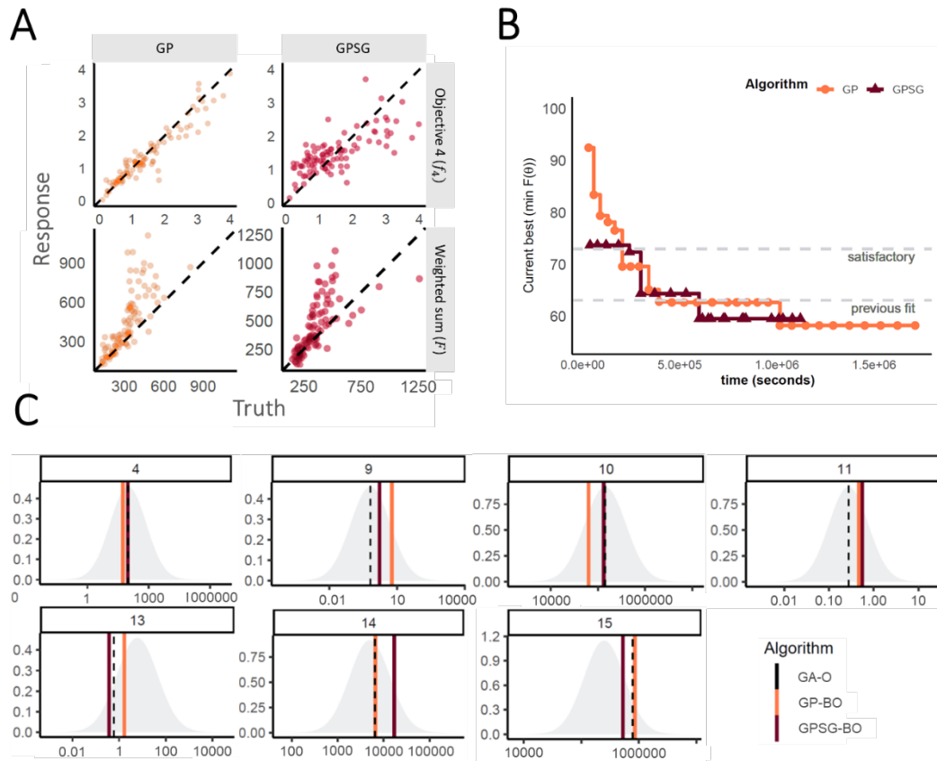
Fig. 2. Emulator performance. A. Example of emulator predictions vs true values on a 10% holdout set.
