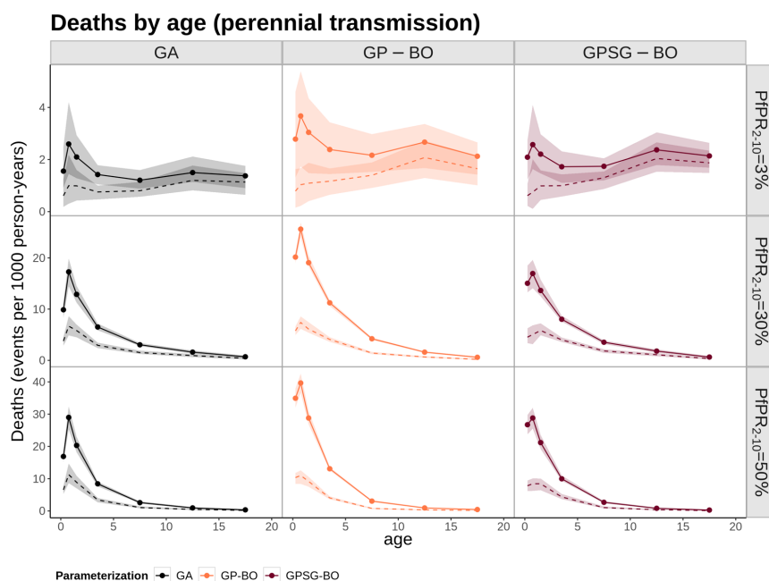
Figure S30. Yearly incidence of malaria-related deaths in a perennial transmission setting as a function of age, displayed by transmission intensity (PfPR 2-10 ) and parameterization. Malaria mortality incidence is presented in terms of the yearly number of deaths in a population of 1000 individuals. The dashed estimates represent direct malaria deaths, and the solid all malaria deaths (including those attributable to co-morbidities). The PfPR 2-10 categories include simulated prevalences of 2.5-3.5%, 9-10%, 28-32%, and 47-53% labeled as 3%, 10%, 30%, and 50%, respectively
