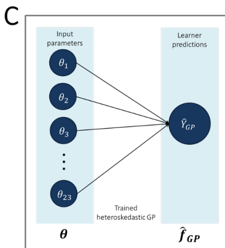
Gaussian process
