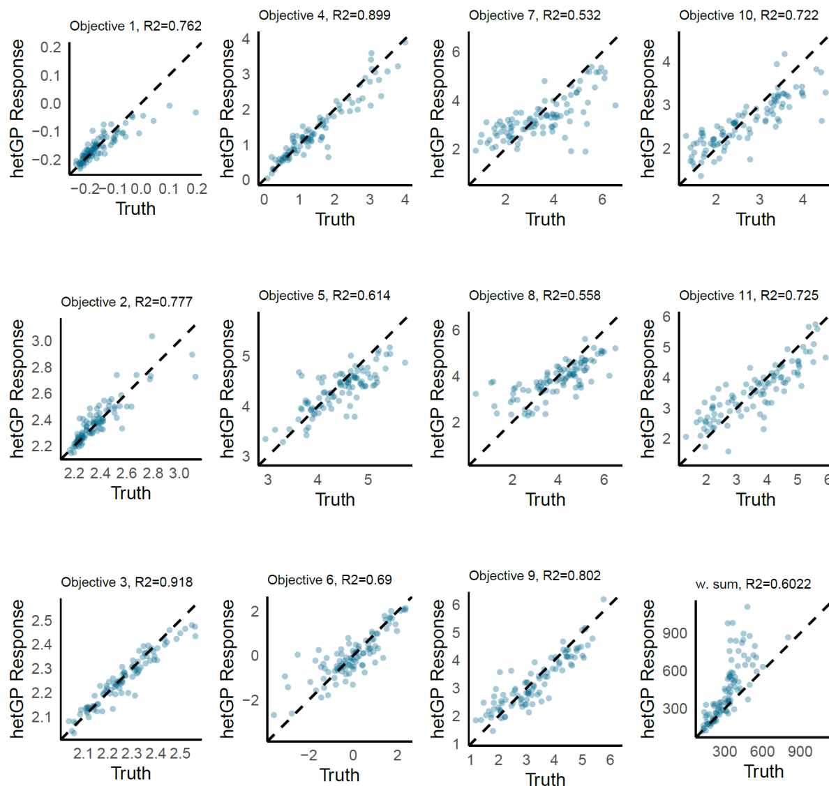
Figure S3. GP emulator performance. Emulator predictions vs true values on a holdout set compromising 10% of initial samples in iteration 30 (final iteration). w.sum is the weighted sum F , of the 11 objectives. Here, predictions are generated as the weighted sum of individual objective predictions.
