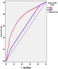
ROC Curve
