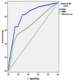
ROC Curve
