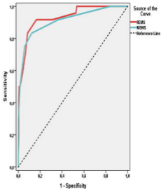
ROC Curve
