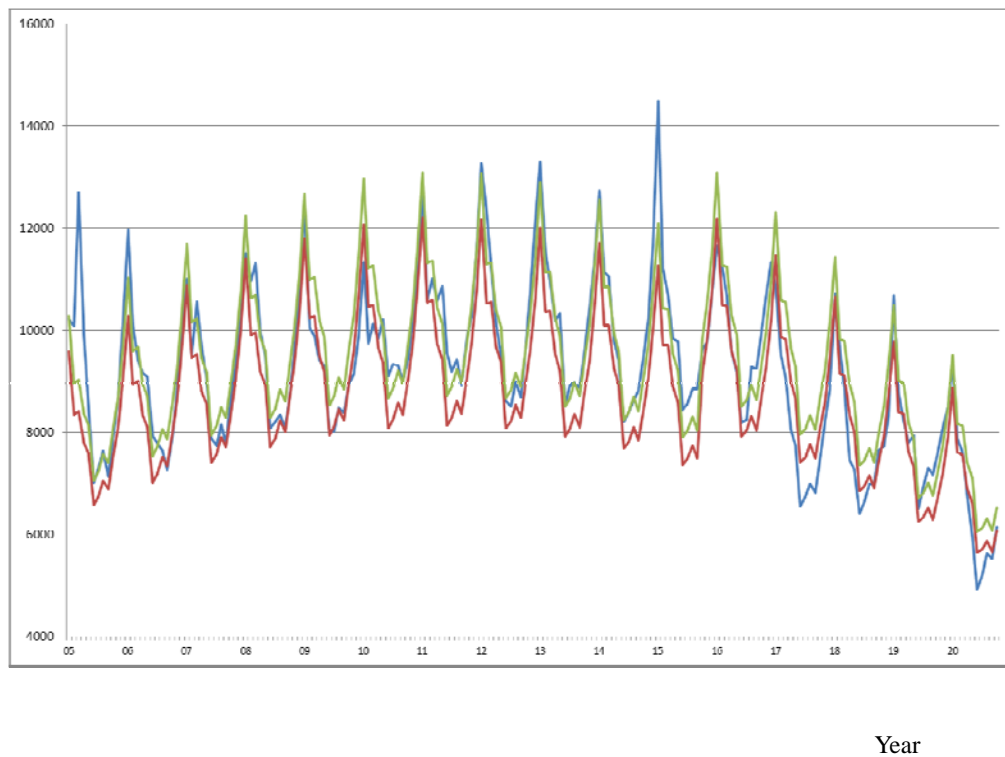
Figure 1: Observations of the estimated baseline and threshold for pneumonia deaths from 2005 through October 2020 in Japan (persons)
