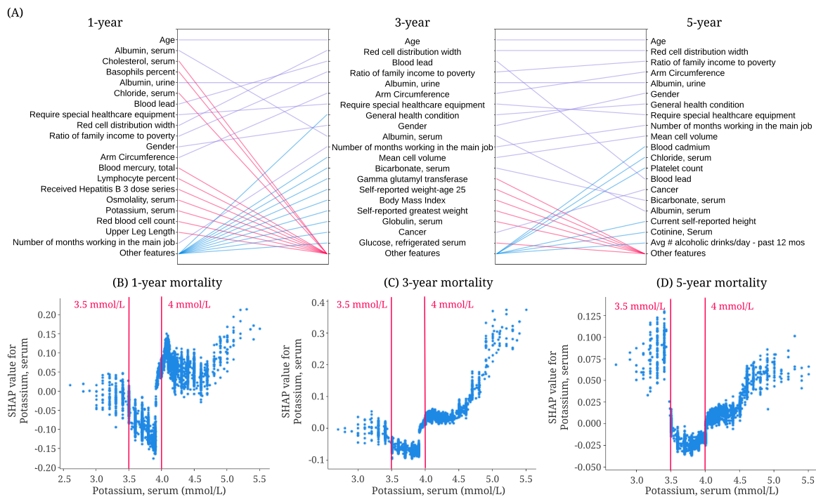
Figure 6: Identifying important discoveries for mortality prediction from tree-based models using different follow-up times (Section 3.3.1). (A) Relative importance of input features in 1-, 3-, and 5-year mortality models. For each model, the figure shows the 20 most important features on prediction (ordered by the importance). The purple line indicates that the feature is in the top 20 features of two models. Blue and red lines indicate the feature is in the top 20 features of one model, but not in the top 20 features of the other. (B) The SHAP value of serum potassium in the 1-year mortality model. (C) The SHAP value of serum potassium in the 3-year mortality model. (D) The SHAP value of serum potassium in the 5-year mortality model.
