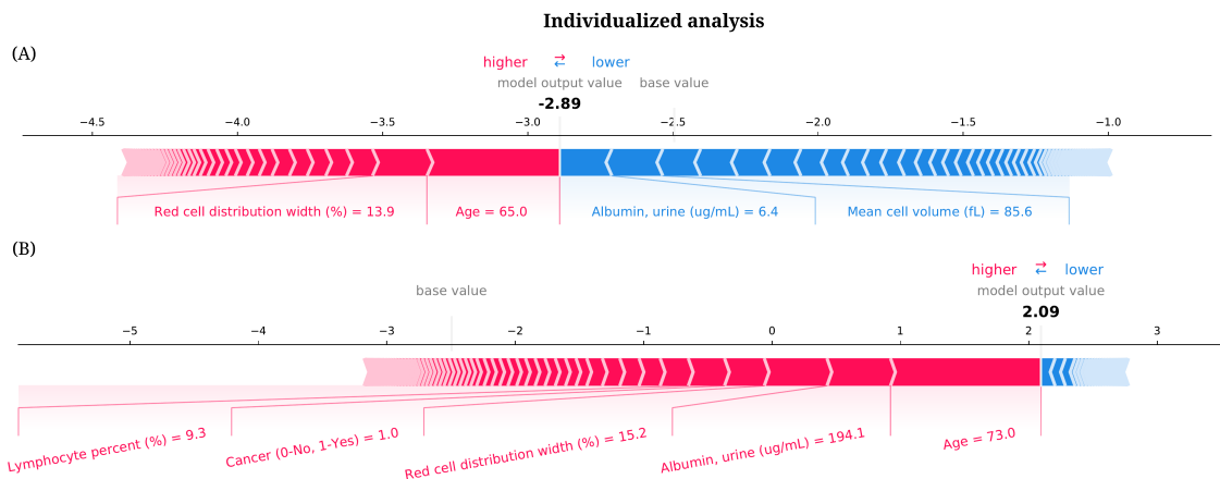
Figure 5: Combining 5-year mortality prediction gradient boosted trees models and local explanations to achieve explanation for individual samples. Tree-based mortality models can analyze individualized mortality predictions (Section 3.2.5). (A) The individualized explanation for an individual who is alive after 5 years. The output value is the prediction for that individual. The base value is the mean prediction (the value that would be predicted if we did not know any features for the current output). The features in red increase mortality risk, and those in blue decrease it. (B) The individualized explanation for a sample who is deceased after 5 years.
