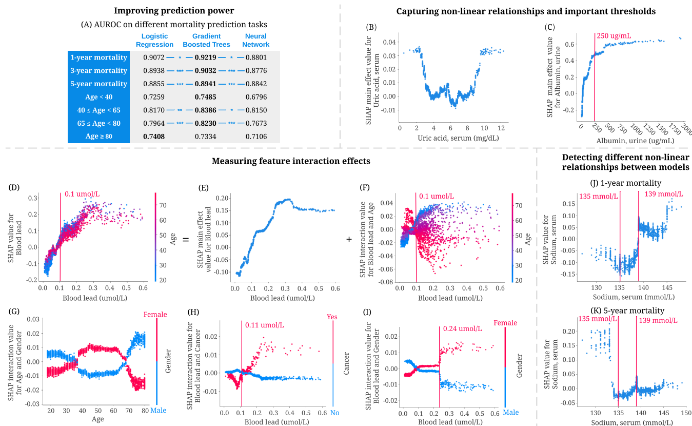
Figure 3: Advantages of tree-based models for mortality prediction. (A) The area under the ROC curve (AUROC) of gradient boosted tree models outperforms both linear models and neural networks for six of our prediction models. (Section 3.1.1). (***) represents a P-value < 0.001, (**) represents a P-value < 0.01, and (*) represents a P-value < 0.05. P values are computed using bootstrap resampling over the tested time points while measuring the difference in area between the curves. (B,C) Tree-based models can capture non-linear relationships and important thresholds (Section 3.1.3). (B) The main effect of uric acid on 5-year mortality. Higher SHAP value leads to higher mortality risk (C) The main effect of urine albumin on 5-year mortality. (D–I) Tree-based models can measure feature interaction effects (Section 3.1.4). (D) SHAP value for blood lead level in the 5-year mortality model. Each dot corresponds to an individual. (E) We can use SHAP interaction values to remove the interaction effect of age from the model and obtain the main effect of blood lead on 5-year mortality. (F) Plotting just the interaction effect of blood lead with age shows how the effect of blood lead on mortality risk varies with age. (G) The SHAP interaction value of age vs. gender in the 5-year mortality model. (H) The SHAP interaction value of blood lead vs. cancer in the 5-year mortality model. (I) The SHAP interaction value of blood lead vs. gender in 5-year mortality model. (J,K) Tree-based models can highlight different non-linear relationship between models. (Section 3.1.5) (J) The SHAP value of serum sodium in the 1-year mortality model. (K) The SHAP value of serum sodium in the 5-year mortality model.
