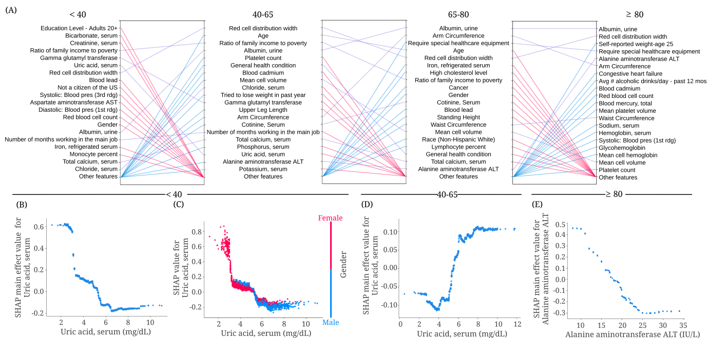
Figure 7: Identifying important discoveries for mortality prediction in different age groups (Section 3.3.2). (A) Relative importance of input features in <40, 40-65, 65-80 and \geq 80 age groups. For each model, the figure shows the 20 most impactful features on prediction (ranked from most to least important). The purple line indicates that the feature is in the top 20 features of two models. Blue and red lines indicate the feature is in the top 20 features of one model, but not in the top 20 features of the other. (B) The main effect of serum uric acid on 5-year mortality in the <40 age group. (C) The SHAP value of serum uric acid in the <40 age group 5-year mortality model. (D) The main effect of serum uric acid on 5-year mortality in the 40-65 age group. (E) The main effect of alanine aminotransferase on 5-year mortality in the \geq 80 age group.
