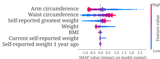
Figure 9: SHAP summary plot of the 5-year mortality prediction GBT model trained on BMI-related features.
