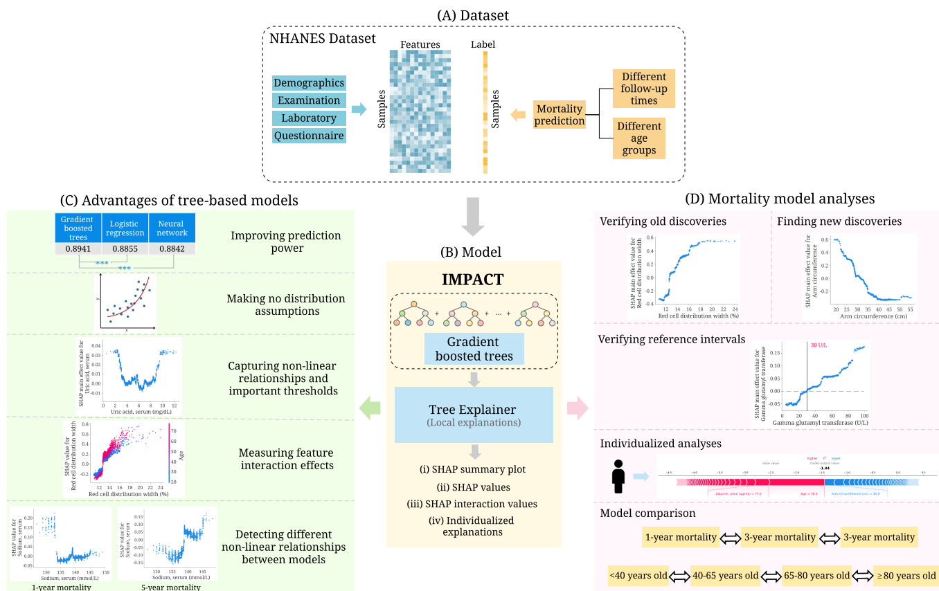
Figure 1: Overview of the IMPACT model and analyses. (A) We use the NHANES (1999-2014) dataset which includes 133 variables and 47,261 samples. The variables can be categorized into four groups: demographics, examination, laboratory and questionnaire. We train the model using different follow-up times and different age groups. (B) IMPACT combines tree-based models with an explainability method. Specifically, IMPACT (1) trains tree-based models are trained for mortality prediction using NHANES dataset (2) uses TreeExplainer to provide local explanations for our models. (C) We illustrate the advantages of interpretable tree-based model compared to traditional linear model in epidemiological studies. (D) We further analyze all mortality models and demonstrate the effectiveness of IMPACT to verify existing findings, identify new discoveries, verify reference intervals, obtain individualized explanations, and compare models using different follow-up times and age groups.
