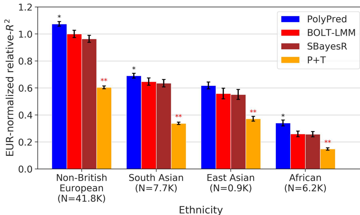
Figure 2: Trans-ethnic PRS results for real UK Biobank traits. We report average prediction accuracy (relative- R^2 ; see main text), meta-analyzed across 7 well-powered, independent traits, for PRS trained in UK Biobank British samples (average N=325K ) and applied to 4 UK Biobank target populations. Target population sample sizes are indicated in parentheses; PolyPred used 500 additional training samples from each target population to estimate mixing weights. Asterisks above each bar denote statistical significance of the difference vs. BOLT-LMM, with black asterisks denoting an advantage and red asterisks denoting a disadvantage (* P<0.05 ; ** P<0.001 ). Errors bars denote standard errors. Numerical results, results for all 49 traits analyzed, absolute prediction accuracies ( R^2 ), and P-values of relative improvements vs. BOLT-LMM are reported in Supplementary Tables 4-5.
