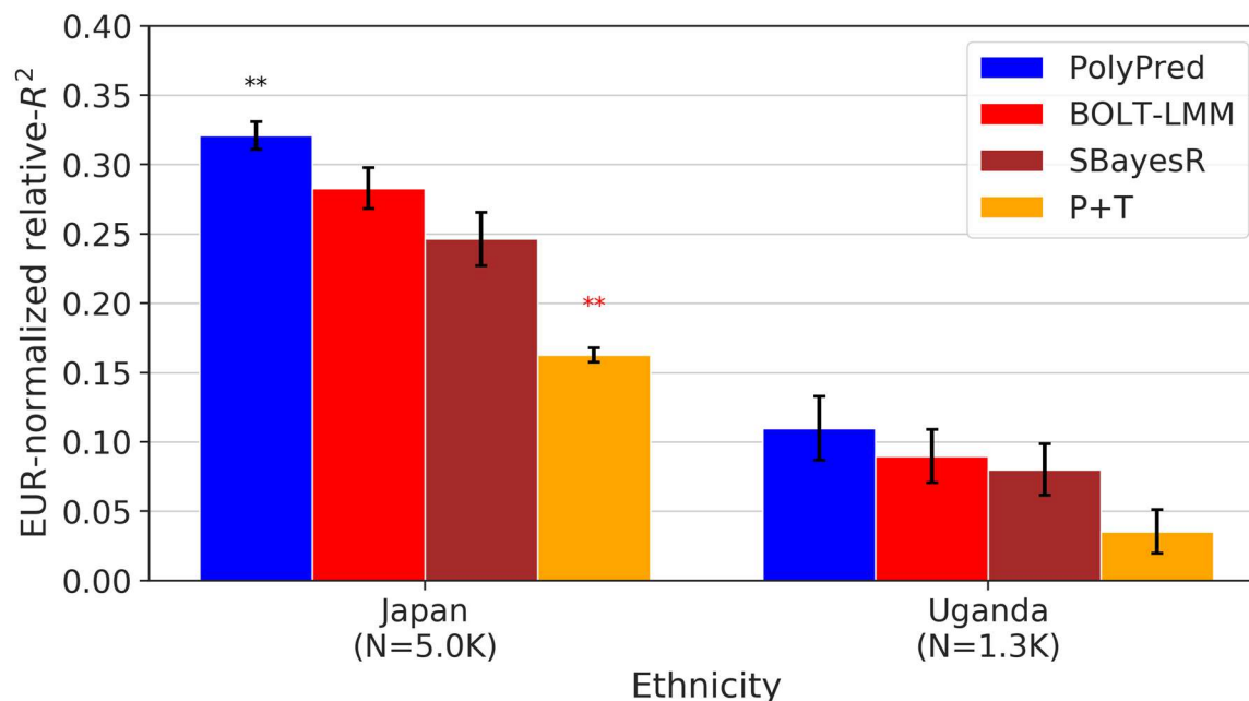
Figure 3: Trans-ethnic PRS results for Biobank Japan and Uganda-APCDR traits. We report average prediction accuracy (relative- R^2 ; see main text), meta-analyzed across 7 well-powered, independent traits, for PRS trained in UK Biobank British samples (average N=325K ) and applied to Biobank Japan and Uganda-APCDR target populations. Target population sample sizes are indicated in parentheses; PolyPred used 500 additional training samples from each target population to estimate mixing weights. Asterisks above each bar denote statistical significance of the difference vs. BOLT-LMM, with black asterisks denoting an advantage and red asterisks denoting a disadvantage (* P<0.05 ; ** P<0.001 ). Errors bars denote standard errors. Numerical results, results for all 23 traits analyzed, absolute prediction accuracies ( R^2 ), and P-values of relative improvements vs. BOLT-LMM are reported in Supplementary Table 7.
