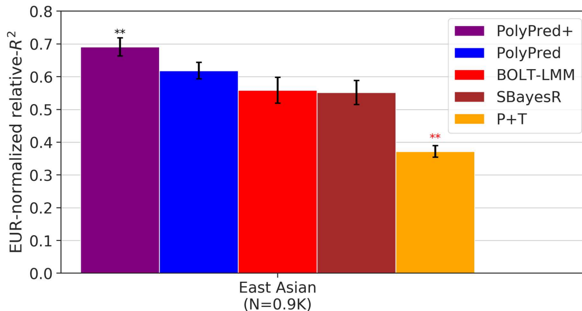
Figure 4: Trans-ethnic PRS results for UK Biobank East Asians using PolyPred+. We report average prediction accuracy (relative- R^2 ; see main text), meta-analyzed across 7 well-powered, independent traits, for PRS trained in UK Biobank British (average N=325K ) and Biobank Japan samples (average N=124K ; used by PolyPred+ only) and applied to UK Biobank East Asians. The target population sample size is indicated in parentheses; PolyPred and PolyPred+ used 500 additional training samples from the target population to estimate mixing weights. Asterisks above each bar denote statistical significance of the difference vs. BOLT-LMM, with black asterisks denoting an advantage and red asterisks denoting a disadvantage ( *P<0.05 ; **P<0.001 ). Errors bars denote standard errors. Numerical results, results for all 23 traits analyzed, absolute prediction accuracies ( R^2 ), and P-values of relative improvements vs. BOLT-LMM are reported in Supplementary Table 4.
