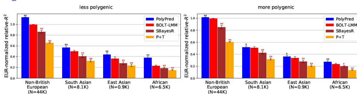
Figure 1: Trans-ethnic PRS results for simulated UK Biobank traits. We report average prediction accuracy (relative- R^2 ; see main text) for PRS trained in UK Biobank British samples ( N=337K ) and applied to 4 UK Biobank target populations across 100 simulated traits with less polygenic (0.1% of SNPs causal; left panel) or more polygenic (0.3% of SNPs causal; right panel) architectures. Target population sample sizes are indicated in parentheses; PolyPred used 500 additional training samples from each target population to estimate mixing weights. Asterisks above each bar denote statistical significance of the difference vs. BOLT-LMM, with black asterisks denoting an advantage and red asterisks denoting a disadvantage (* P<0.05 ; ** P<0.001 ). Errors bars denote standard errors. Numerical results, absolute prediction accuracies ( R^2 ), and P-values of relative improvements vs. BOLT-LMM are reported in Supplementary Table 1.
