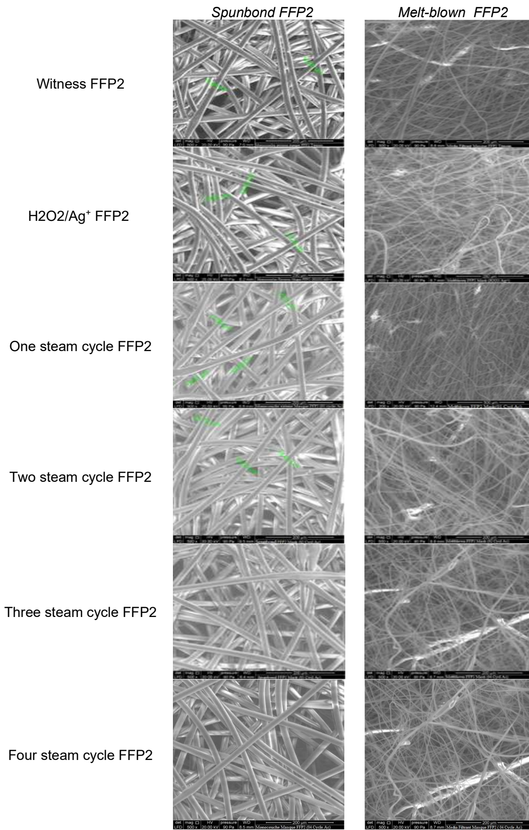
Figure 1- SEM images of the Melt-blown and Spunbond composing FFP2 masks per reprocessing cycle.
