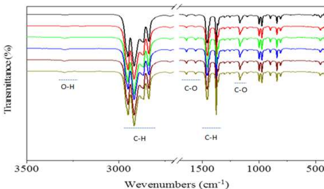
Figure II- FTIR Spectra of the Melt-blown layers composing FFP2 masks per reprocessing cycle
