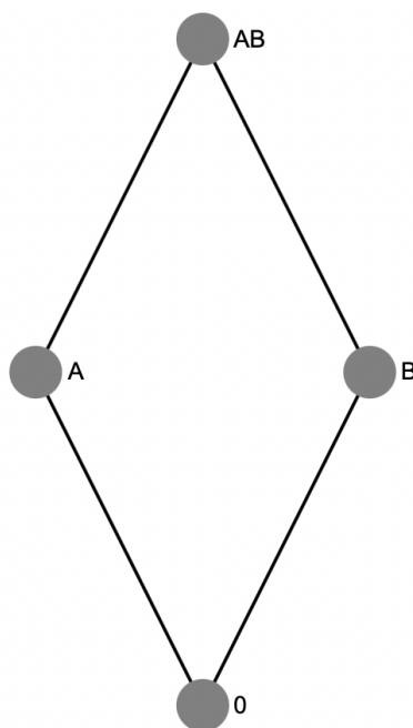
Figure 1: Hasse diagram of lattice model with 2 subjects, A and B
