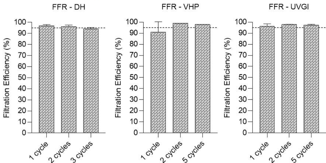
Figure 4. Filtering facepiece respirator (FFR) NaCl filtration efficiency- and surgical mask (SM) bacterial filtration efficiency (BFE) testing after single-cycle or multiple-cycle decontamination using dry heat (DH), vaporised hydrogen peroxide (VHP), and ultraviolet germicidal irradiation (UVGI). Horizontal dashed lines represent the NaCl filtration efficiency requirement of \geq 95\% according to NIOSH 42 CFR Part 84. Untreated FFRs ( n=3 ) surpassed the minimum NaCl filtration efficiency, achieving 97.01% ( \pm 0.56 ) as a baseline before treatment. Horizontal dotted lines represent the bacterial filtration efficiency (3 \mu m droplet size) requirement of \geq 98\% according to EN 14683 for Type II and ASTM F2100 for Level 2 SMs. Untreated SMs ( n=3 ) surpassed the minimum BFE, achieving 99.50% ( \pm 0.08 ) as a baseline before treatment.
