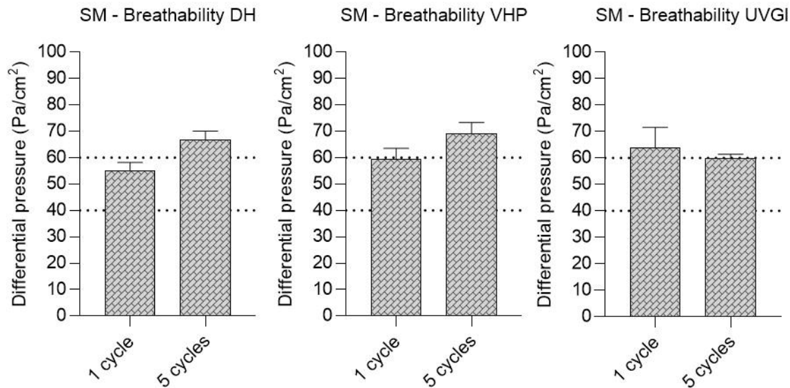
Figure 5. Surgical mask (SM) breathability testing after single-cycle or multiple-cycle decontamination using dry heat (DH), vaporised hydrogen peroxide (VHP), and ultraviolet germicidal irradiation (UVGI). Horizontal dotted lines represent the maximum allowed differential pressure in following standards: < 40 \text{ Pa/cm}^2 according to EN 14683:2019 Annex C for Type I and II masks and < 60 \text{ Pa/cm}^2 for Type IIR. Untreated SMs ( n=5 ) achieved 52.08 (\pm 0.99) \text{ Pa/cm}^2 differential pressure as a baseline before treatment.
