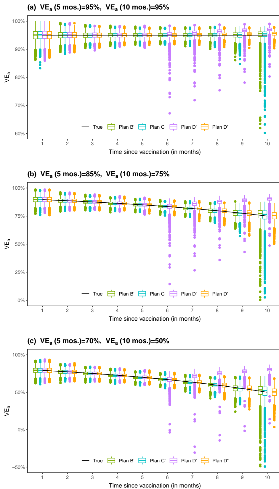
Figure 3. Proposed estimates of VE_a under four unblinded crossover plans.
