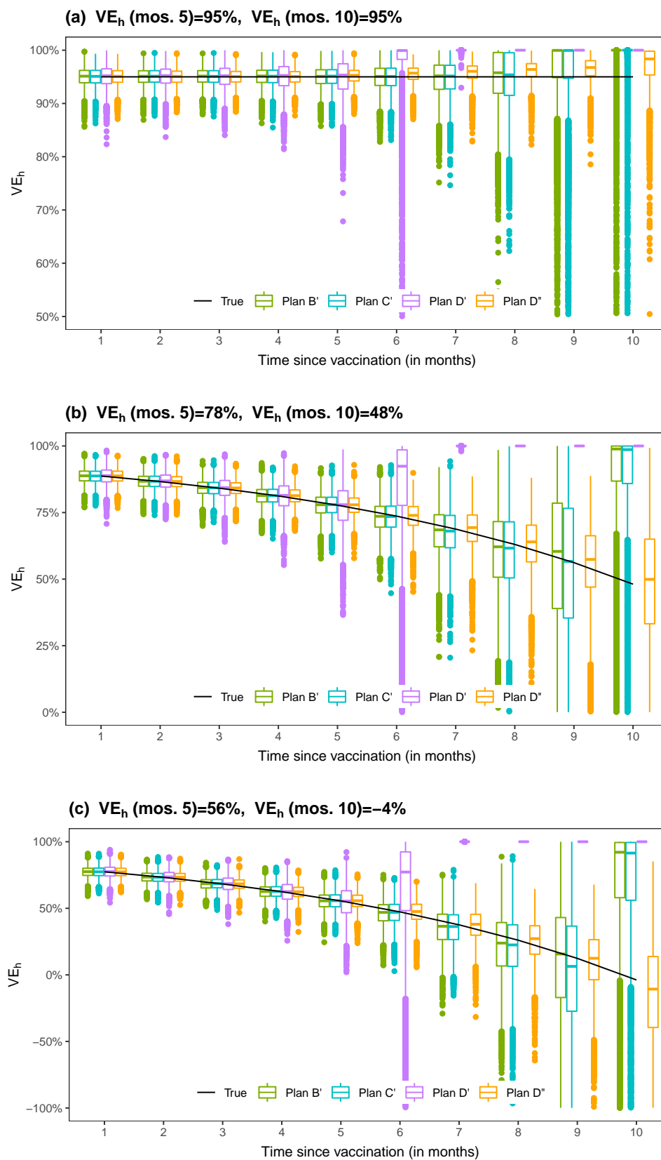
Figure 5. Proposed estimates of VE_h under four unblinded crossover plans.
