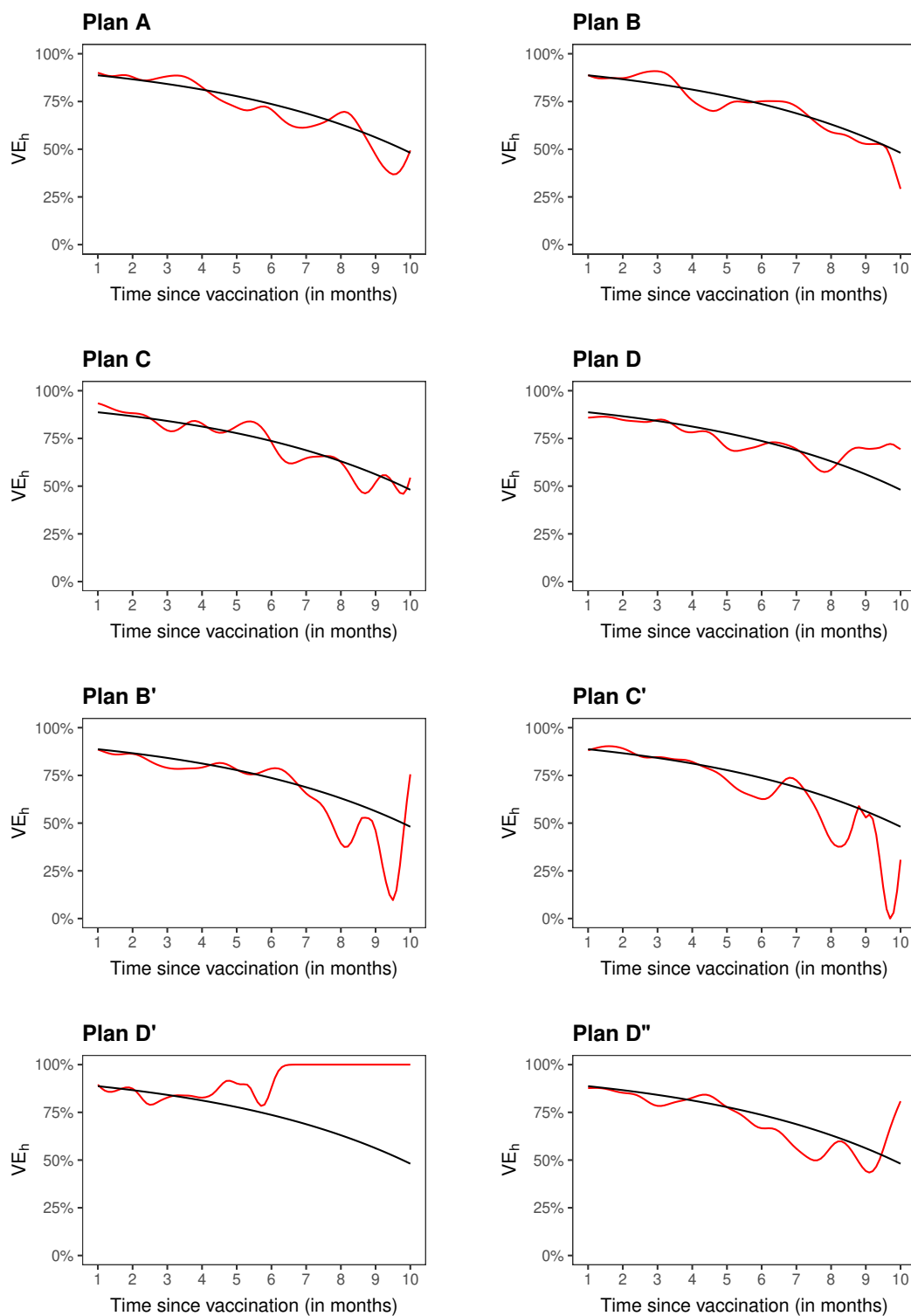
Figure 7. Estimation of VE_h a clinical trial with no crossover (A), three blinded crossover (B–D), and four unblinded crossover (B’–D’): the black curve pertains to the true value, and the red curve to the proposed estimate.
