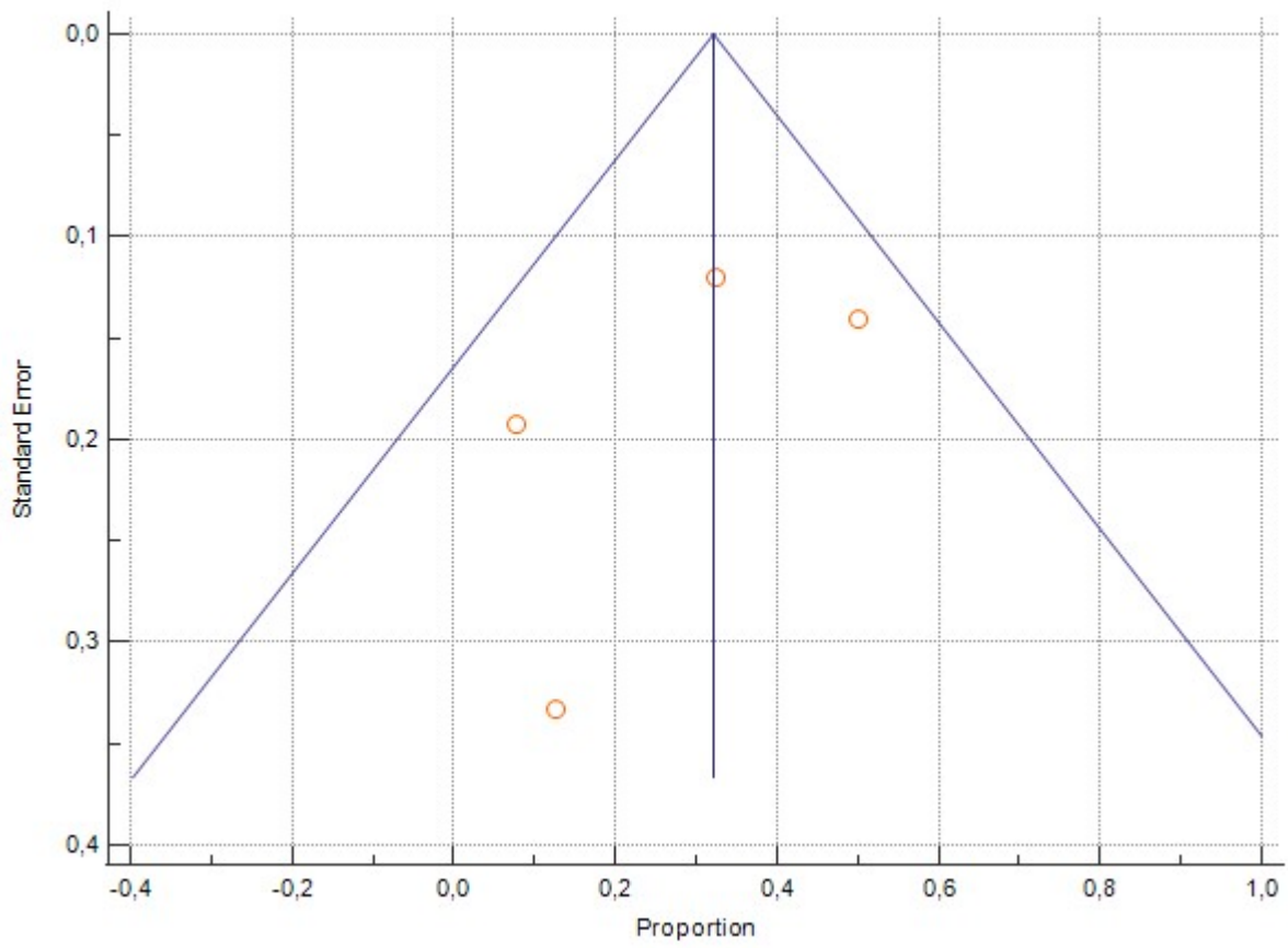
Figure 3. Funnel plot showing no apparent asymmetry.
