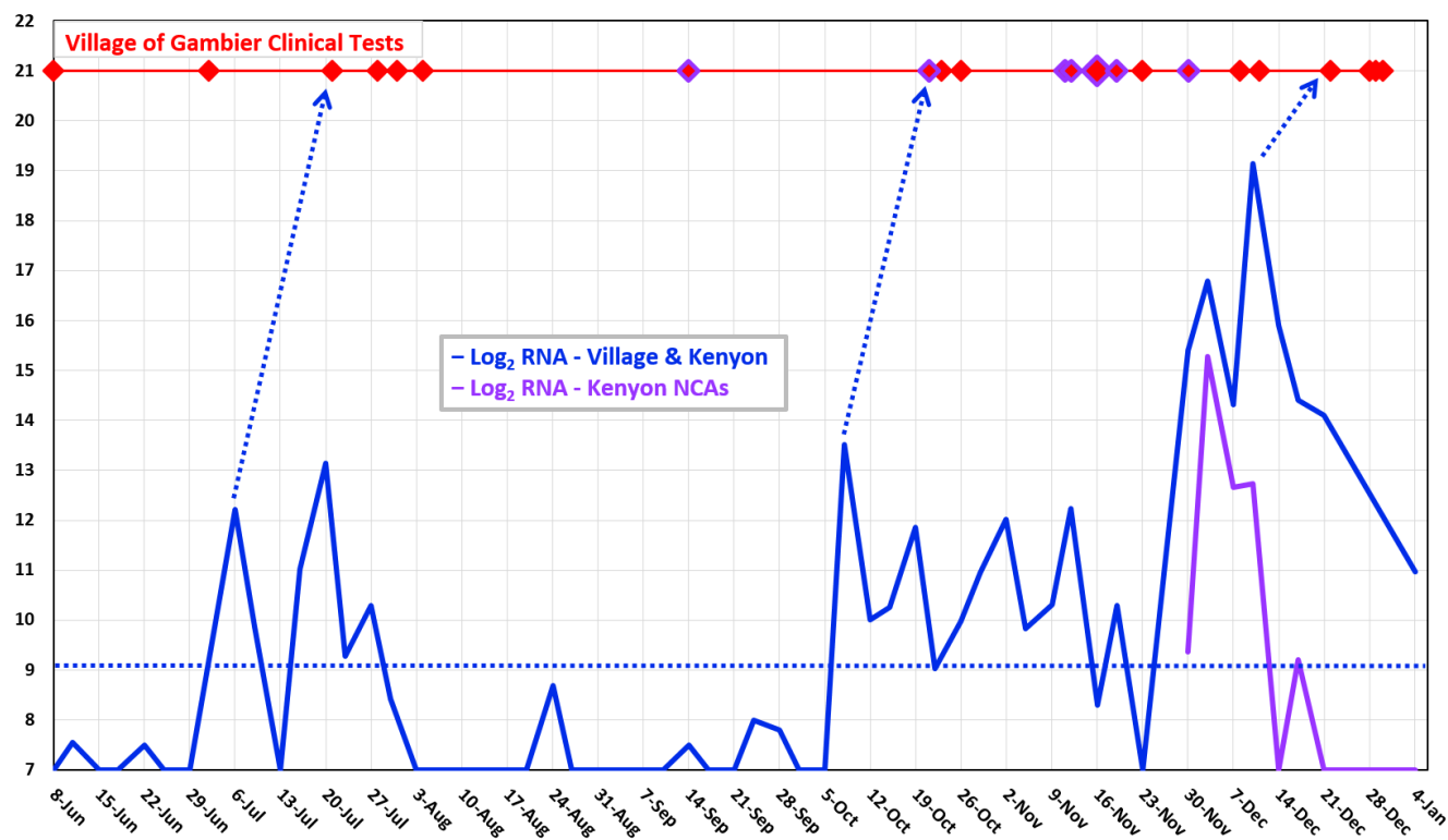
Figure 1. Wastewater SARS-CoV-2 RNA counts tracked with clinical testing.
