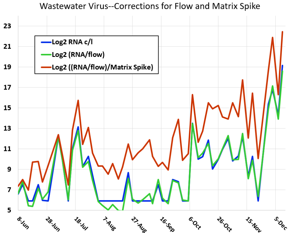
Figure 3. Wastewater signal correction factors.
