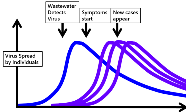
Figure 2. Model for relationship between wastewater SARS CoV-2 signal and COVID-19 infections. The wastewater RNA concentration starts to rise several days before symptoms occur. The first case may however be asymptomatic. Secondary infections occur early, becoming evident much later.
