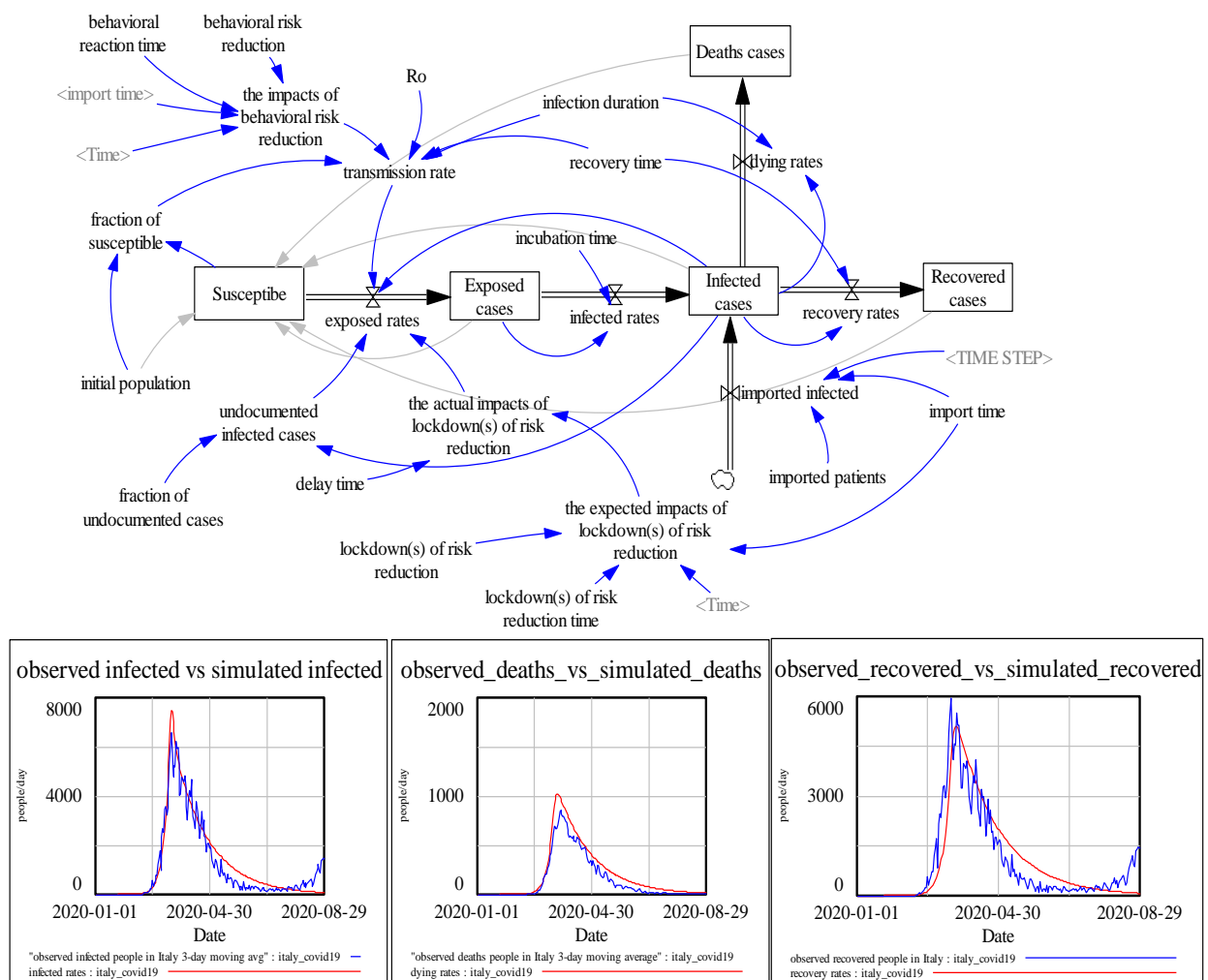
Figure 1. The SIER model for Italy
