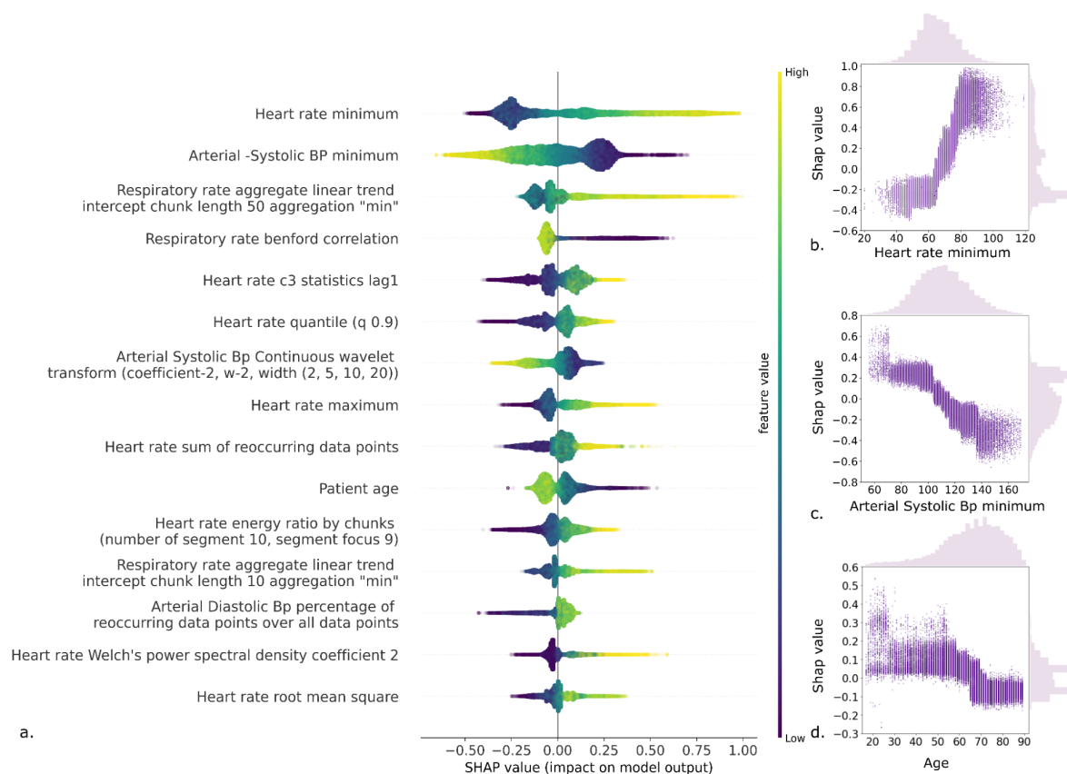
Figure3 a.) SHAP values of top 15 hand-engineered time-series features (descending order) derived from the five-fold test set on eICU data. The Violin plot shows the distribution of SHAP values. The color map represents the feature value from low to high b.) A scatter plot of Heart rate minimum and corresponding SHAP values, showing a positive correlation between the two. c.) A scatter plot of Arterial Systolic Blood pressure minimum and corresponding SHAP values, showing negative correlation d.) A scatter plot of Patient age and corresponding SHAP values, showing a negative correlation.
