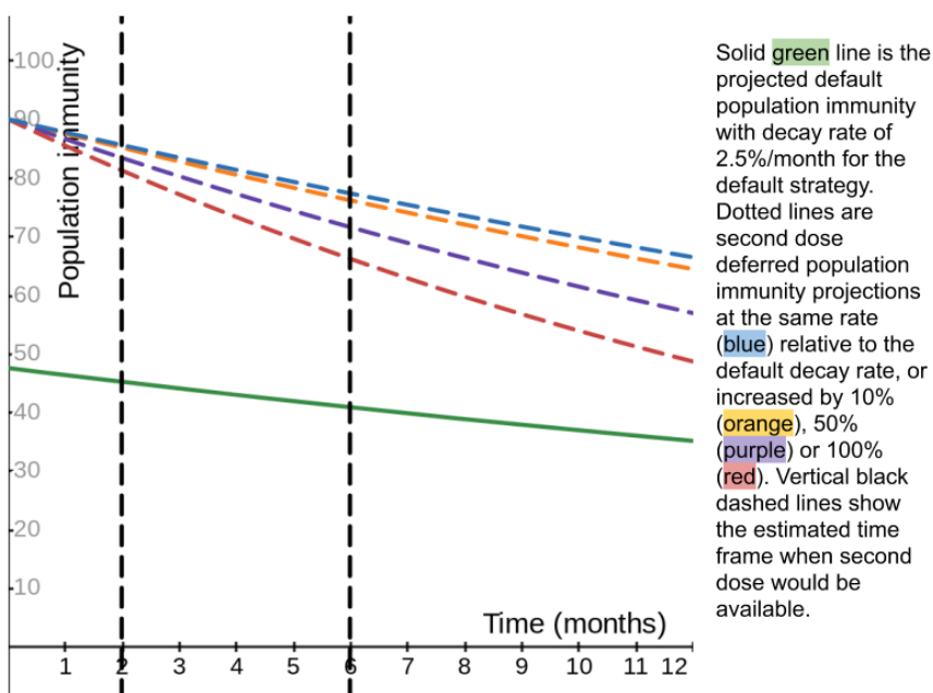
Image 5: Evaluating varying decay rates of one dose efficacy relative to the default decay rate: The decay rate is set at 2.5% for the two dose regimen. The decay rate for one dose efficacy ranges from the same decay rate to the 2 dose regimen. Even with a decay rate increased 100% compared to the default regimen, the second dose deferral strategy clearly increases the population immunity.
