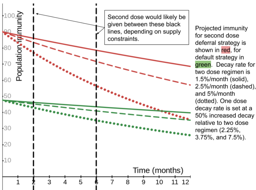
Image 4: Evaluating varying decay rates of default strategy: The second dose deferral strategy (red) shows clear benefit to population immunity relative to the default regimen (green) with the default regimen decay rates varying from 1.5%/month to 5%/month and the relative increase in decay rate for one dose efficacy being set at 50% higher. The same type of line (solid, dashed or dotted) should be compared between the two strategies. Realistic time frames until a
