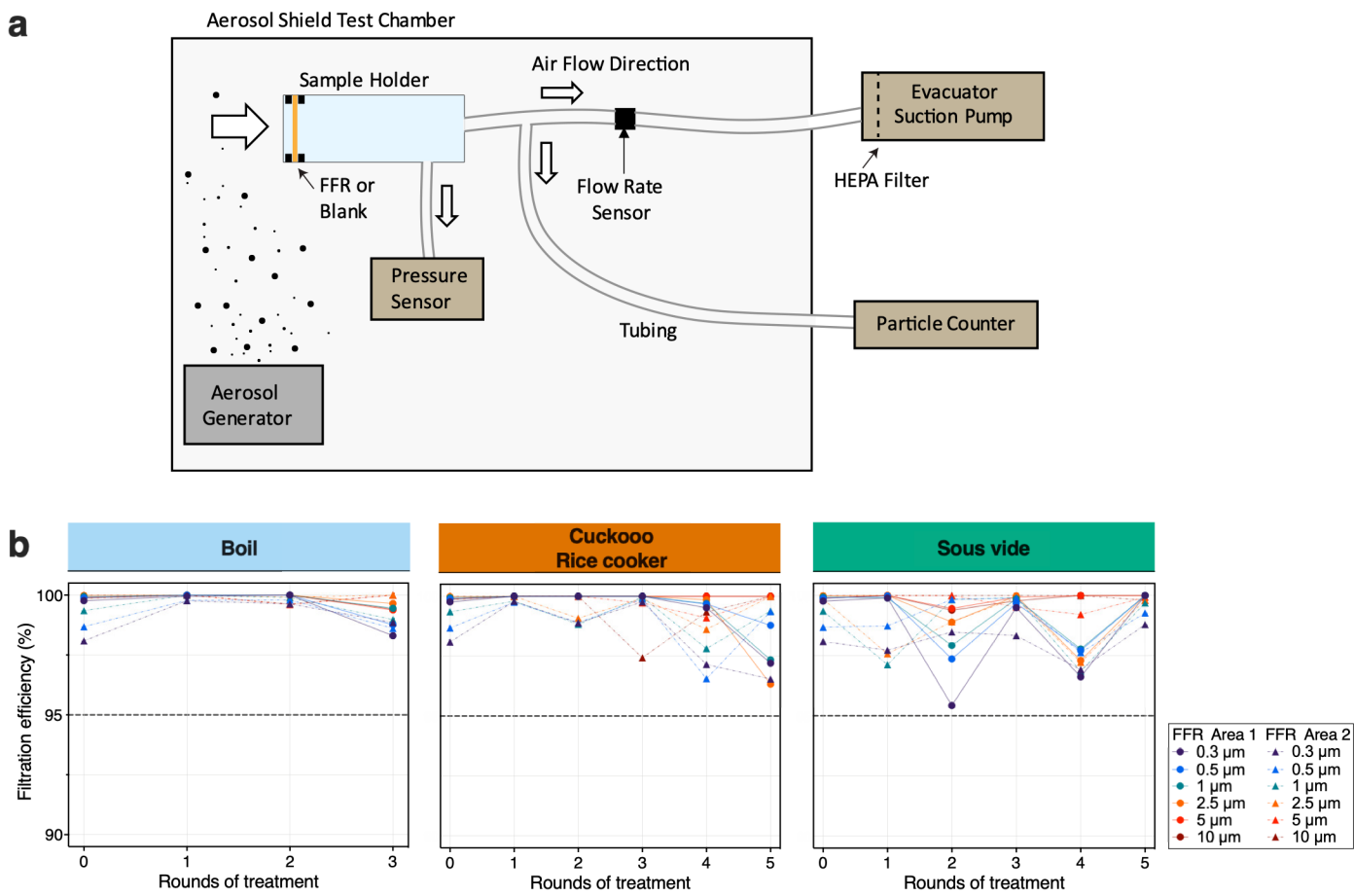
Fig 4. Filtration efficiency for control and heat-treated Halyard Fluidshield 3 FFRs.
