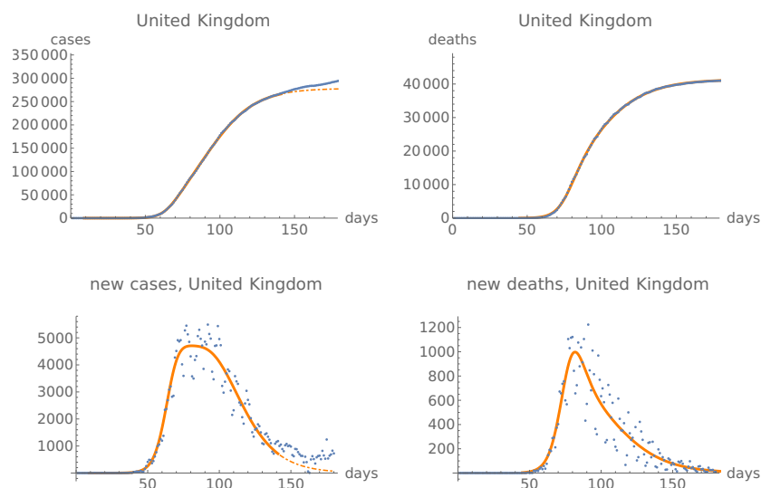
Figure 2: Same as the last two lines of Figure 1 for the United Kingdom.
