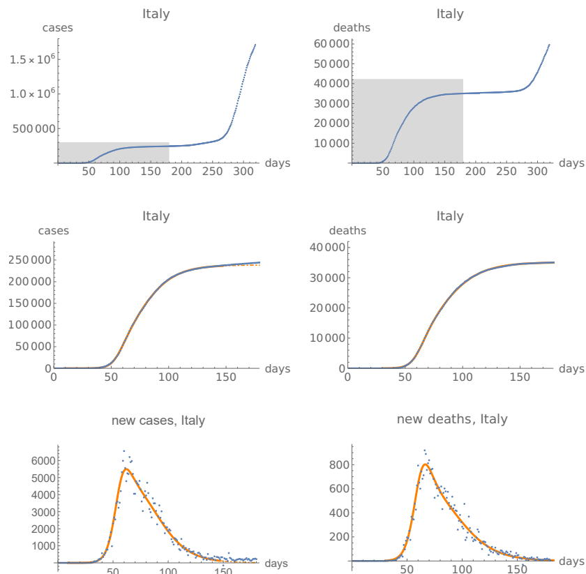
Figure 1: Fits of the function I to the first phase of the Covid-19 pandemic in Italy. First line: the cumulative cases time-series and death time-series up to December 6, 2020. The second line is a zoom to the shaded windows in the first line, where moreover the fits of the function I , are shown. The continuous orange curve showing the fit to the curve of accumulated cases becomes dashed on day 148 (June 16, 2020), on which the fit starts deviating from the data; we interpret this as the end of the first phase of the epidemic. Third line: Daily infections and deaths, together with the derivative of the function I . Note the different scales on all plots.
