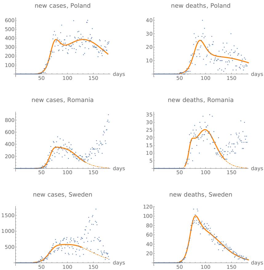
Figure 3: Time series for Poland, Romania and Sweden, with the derivative of the best fit of the function I indicated in orange. The orange lines become dashed on the day at which the fit of the function I to the data is optimal, when compared to fits with different lengths, indicating the start of a new phase of the epidemic. The lack of a clear peak, as well as the width of the region where the numbers of daily new infections are high before starting to decline, explain the difference seen in Table 1 between the lags as determined from the function I and from the integral method.
