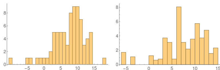
Figure 8: The histograms of the lags between days of the maximum number of casualties and the maximum number of daily infections for the first wave of Covid-19, as determined by the “average-data-integral” method. The first histogram is direct, the second is obtained by weighting the data inversely proportionally to the width of the peak.
