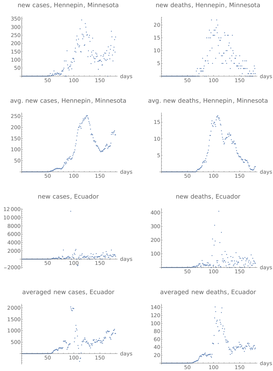
Figure 9: Time series for the outliers in the histogram of Figure 8, namely Hennepin, Minnesota and Ecuador.
