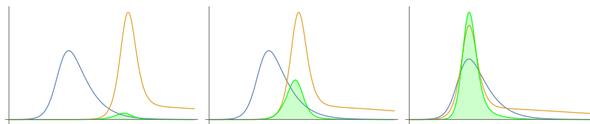
Figure 6: Illustration of the integral overlap method: Consider the blue and orange functions in the left plot. The green function is their product, and the shaded area under the green curve is the integral equivalent of the value f(0) of the function f of (2). In the middle plot the orange function has been shifted to the left by some value r , leading to an increased area, equal to f(r) , under the new product curve. The area under the graph of the product function is maximised by shifting the orange function as shown in the right plot.
