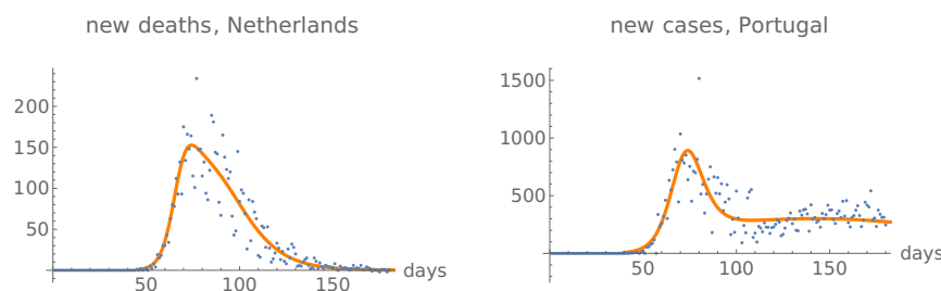
Figure 7: Daily death time-series for Netherlands and daily infections time-series for Portugal, with the derivative of the best fit of the function I indicated in orange.
