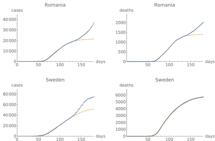
Figure 5: Fits of the function I to the first phase of the Covid-19 pandemic for Romania and Sweden. A clear transition from one phase of the epidemic to another for Romania can be seen in Figure 3, which is perhaps less clear on the plots here. Similarly a clear transition to a second phase for the death time-series of Sweden can be seen in Figure 3, but less so in the cases time-series of Sweden, or in the plots here. We draw attention to different scales on different plots.
