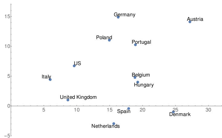
Figure 4: Lag between days of the maximum number of casualties and the maximum number of daily infections for the first wave of Covid-19 determined from the function I , ordered with decreasing quality of the fits to the function I . Romania and Sweden have not been included in the plot, because of the width of the error interval when calculated by the integral overlap method.
