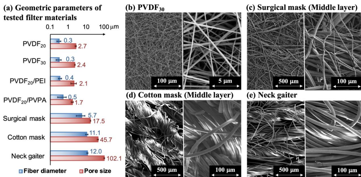
Figure 1 (a) Geometric parameters of tested filter materials, and SEM of (b) PVDF 30 , (c) surgical mask middle layer, (d) cotton mask middle layer, and (e) neck gaiter.
