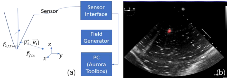
130 131 Figure 3. (a) Illustration of Pivot Calibration Using NDI Aurora EM Tracking System. (b) Mapped Location 132 of Catheter Tip in 2D Echocardiography. 133
