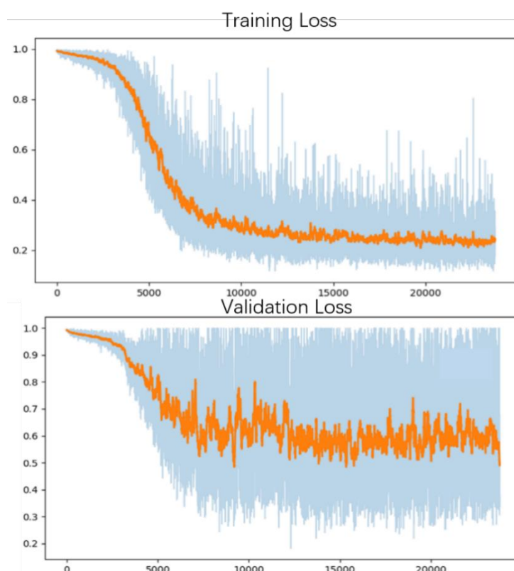
Figure 8. Training curve of the deep learning model's training and validation loss.
