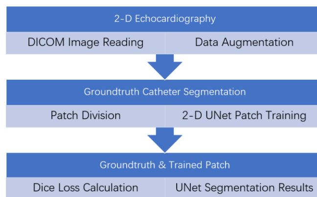
Figure 5. Flow chart of Echocardiography UNet Model Training Procedure.
