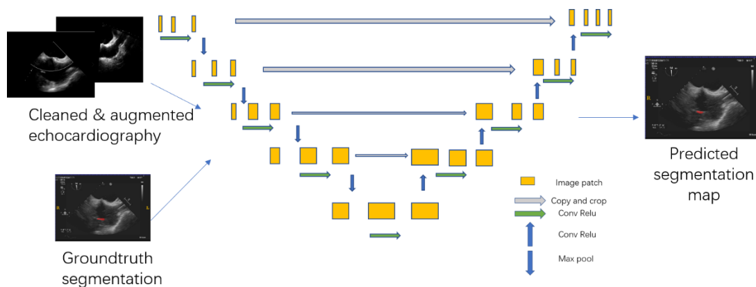
Figure 4. Diagram of Deep Learning Model Trained on 2-D Echocardiography Dataset.
