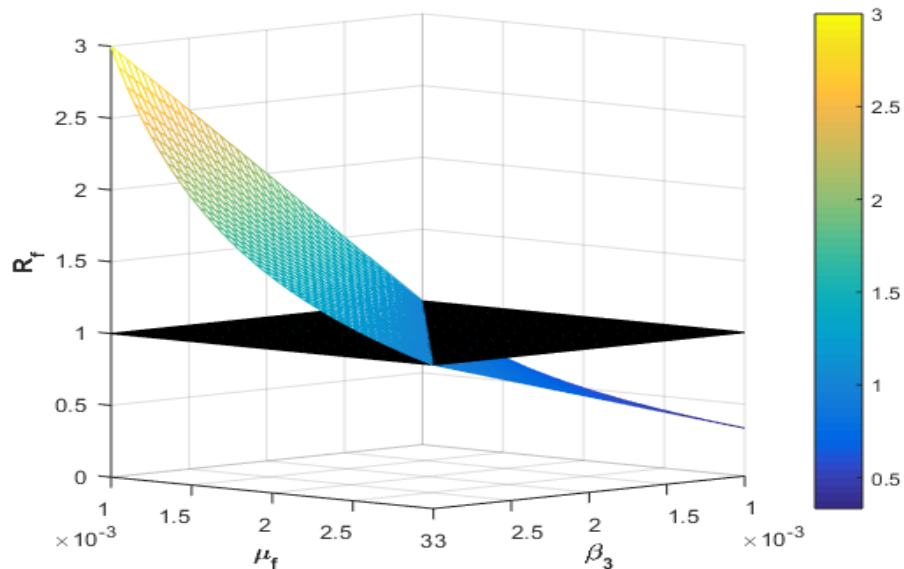
Figure 7: Effects of \beta_3 and \mu_f on the contamination food constant ( \mathcal{R}_f ).
