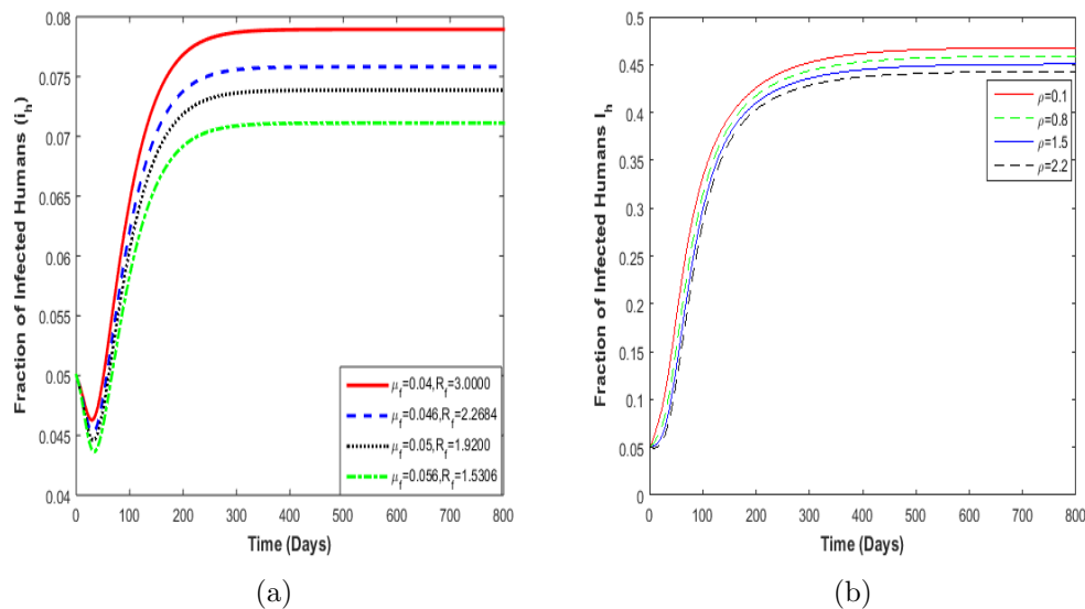
Figure 8: (a) Effects varying removal of contaminated food products ( \mu_f ) on the fraction of infected humans. (b) Effects varying the rate of non-aware susceptible becomes aware susceptible ( \tilde{\rho} ) on the fraction of infected humans. The value for the \mathcal{R}_f is 1.5306.
