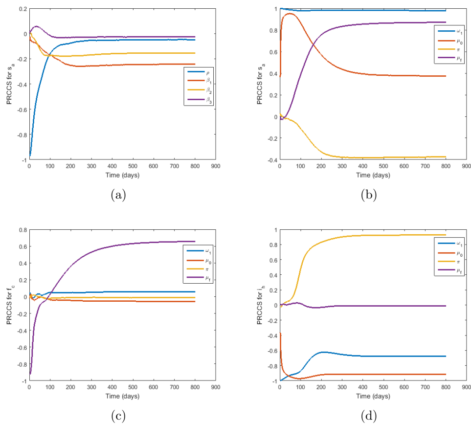
Figure 3: Partial correlation coefficients of parameters \pi, \mu_0, \tilde{\rho}, \omega_1, \beta_1, \beta_2, \beta_3 and \mu_f over time for state variables s_a, f_c and i_h respectively. Note that, \rho in the legend represents \tilde{\rho} due to Matlab do not compile tilda.
