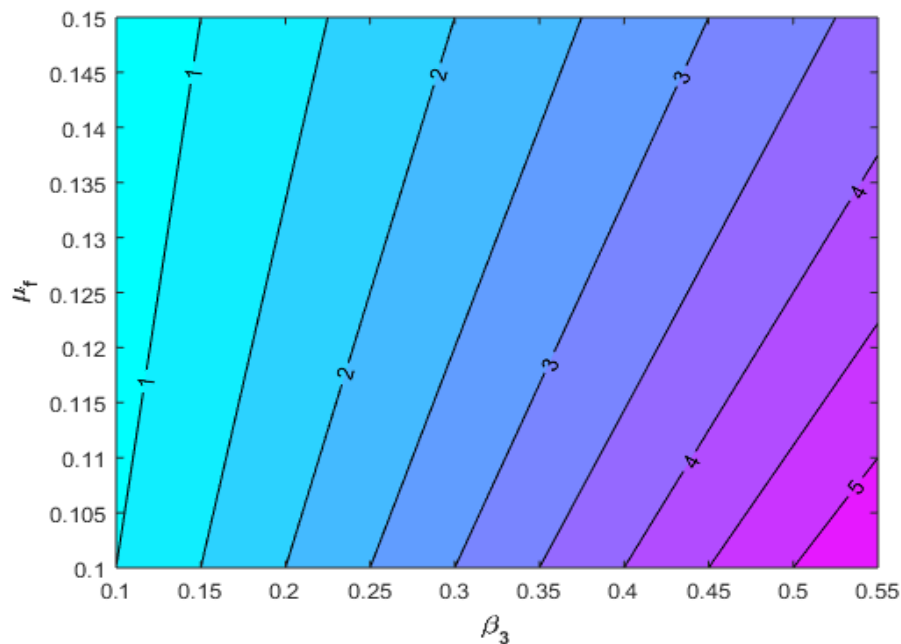
Figure 6: Contour plot of contaminated food generation number ( \mathcal{R}_f ) as a function of \beta_3 and \mu_f .
