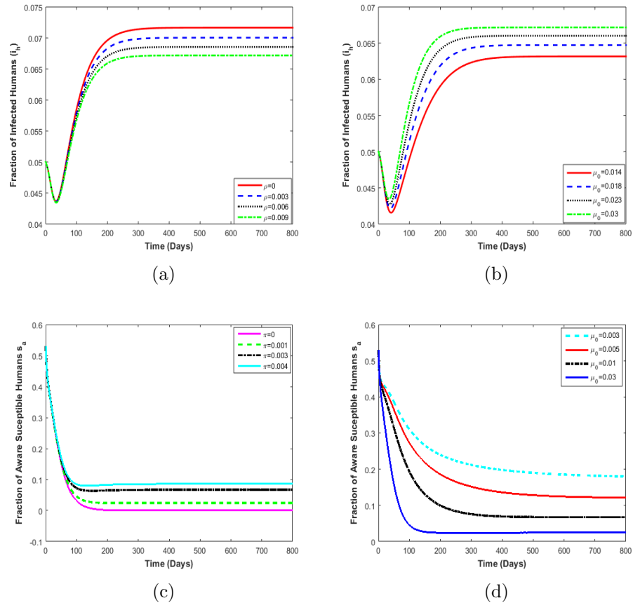
Figure 5: (a) Effects of implementing of media campaigns ( \pi ) on the fraction of infected humans. (b) Effects of depletion of media campaigns ( \mu_0 ) on the fraction of infected humans. (c) Effects of implementation of media campaigns ( \pi ) on the fraction of aware susceptible humans. (d) Effects of depletion of media campaigns ( \mu_0 ) on the fraction of aware susceptible humans.
