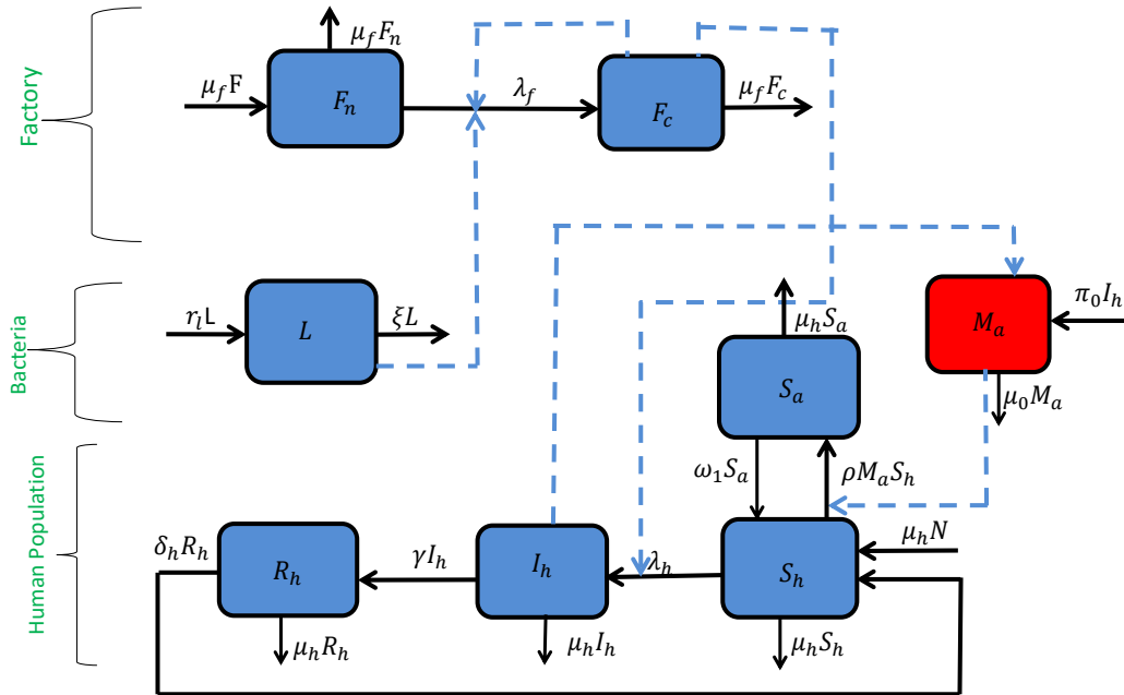
Figure 1: Shows the model flow diagram. The solid arrows represent the transitions between the compartments while the dotted lines represent the influences on the solid arrows and the compartments.
