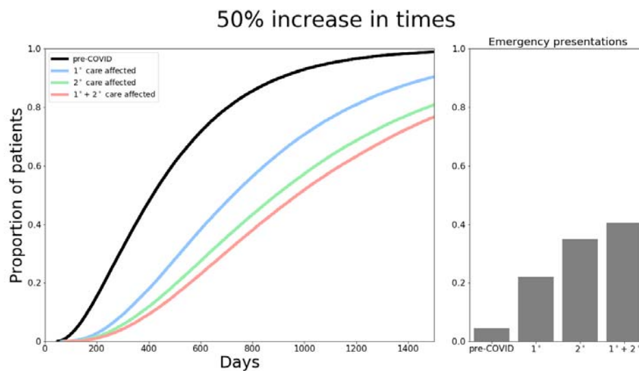
Figure 3 - Total time from symptom onset to diagnosis and proportion of emergency presentations if primary, secondary and both care services are increased by 50%.
