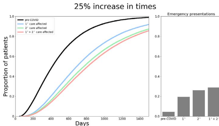
Figure 2 - Total time from symptom onset to diagnosis and proportion of emergency presentations if primary, secondary and both care services are increased by 25%.
