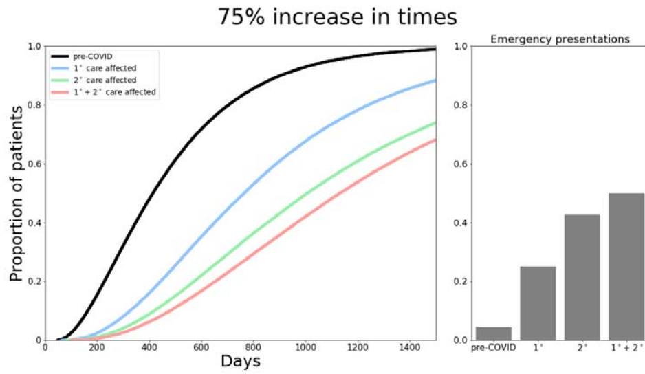
Figure 4 - Total time from symptom onset to diagnosis and proportion of emergency presentations if primary, secondary and both care services are increased by 75%.
