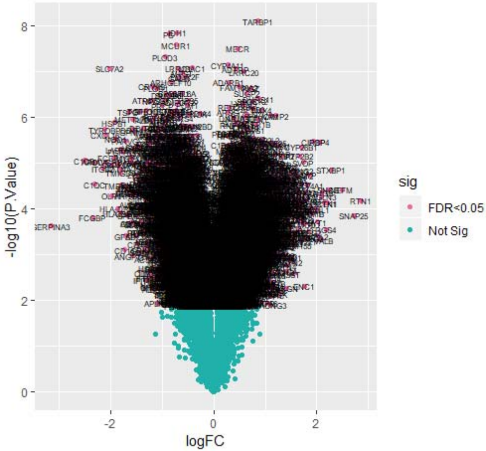
Fig. 2. Volcano plot of differentially expressed genes. Genes with a significant change of more than two-fold were selected.
