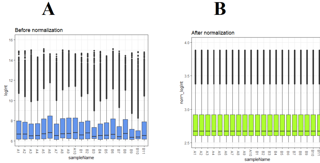
Fig. 1. Box plots of the gene expression data before normalization (A) and after normalization (B). Horizontal axis represents the sample symbol and the vertical axis represents the gene expression values. The black line in the box plot represents the median value of gene expression. (A1, A2, A3, A4, A5, A6, A7, A8, A9, A10 = normal controls samples; B1, B2, B3, B4, B5, B6, B7, B8, B9, B10 = sCJD samples)
