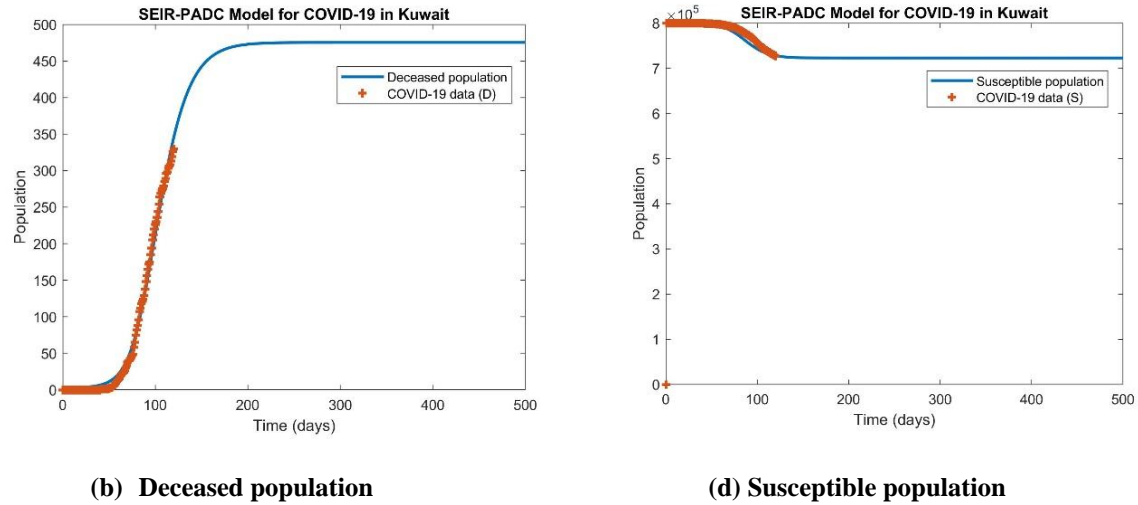
Figure 2: Fitting 4 set of COVID-19 data simultaneously with SEIR-PADC model for dynamics of COVID-19 in Kuwait (23 June 2020).
