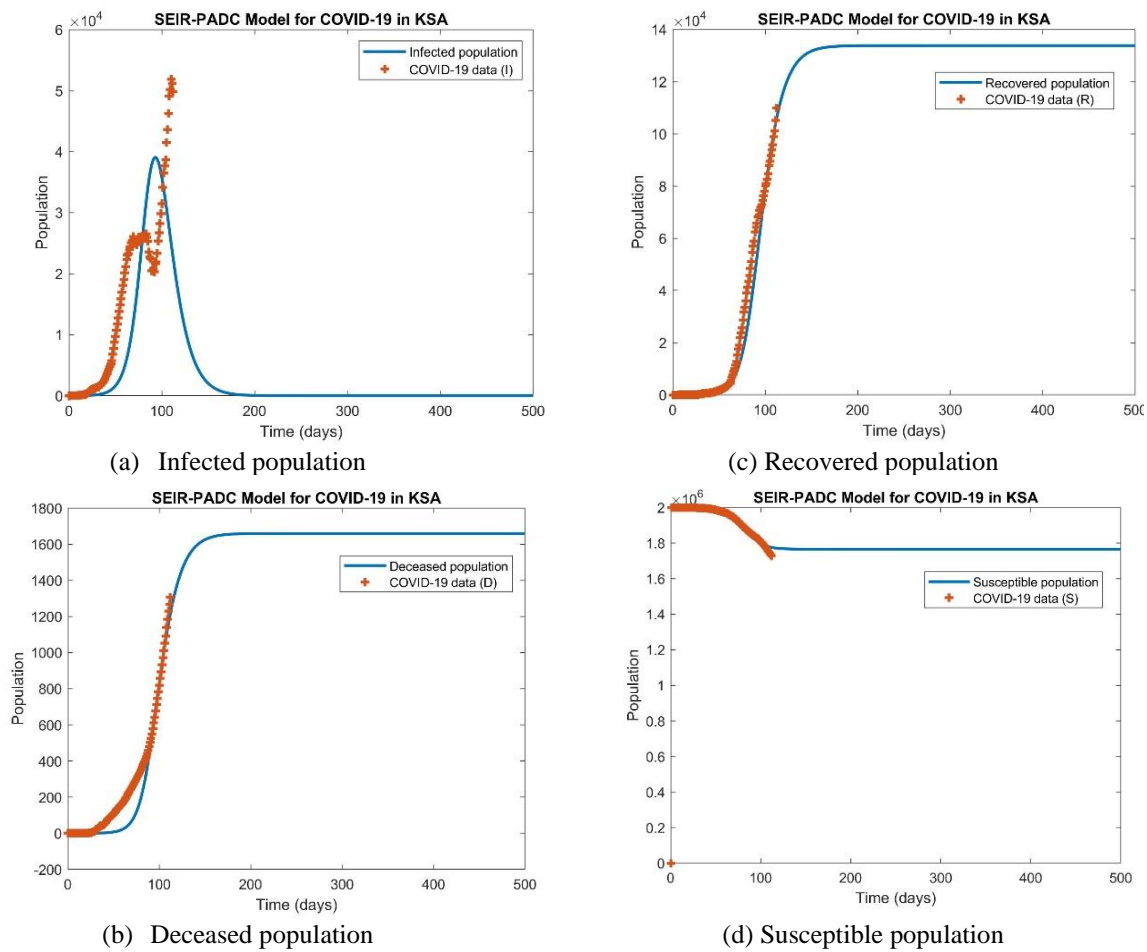
Figure 6: Fitting 4 set of COVID-19 data simultaneously with SEIR-PADC model for dynamics of COVID-19 in KSA (23 June 2020).
