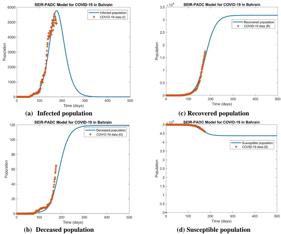
Figure 3: Fitting 4 set of COVID-19 data simultaneously with SEIR-PADC model for dynamics of COVID-19 in Bahrain (23 June 2020).
