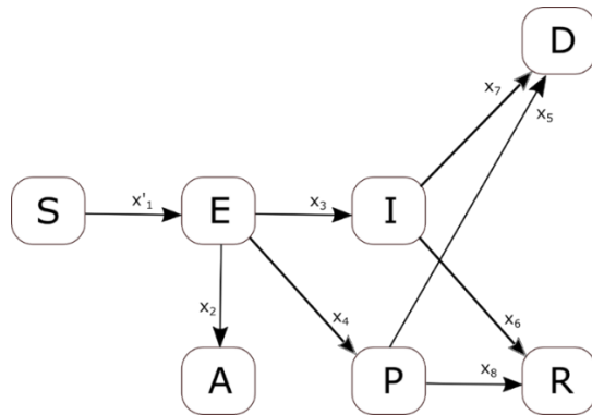
Figure 1: Flow chart of SEIR-PADC dynamic model.
