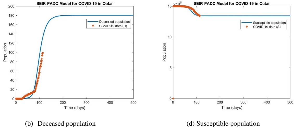
Figure 5: Fitting 4 set of COVID-19 data simultaneously with SEIR-PADC model for dynamics of COVID-19 in Qatar (23 June 2020)
