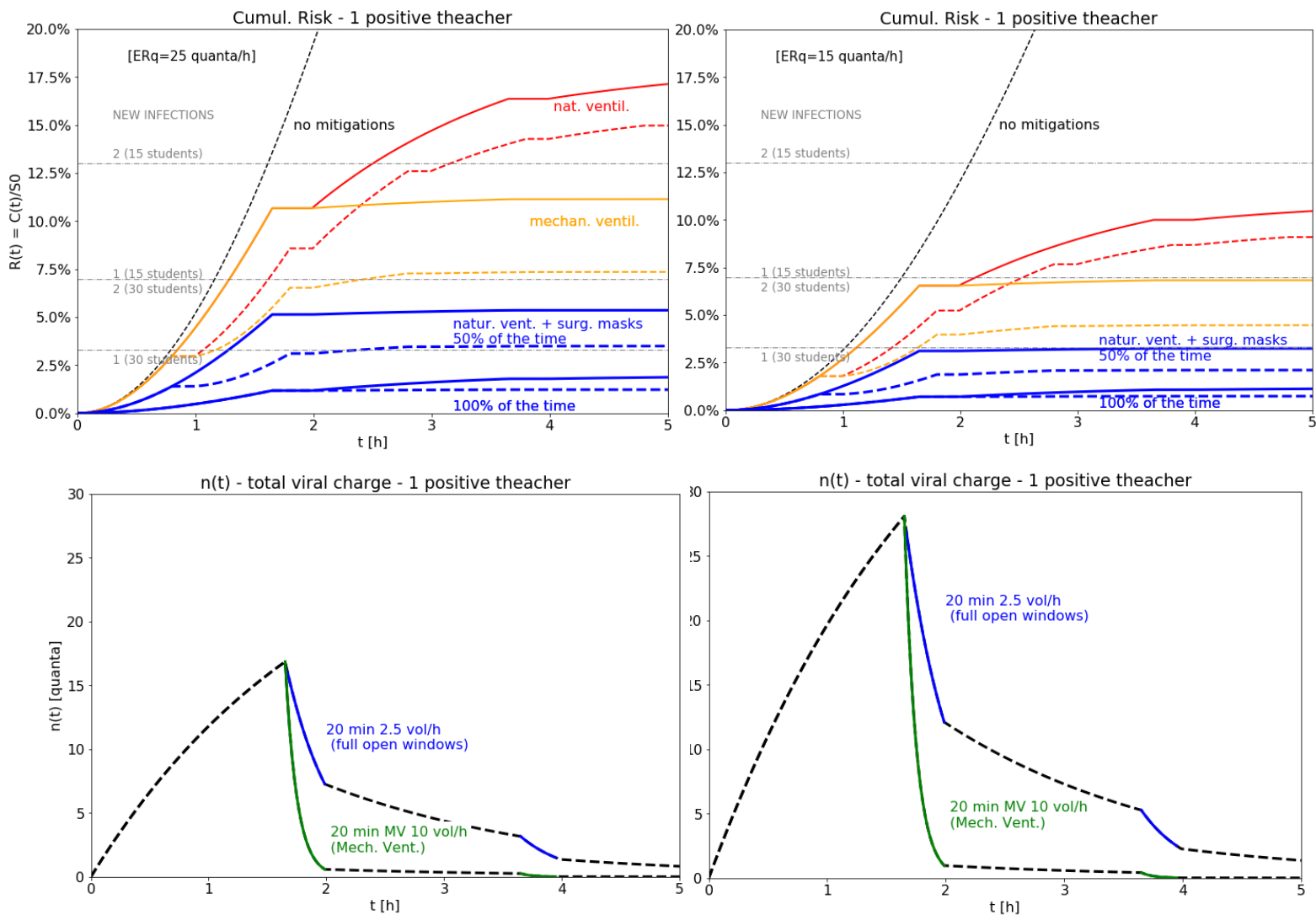
355 Figure 4 Top: cumulative risk curves for the case of an infected teacher in a classroom of volume V = 170 \text{ m}^3 for 2 356 hours as a function of exposure of subjects. Pessimistic (left) vs optimistic (right) scenarios calculated with high ER_q 357 (a) and low ER_q (b), respectively. Natural and mechanical ventilation profiles refer to Fig.2. Bottom: time evolution of 358 viral charge in classroom in natural (open windows) cases and with mechanical ventilation
