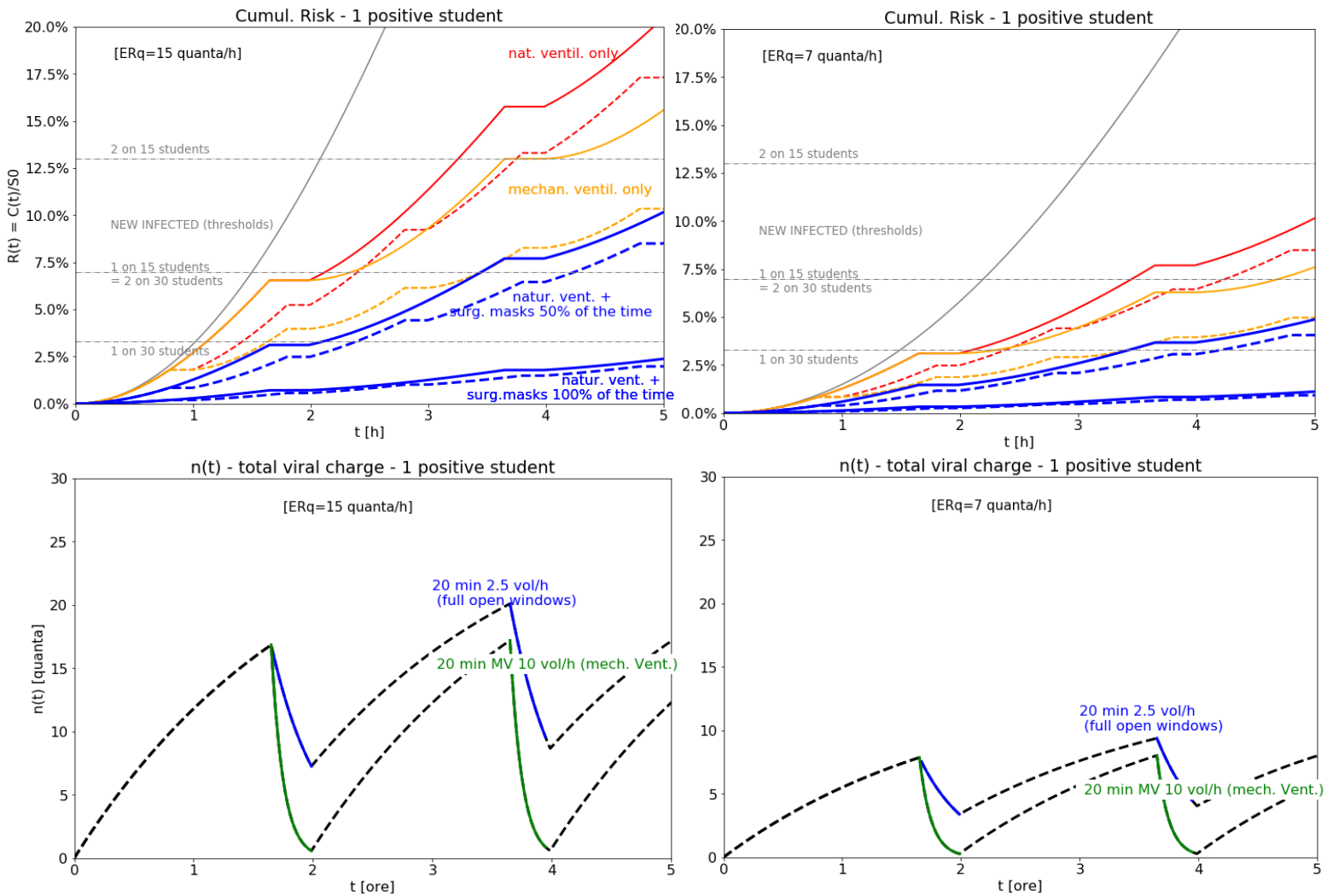
341 Figure 3 Top: cumulative risk curves of indirect airborne transmission as a function of exposure time, considering a 342 standard classroom ( V = 170 \text{ m}^3 ). a) Pessimistic scenario calculated with high ER_q . b) Optimistic scenario with low 343 ER_q . Natural and mechanical ventilation profiles refer to Fig.2. Bottom: time evolution of viral charge in classroom in 344 natural (open windows) cases and with mechanical ventilation.
