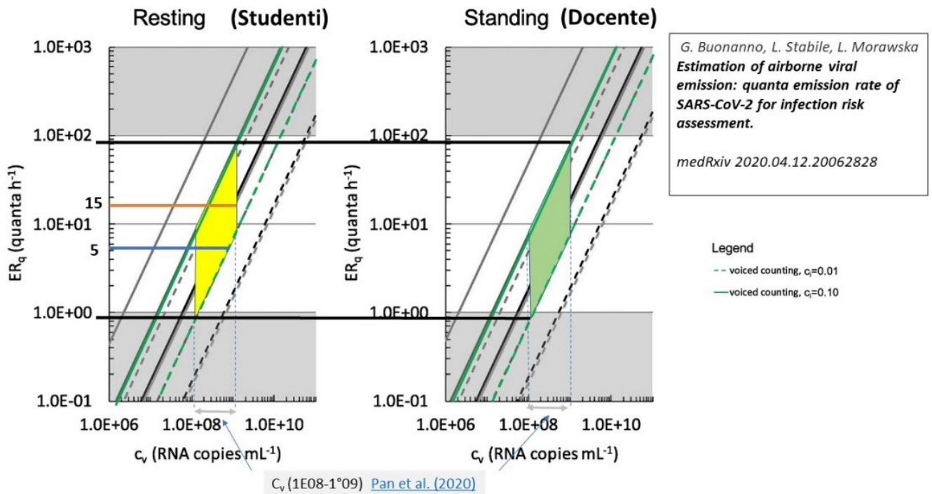
473 Figure A.1. Range of variation for ERq for resting and standing individual as published in [Buonanno 2020]. The 474 values chosen in the present study are highlighted in blue and orange. The yellow and green zones originates by the 475 viral parameters c_i and c_v [Pan et al. 2020].
