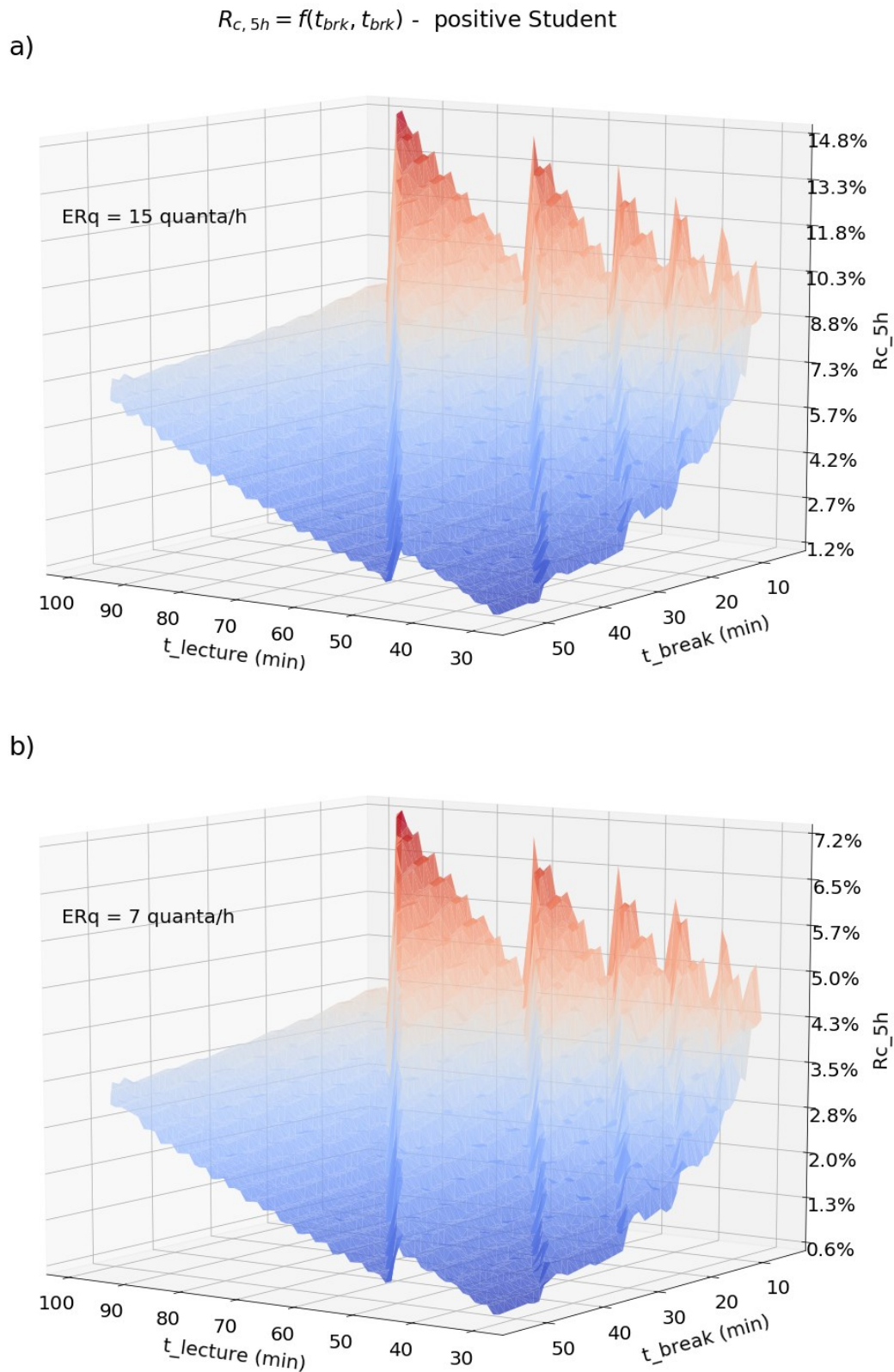
Figure 5 – a,b) Cumulative contagion risk function after 5h exposure R_{c,5h} as a function of lecture and break duration ( t^{lec}, t^{brk} ) for high (a) and low (b) emission rates of the infective source. Hypothesis: one infective student in a classroom of 170 m 3 and face mask effective for 50% of the time ( f_{in}=0.15, f_{out}=0.45 )
